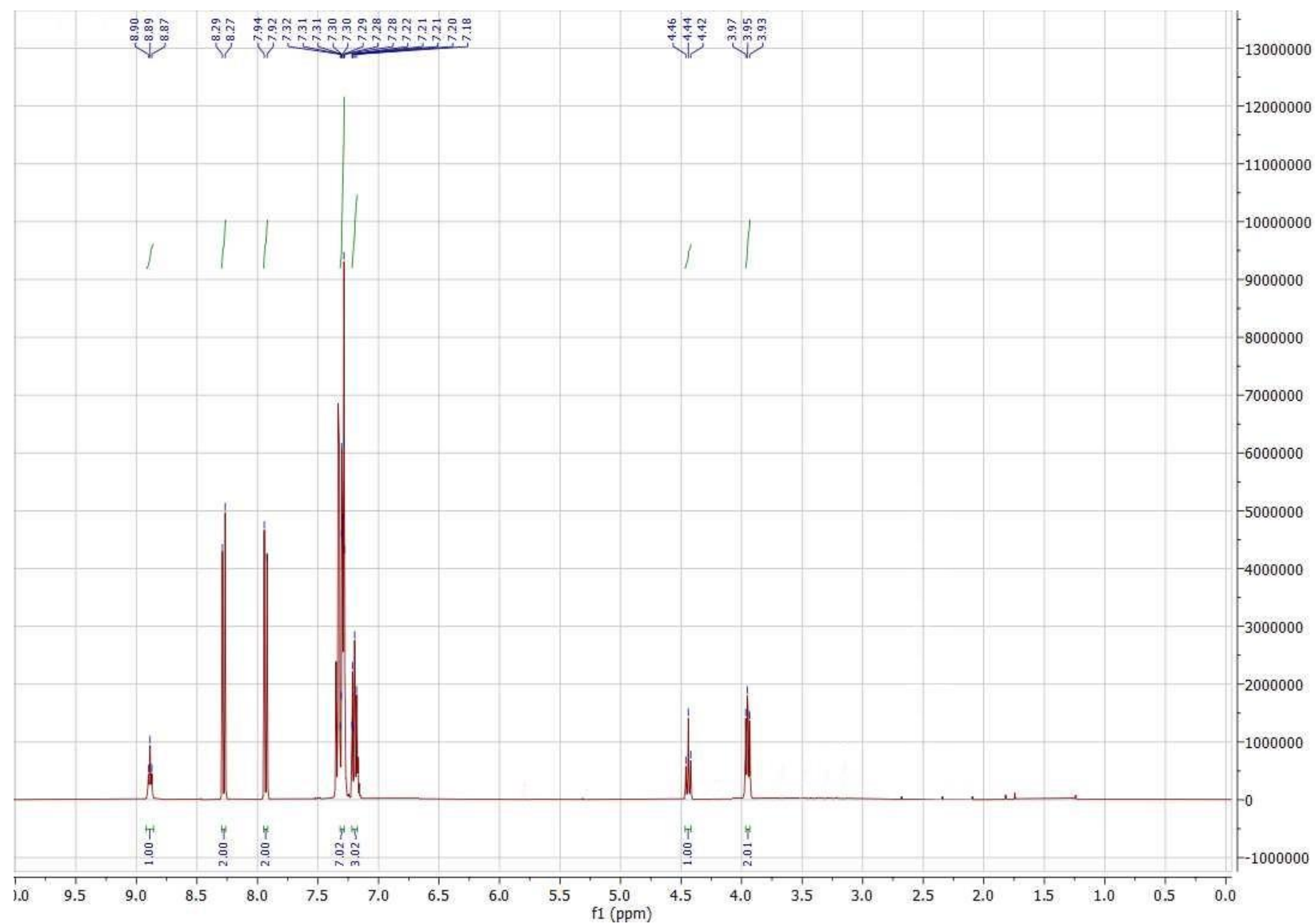
Figure S1. 1 H-NMR spectrum of compound 3.
