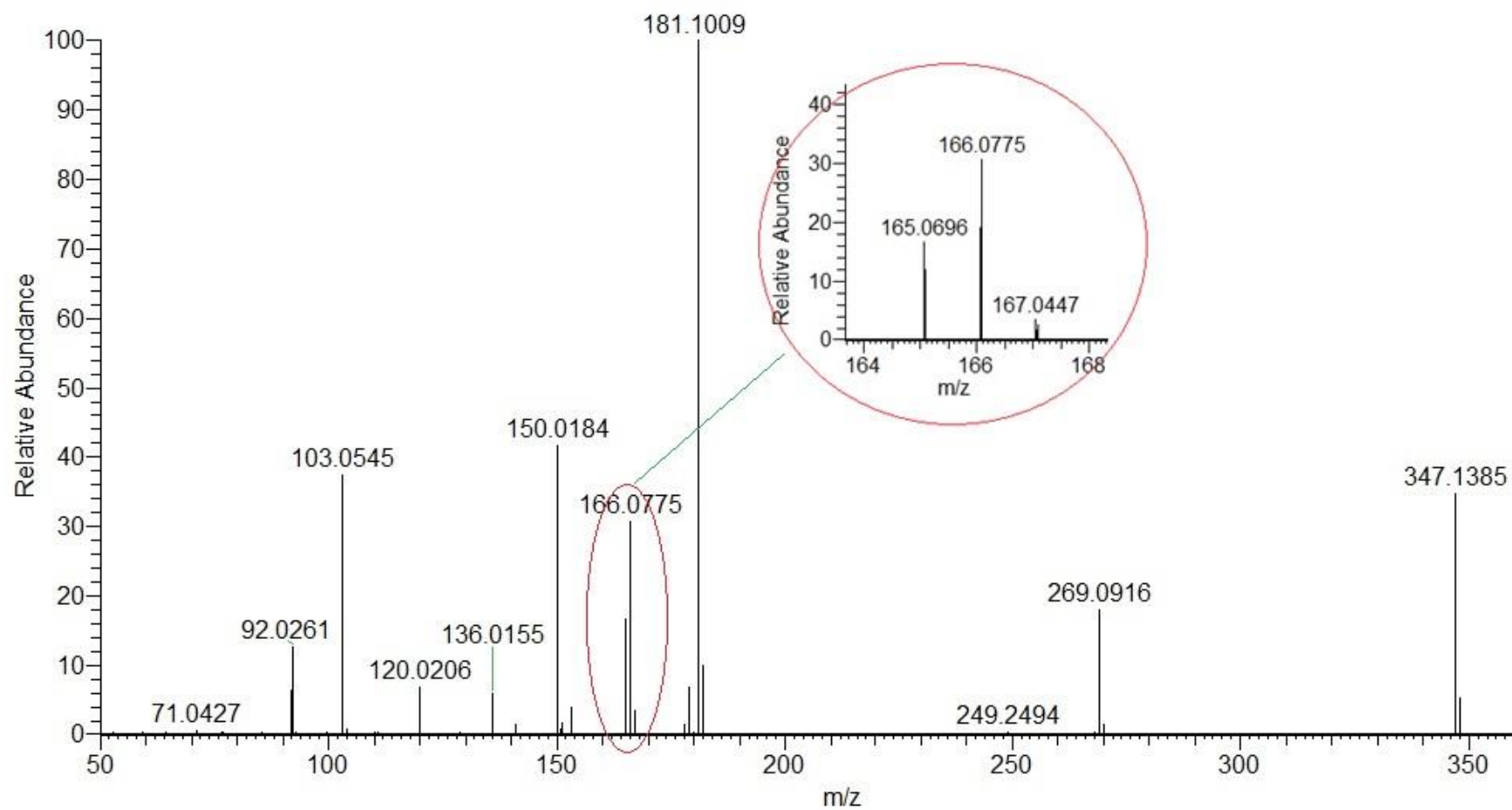
Figure S5. Mass spectrum of compound 3 obtained by positive ion ESI-MS/MS.
