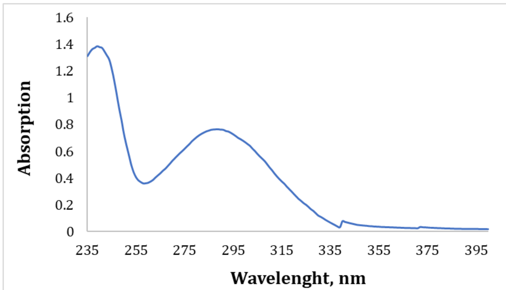
Figure S3. UV spectrum of compound 3.
