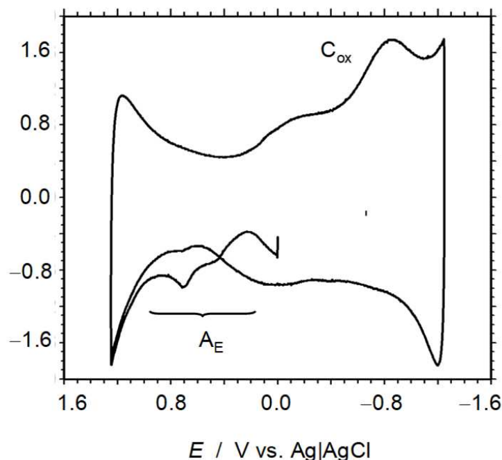
Figure 1. Cyclic voltammogram after semi-derivative convolution of a microparticulate deposit of the ethanolic extract of sample A^{-5} on GCE in contact with air-saturated 0.25 M HAc/NaAc aqueous buffer at pH 4.75. Potentials can initiate at 0.0 V vs. Ag/AgCl in the positive direction; potential scan rate 50 \text{ mV s}^{-1} .
