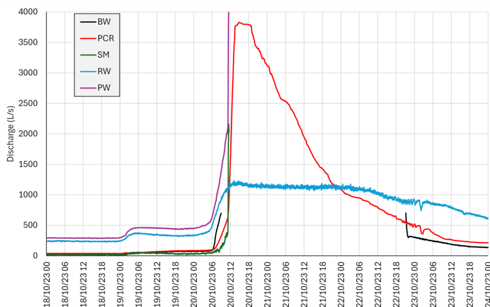
Figure 8. Discharge hydrographs for BW, PCR, SM, RW and PW. Note that the BW hydrograph has been truncated for the period when water was backing up above the weir.
