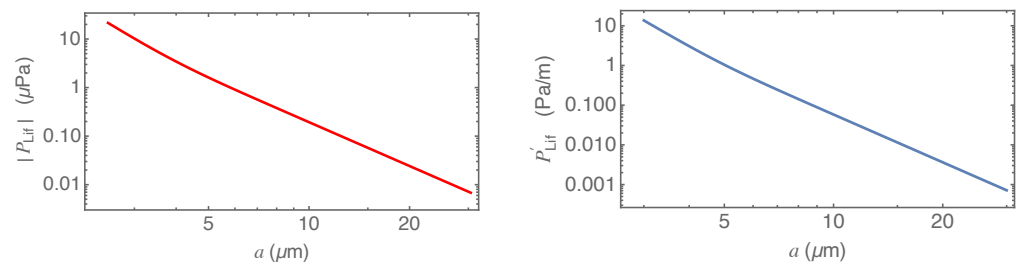
Figure 13. Pressure (left) and its gradient (right) in equilibrium at temperature T = T_{\text{eq}} = 293 \text{ K} for the configuration depicted in Figure 12. The pressure is negative (attraction) while its gradient is positive. The values of both quantities are evaluated using the Lifshitz Formula (11) (see Appendix B) and the material parameters reported in the caption of Figure 12.
