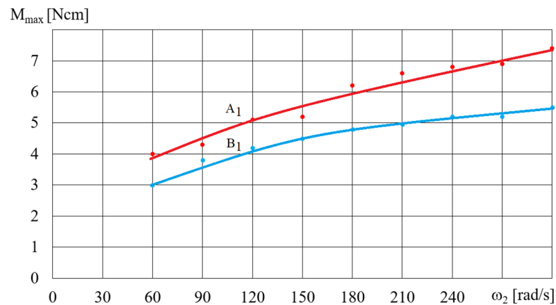
Figure 14. Dependence of the torque M on the angular velocity \omega_2 for fluids A1 and B1 for \omega = 300 rad/s, V = 75 cm 3 .
