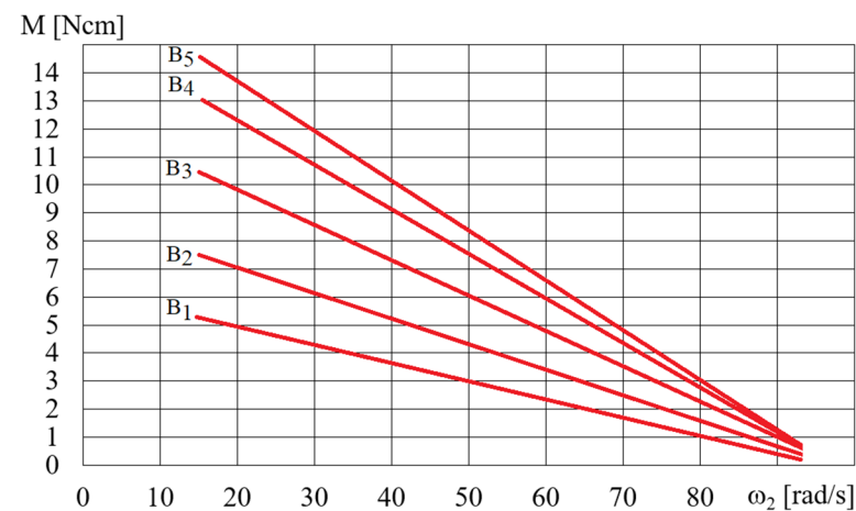
Figure 13. Dependence of the torque M on the angular velocity \omega_2 for fluids B1–B5 for \omega = 300 \text{ rad/s} , V = 75 \text{ cm}^3 .
