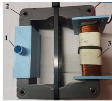
Figure 3. Magnetic device used to test the MR fluid: 1—beaker with MR fluid, 2—electromagnet coil, 3—magnetic circuit.
