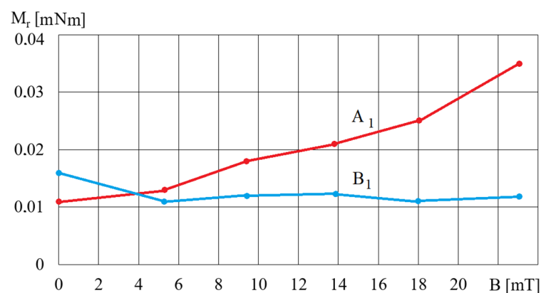
Figure 4. The dependence of the torque, M_r , on magnetic induction B for fluids A1 and B1 and for \omega_r = 2 rad/s.
