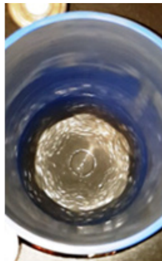
Figure 8. View of a hexagon formed by the rotation of the MR fluid for B3 fluid and \omega = 240 rad/s.
