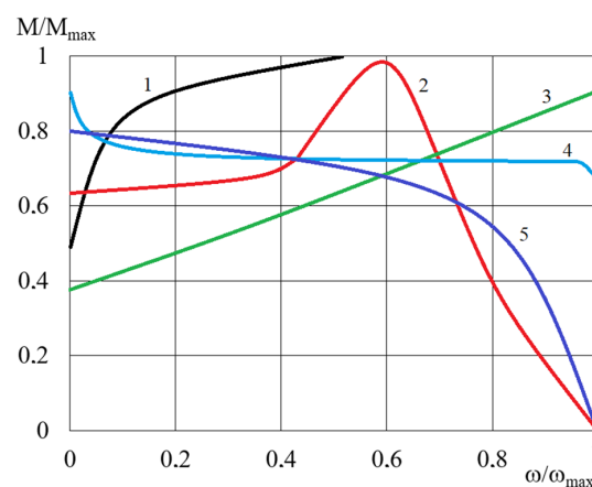
Figure 19. Characteristics of clutches using the influence of a magnetic field: 1—electromagnetic friction-type clutches [8], 2—induction clutches [45], 3—viscous clutches with MR fluid [47], 4—magnetic particle clutches [8], 5—eddy current clutches [8].
