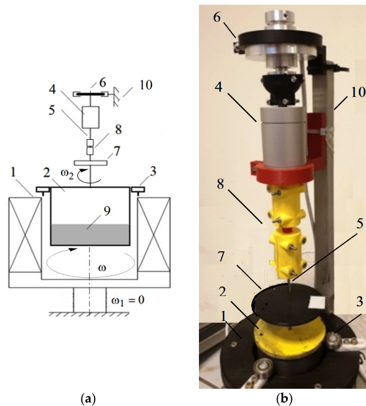
Figure 6. HCMR test stand: (a) construction scheme: 1—stator of a three-phase induction motor, 2—beaker, 3—beaker bearing, 4—torque meter, 5—output shaft, 6—brake, 7—rotational speed meter, 8—clutch, 9—MR fluid, 10—frame; (b) view.
