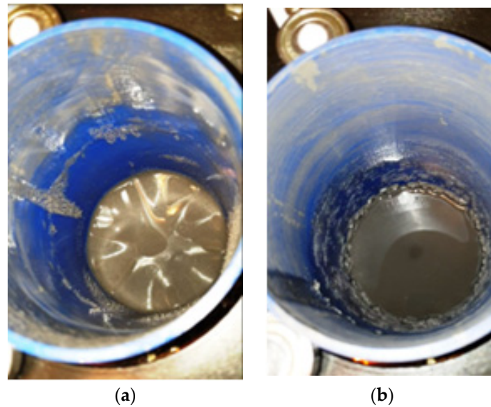
Figure 7. View of the B3 fluid surface at HCMR start-up for \omega = 240 rad/s: (a) wrinkles, (b) ring of swirling fluid.
