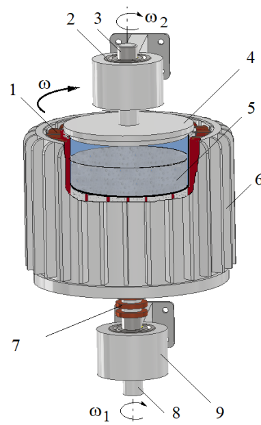
Figure 1. HCMR construction scheme: 1—coil, 2—bearings, 3—output shaft, 4—beaker, 5—MR fluid, 6—stator of a three-phase induction motor, 7—slip rings, 8—input shaft, 9—bearing housing.
