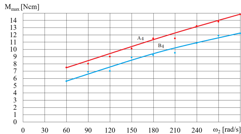
Figure 15. Dependence of the torque M_{max} on angular velocity \omega for fluids A4 and B4, V = 75 cm 3 .
