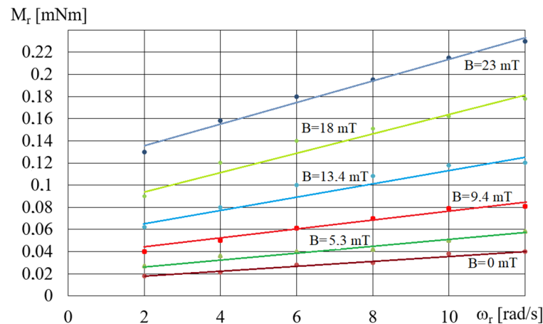
Figure 5. Dependences of the torque M_r on \omega_r for fluid A5 and different values of B .
