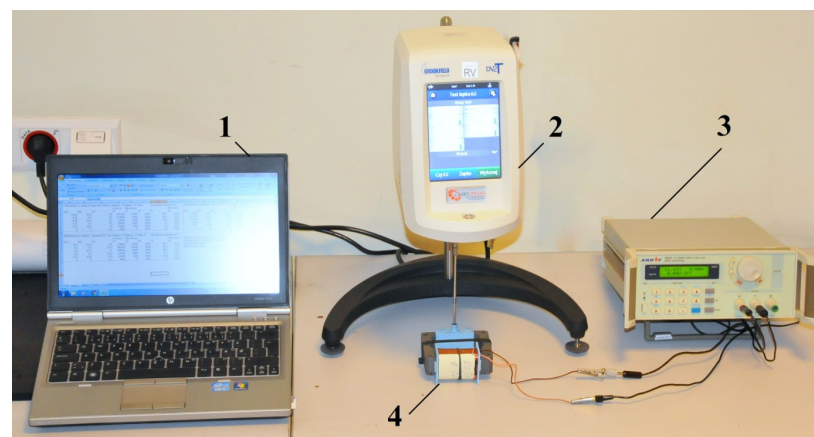
Figure 2. View of the station used for testing the rheological properties of the MR fluid: 1—PC, 2—rheometer, 3—electric power supply, 4—magnetic device.
