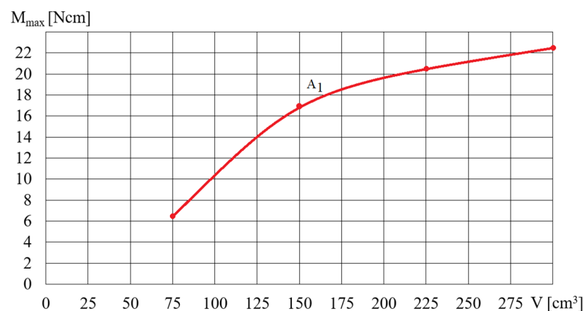
Figure 16. Dependence of the torque M_{max} on the volume V of the fluid A1 for \omega = 200 rad/s.
