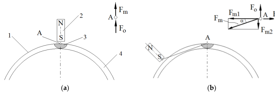
Figure 18. Forces acting on the MR fluid and the beaker during HCMR operation: (a) \omega_2 = \omega ; 1—beaker wall, 2—magnet, 3—MR fluid pulled by the magnet, 4—a ring of MR fluid; (b) \omega_2 < \omega .
