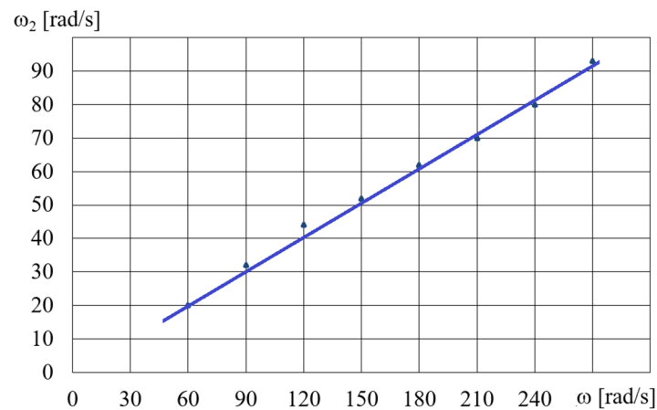
Figure 11. Dependences of angular velocity \omega_2 on angular velocity \omega for the fluid B5 and fluid volume V = 75 \text{ cm}^3 .
