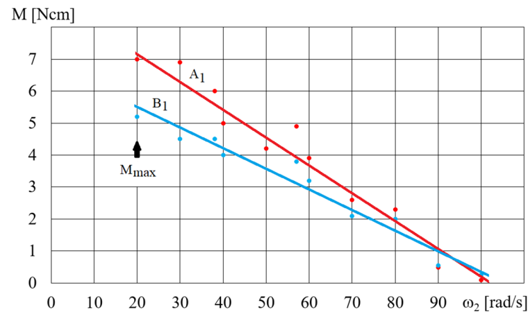
Figure 12. Dependence of the torque M on the angular velocity \omega_2 for fluids A1 and B1, \omega = 300 \text{ rad/s} , V = 75 \text{ cm}^3 .
