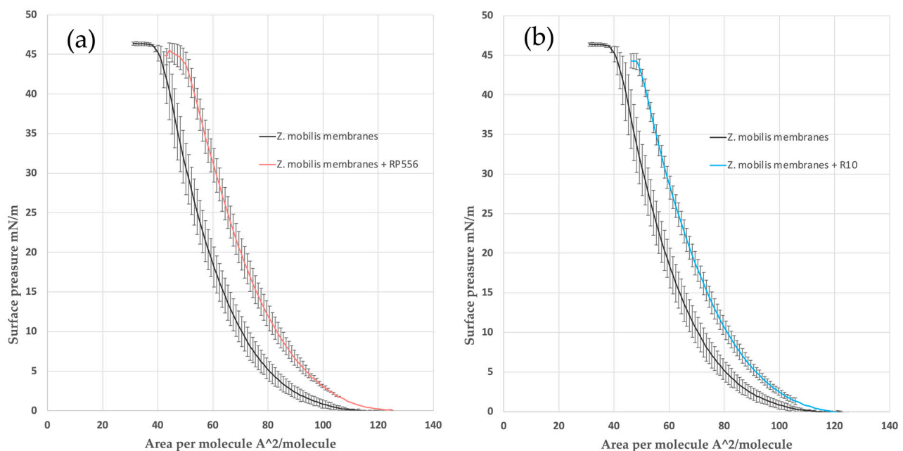
Figure 2. The \pi -A isotherms for Z. mobilis model mixtures with peptides R2 (a) and R10 (b). Dashed lines denote the linear part of the \pi -A isotherms, taken for the calculation of the limiting area per molecule ( A_{\pi \rightarrow 0} ).
