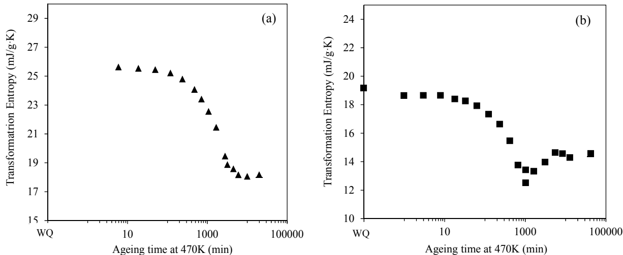
Figure 6. Evolution of the transformation entropy (average absolute values, \Delta S ) as a function of post-quench aging time at 470 K for alloys C2 (a) and C4 (b) (adapted from [15]).
