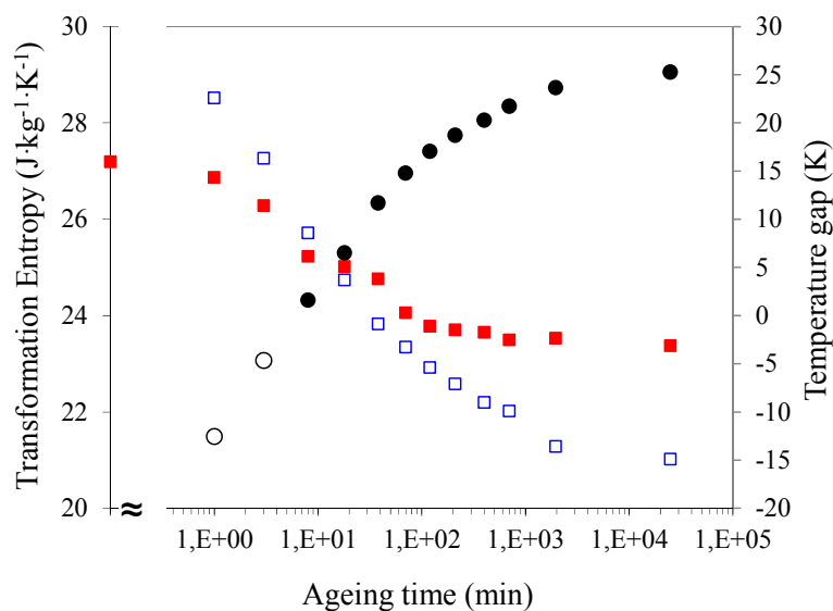
Figure 4. Transformation entropy changes (absolute values) measured for the forward ( \square |\Delta S^{A \rightarrow m}| ) and reverse ( \blacksquare |\Delta S^{m \rightarrow A}| ) MTs, and temperature gap ( T_C^A - T_o ) ( \bullet , right axis; open circles are used for extrapolated Curie temperatures), of alloy C1 as a function of ageing time at 570 K after WQ from 1070 K.
