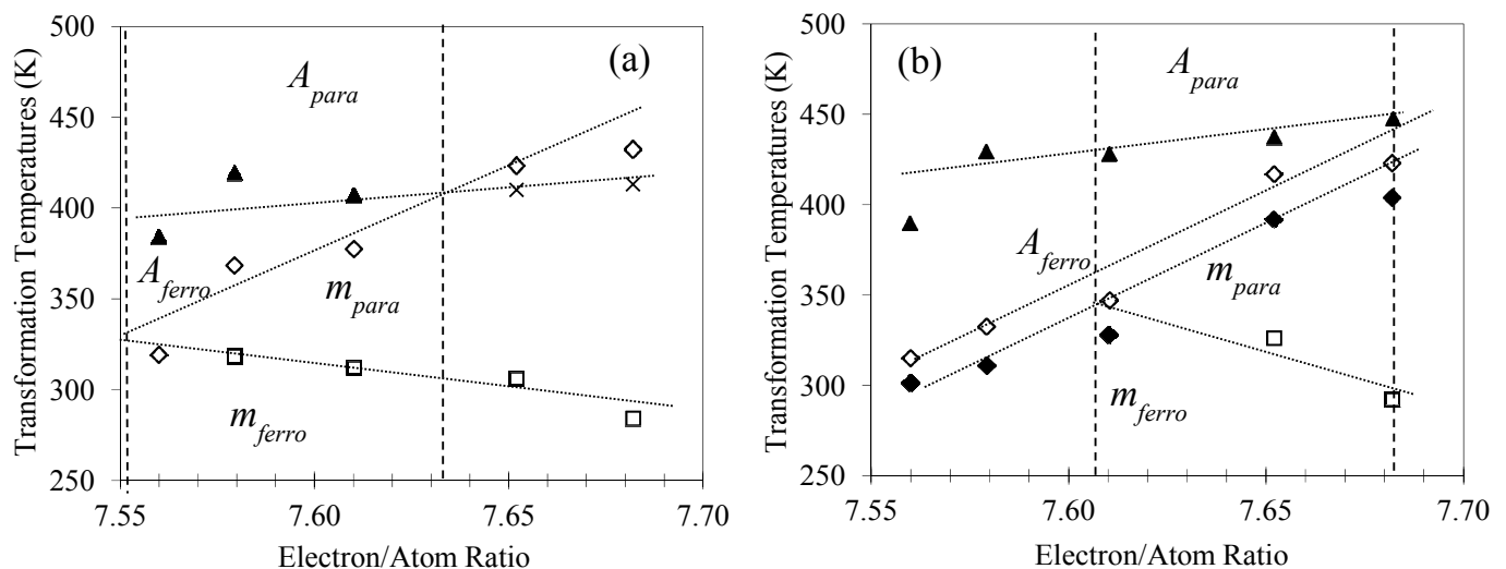
Figure 2. Dependence of the structural and magnetic transformation temperatures ( \blacktriangle T_C^A , \diamond A_p , \blacklozenge M_p and \square T_C^m ) on the electron to atom ratio, (a) after water quench from 1070 K and (b) after 100 min aging at 520 K. Crosses are used for extrapolated T_C^A values (adapted from [15]).
