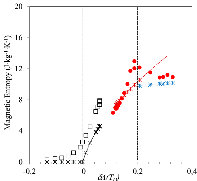
Figure 7. Experimental (absolute values: \square alloy C2, \bullet alloy C4) and calculated magnetic entropy (dashed lines and \ast , \times for A_{ferro} \leftrightarrow m_{para} , \ast for A_{ferro} \leftrightarrow m_{ferro} MTs) as a function of the reduced temperature difference at the transformation temperature \delta_A(T_O) . The structural contribution has been chosen as \Delta S_{strc} = 26 \text{ J} \cdot \text{kg}^{-1} \cdot \text{K}^{-1} .
