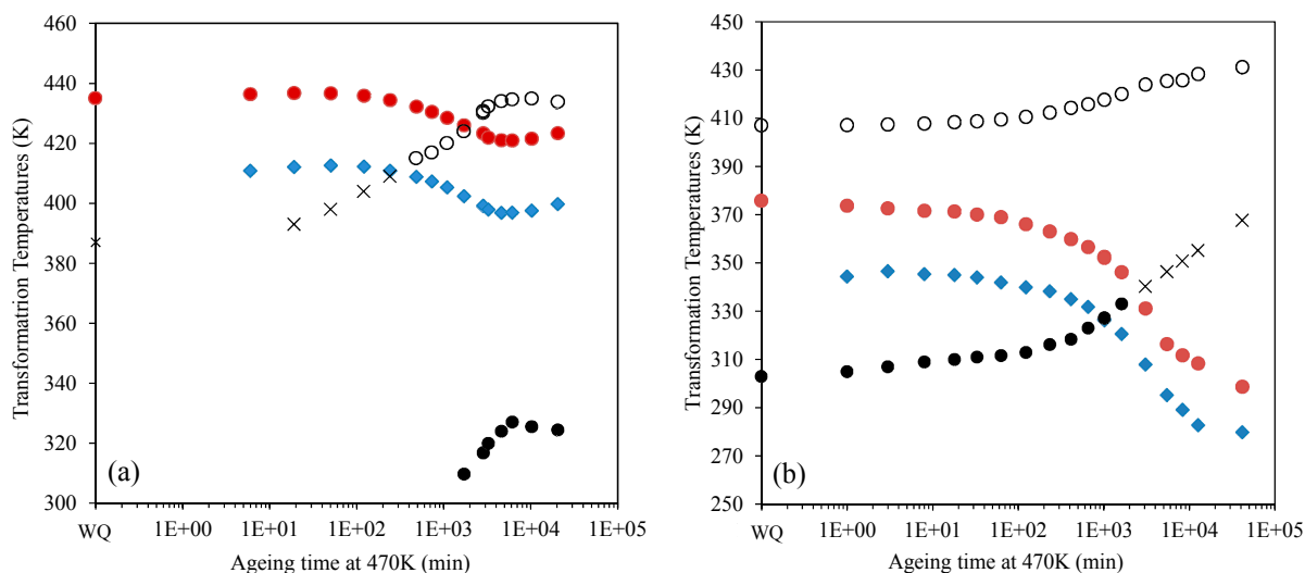
Figure 3. Evolution of the transformation temperatures ( \circ T_C^A , \bullet A_p , \blacklozenge M_p and \bullet T_C^m ) with ageing time at 470 K (after water quench from 970 K) for alloys C2 (a) and C4 (b). For T_C^A < M_p (alloy C2) and T_C^m > A_p (alloy C4) Curie temperatures are extrapolated and indicated as \times (adapted from [15]).
