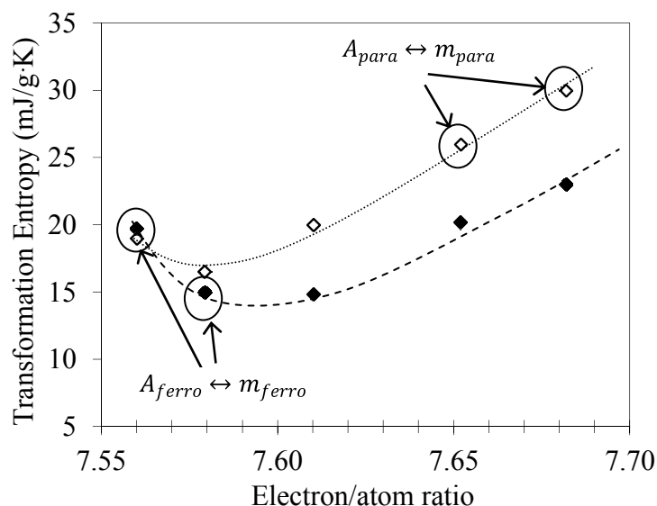
Figure 5. Average absolute values of the transformation entropy changes as a function of the electron to atom ratio ( e/a ), after water quench from 1070 K ( \diamond ), and after 100 min aging at 520 K ( \blacklozenge ). Unless otherwise specified, MT is A_{ferro} \leftrightarrow m_{para} .
