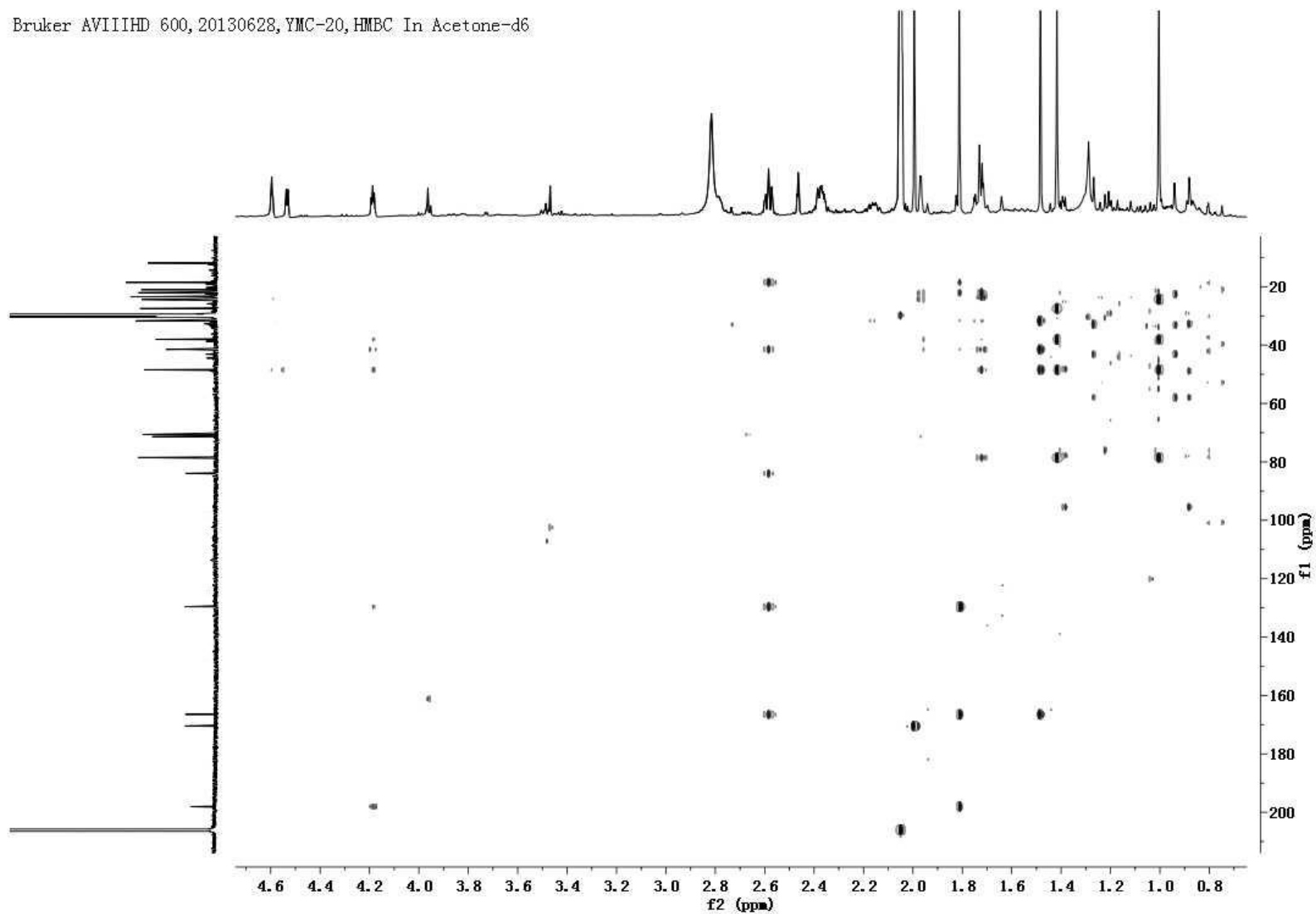
Figure S8. The HMBC Spectrum of Compound 1 in Me 2 CO- d 6 .
