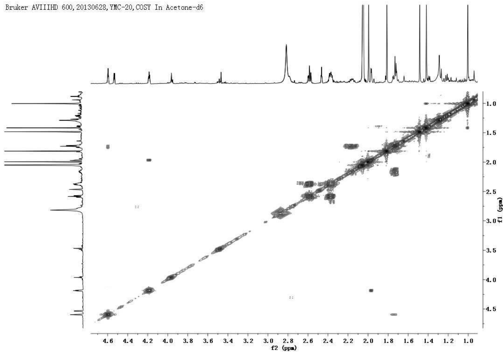
Figure S7. The ^1\text{H} – ^1\text{H} gCOSY Spectrum of Compound 1 in \text{Me}_2\text{CO}-d_6 .
