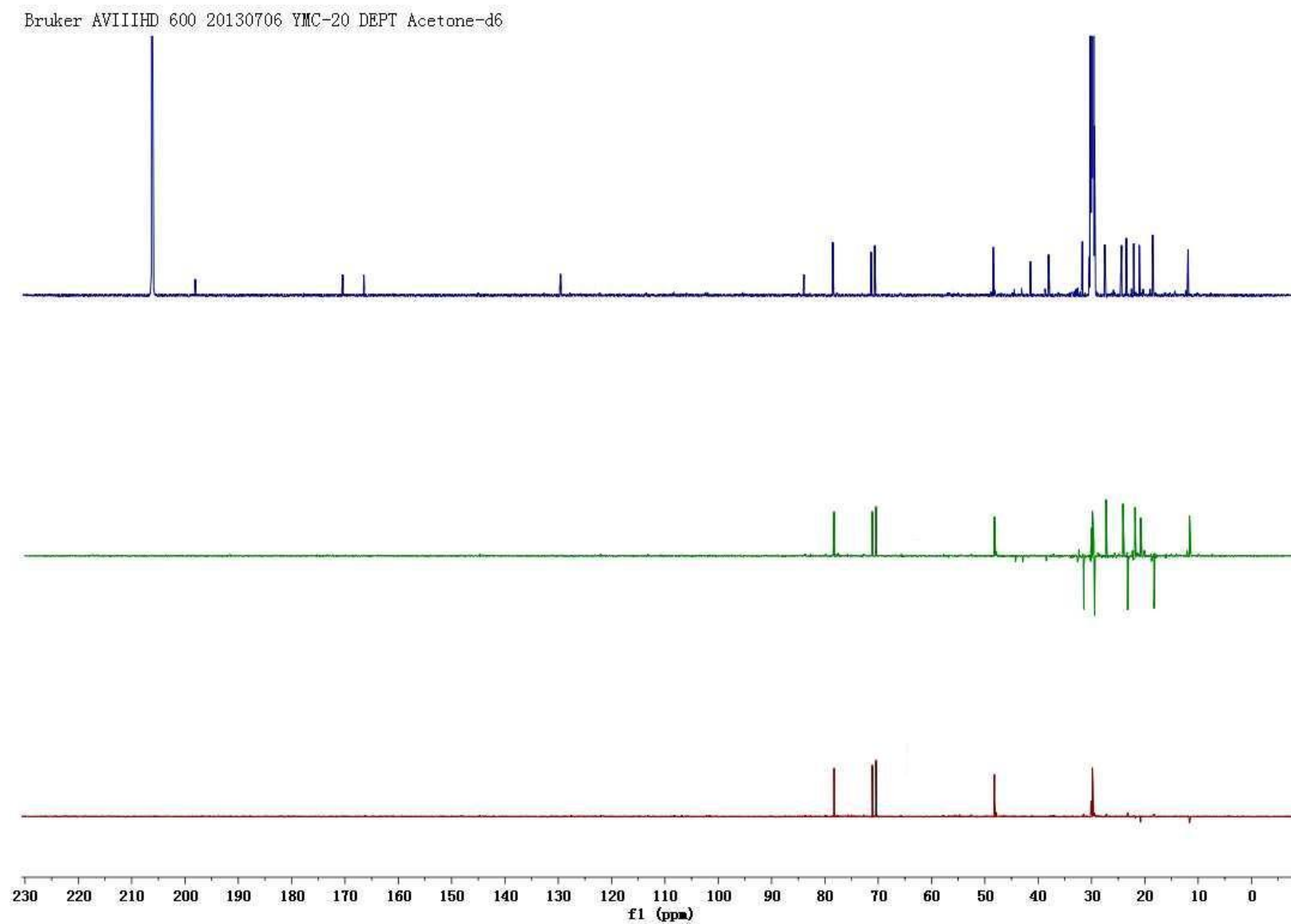
Figure S5. The DEPT Spectrum of Compound 1 in Me 2 CO- d 6 .
