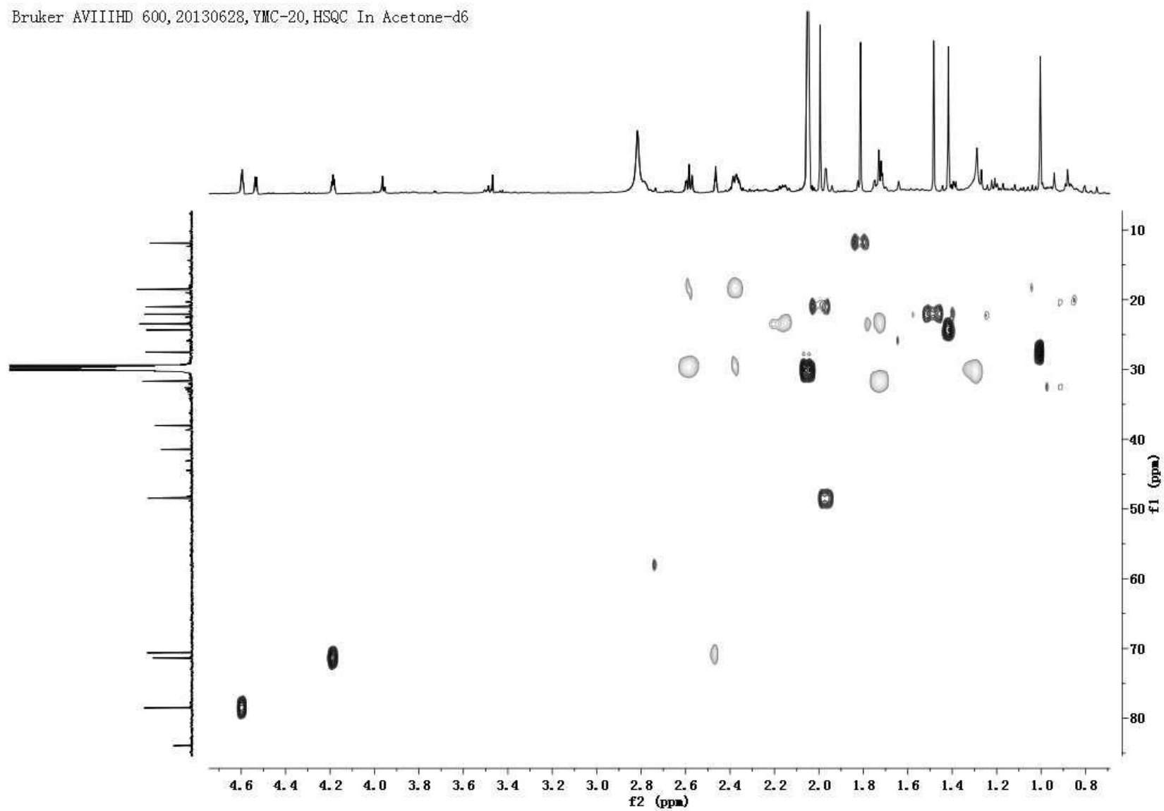
Figure S6. The HSQC Spectrum of Compound 1 in Me 2 CO- d 6 .
