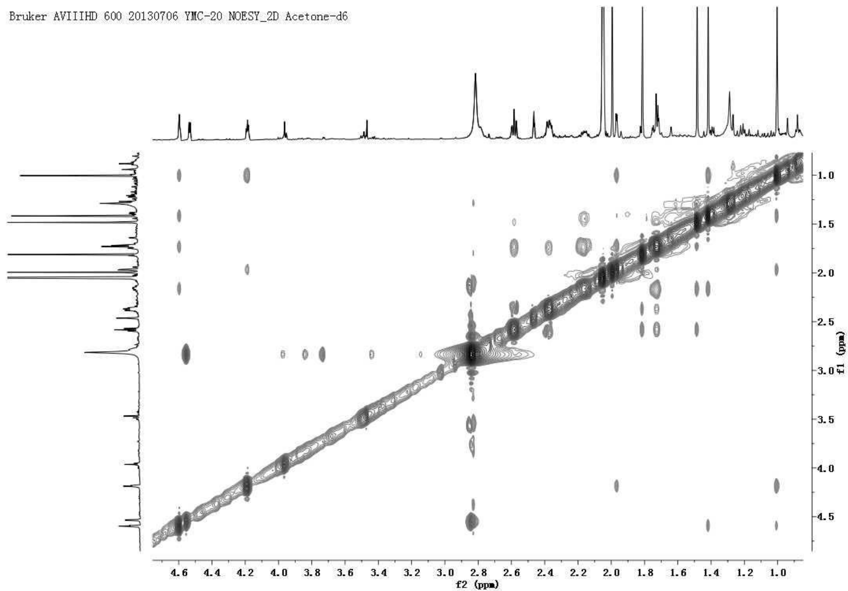
Figure S9. The NOESY Spectrum of Compound 1 in Me 2 CO- d 6 .
