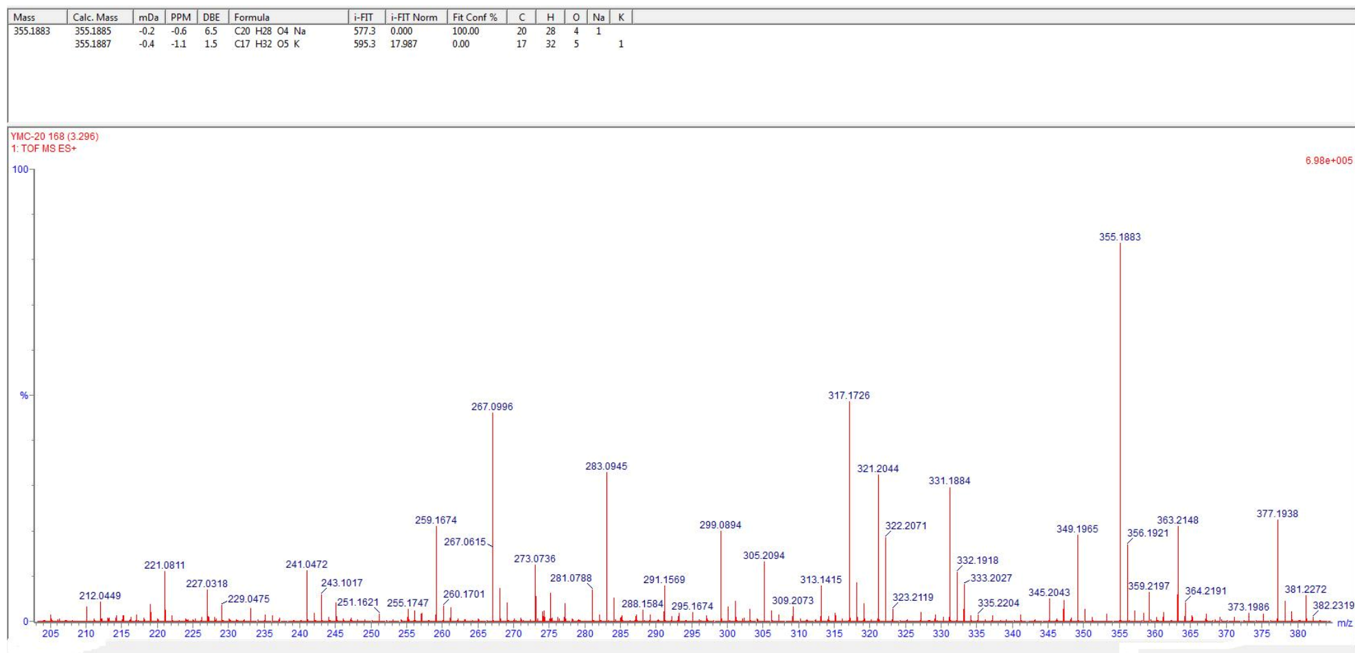
Figure S2. The (+)-HRESIMS Spectroscopic Data of Compound 1.
