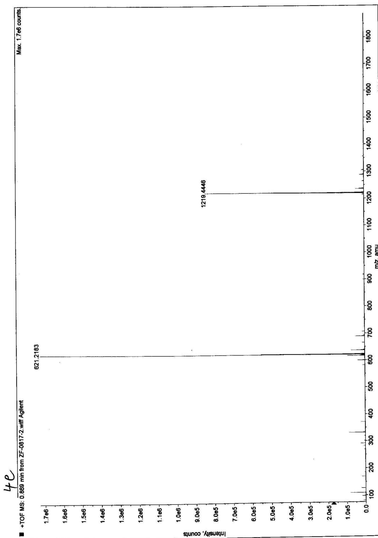
Figure 28. HRMS of compound 4e.
