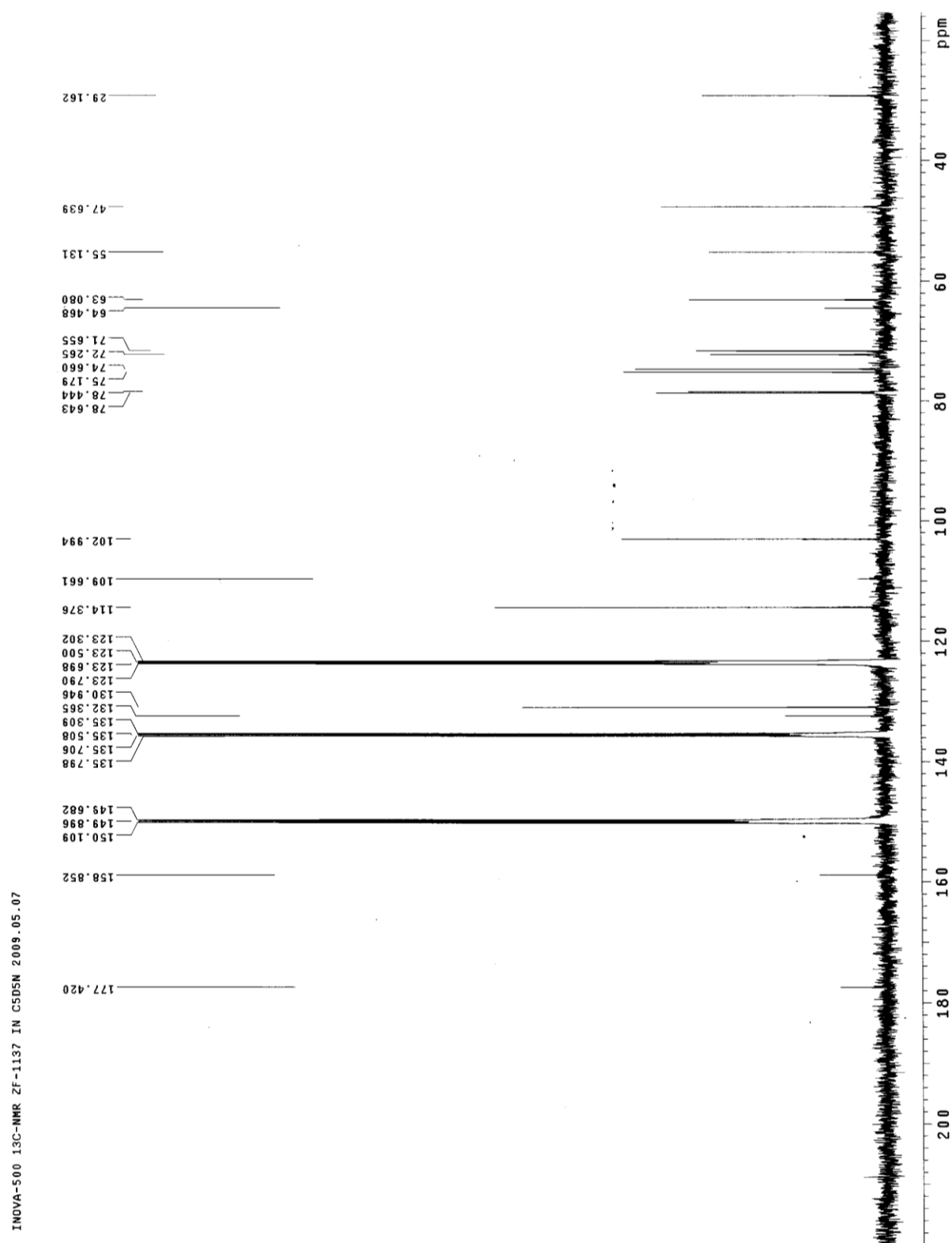
Figure 68. ^{13}\text{C} -NMR of compound 7e.
