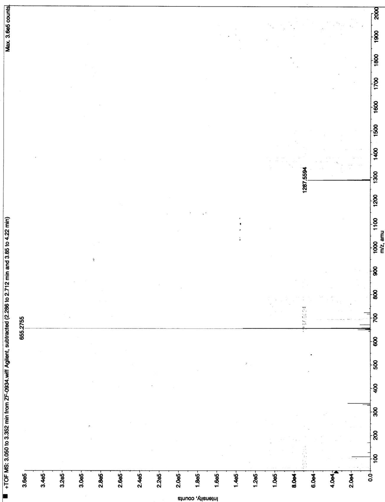
Figure 14. HRMS of compound 3c.
