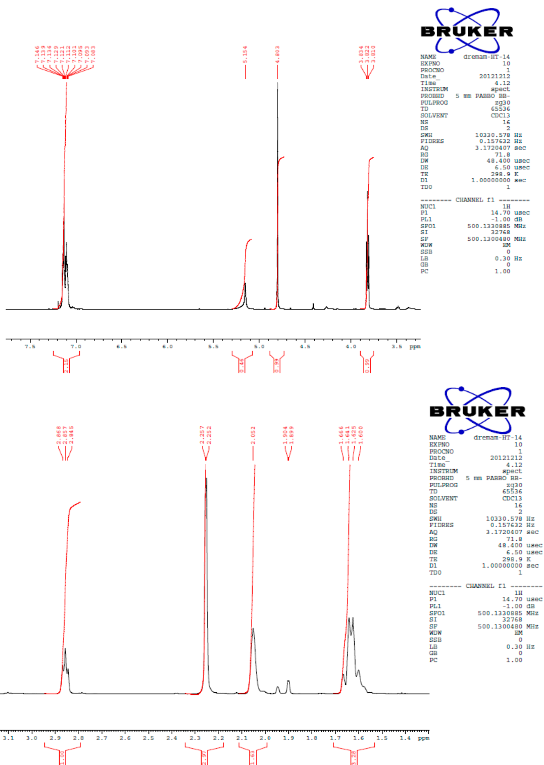
Figure S5. ^1\text{H} -NMR Spectrum of Compound 9 .
