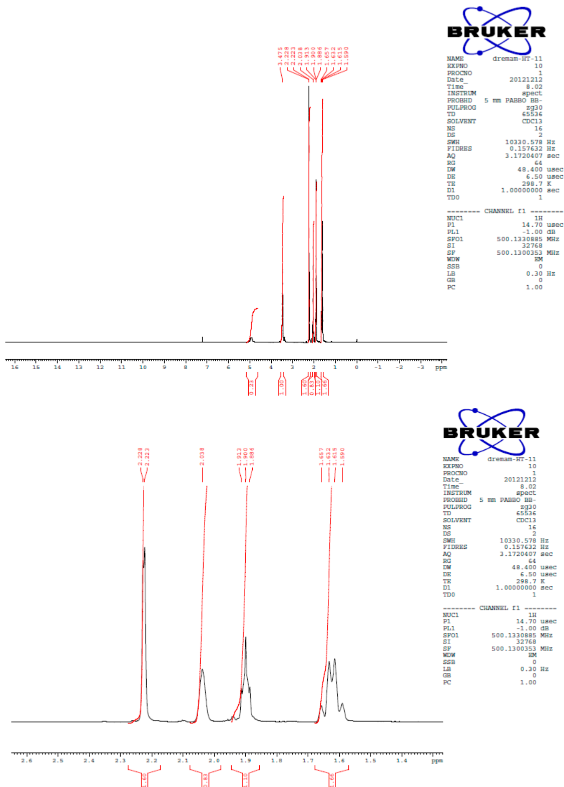
Figure S3. ^1\text{H} -NMR Spectrum of Compound 7.
