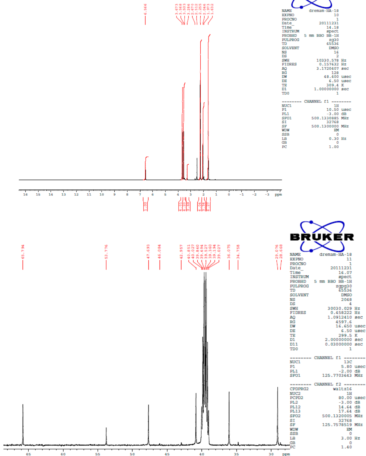
Figure S1. 1 H-NMR Spectrum of Compound 6.
