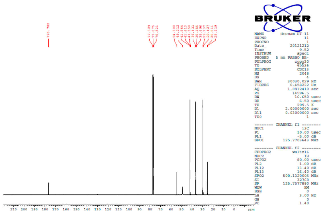
Figure S4. ^{13}\text{C} -NMR Spectrum of Compound 7.
