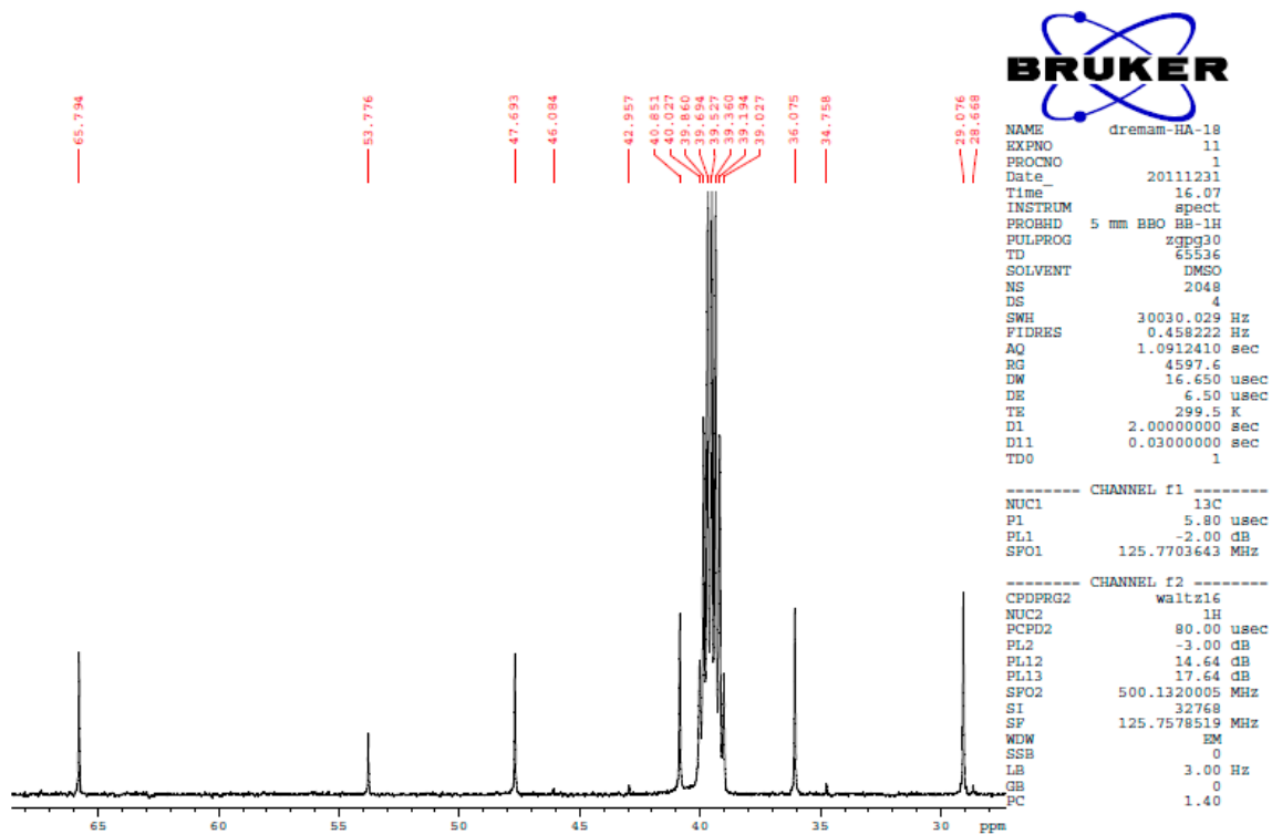
Figure S2. ^{13}\text{C} -NMR Spectrum of Compound 6.
