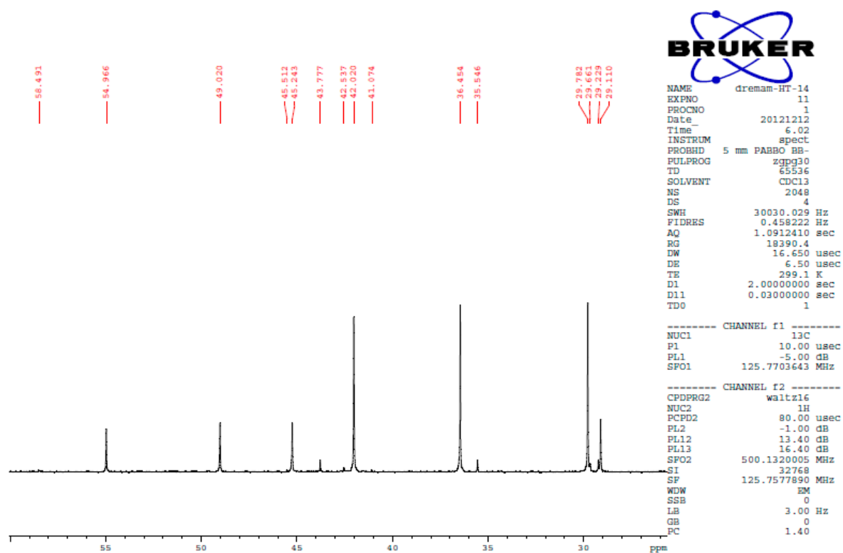
Figure S6. ^{13}\text{C} -NMR Spectrum of Compound 9 .
