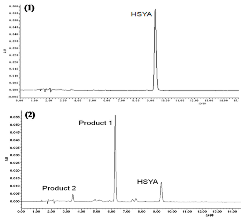
Figure S2. HPLC chromatogram of HSYA standard (time = 0) (1) and HSYA in buffer solution of pH 9.16 after 7 h (2)
