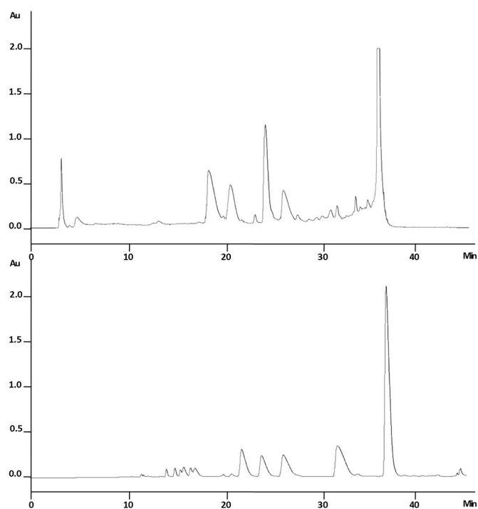
Figure S1. Semi-preparative HPLC profile of \epsilon -viniferin and its metabolites (four glucuronides, upper panel and four sulfates, lower panel), produced by hemi-synthesis.
