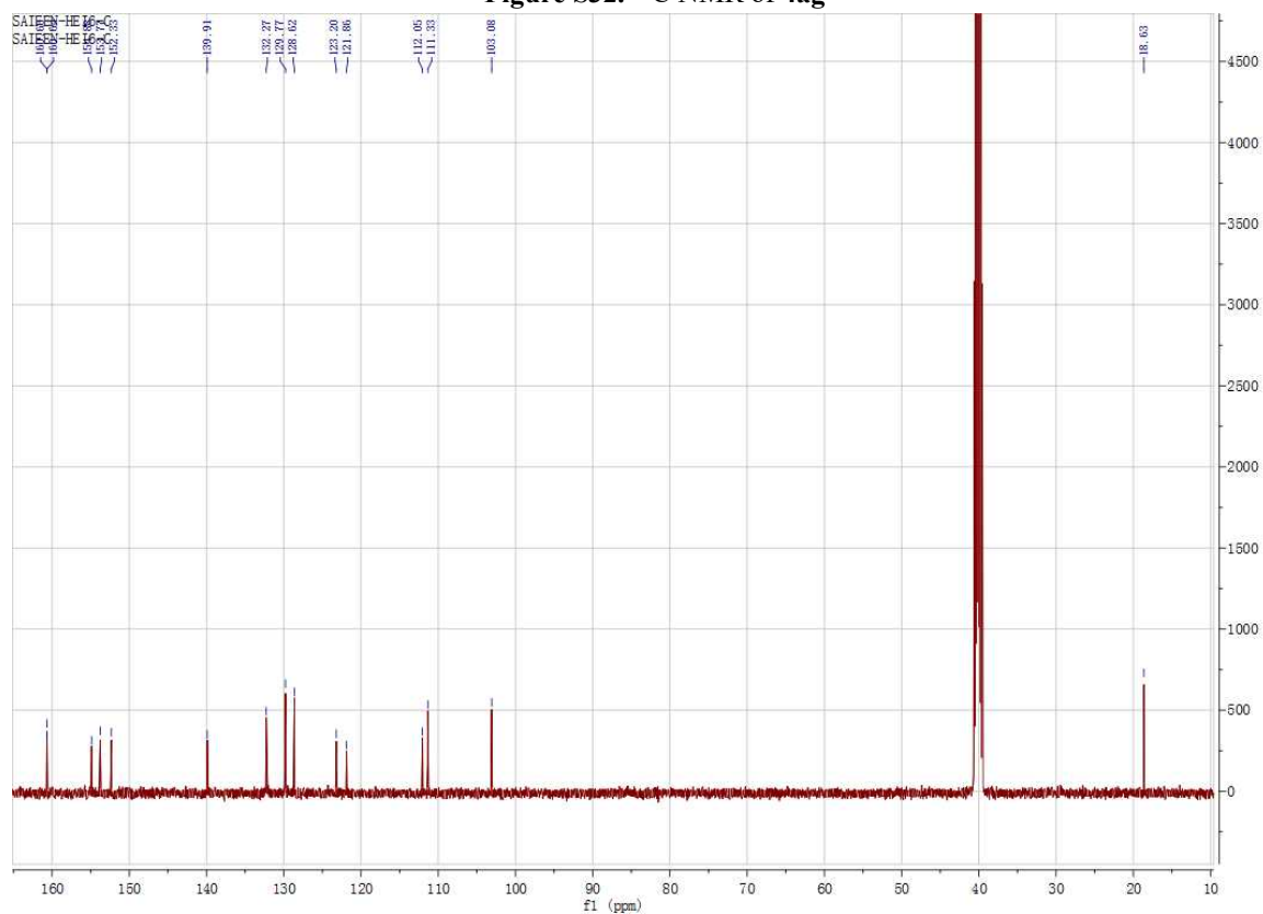
Figure S33. ^{13}\text{C} NMR of 4ah
