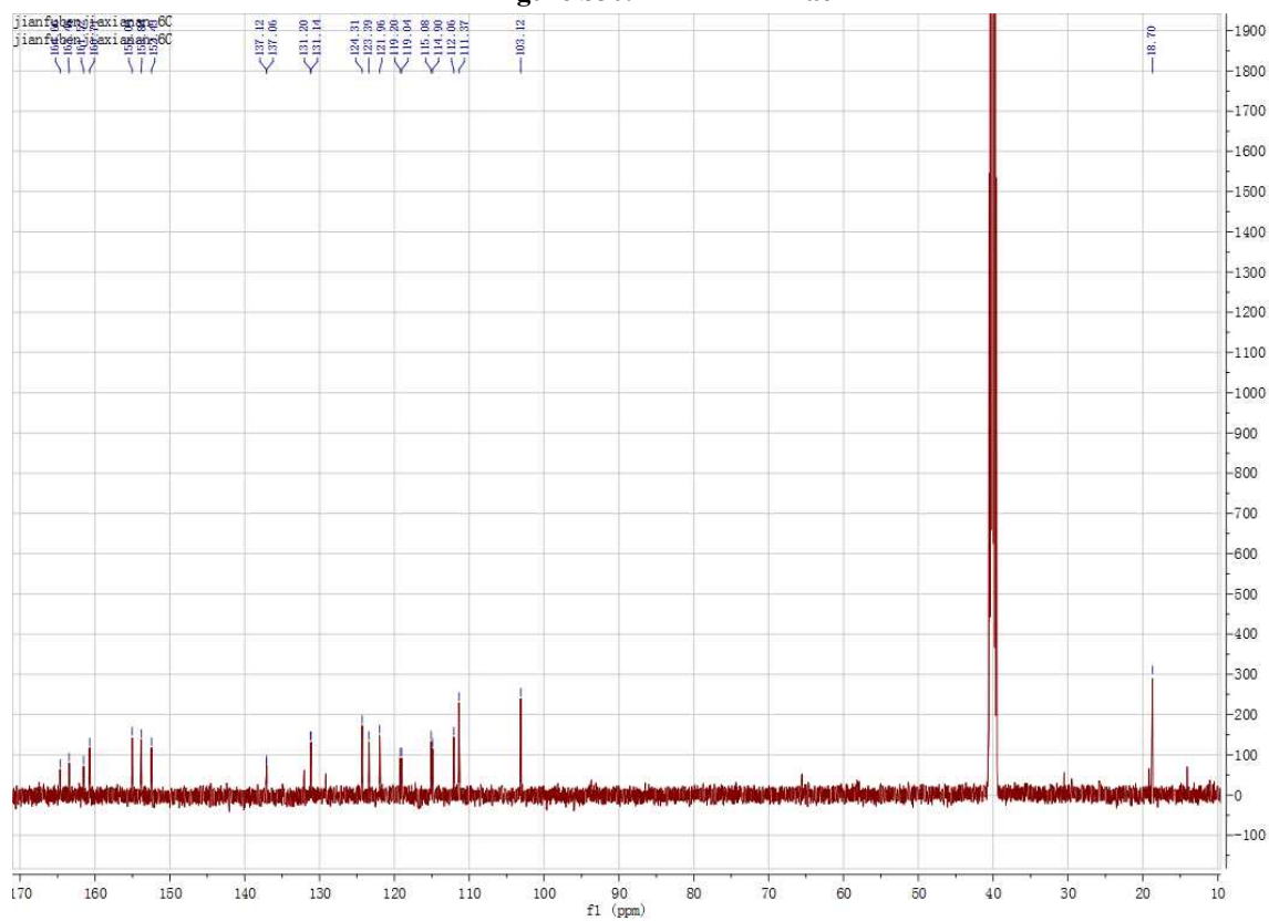
Figure S31. ^{13}\text{C} NMR of 4af
