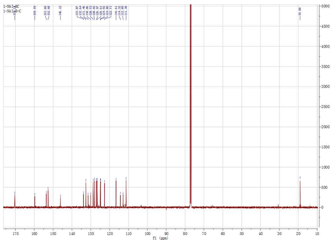
Figure S50. ^{13}\text{C} NMR of 4bq
