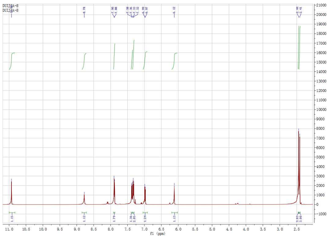
Figure S19. ^1\text{H} NMR of 4bk
