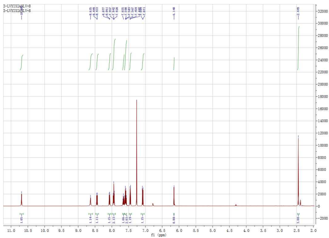
Figure S25. ^1\text{H} NMR of 4bq
