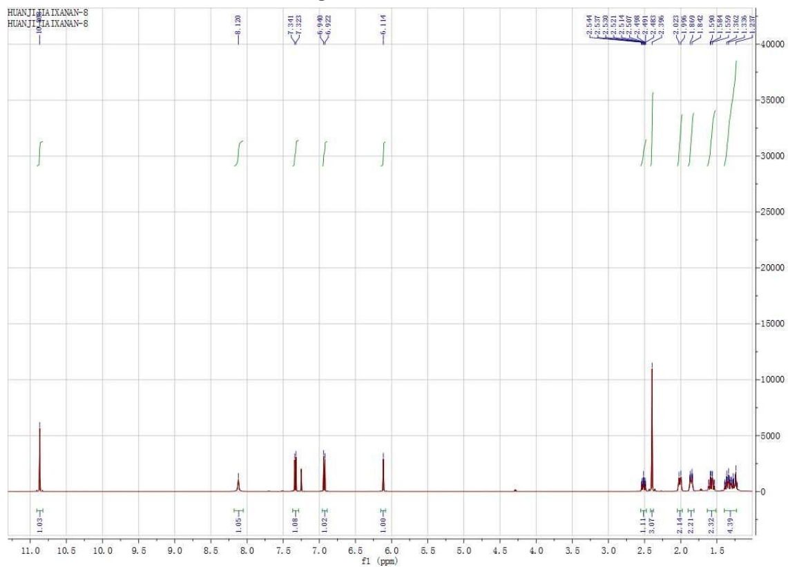
Figure S14. ^1\text{H} NMR of 4bf
