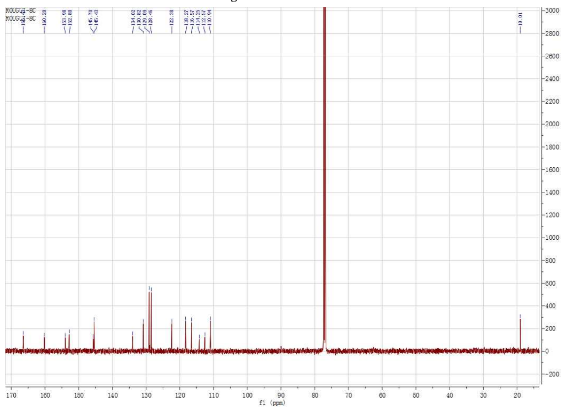
Figure S43. ^{13}\text{C} NMR of 4bj
