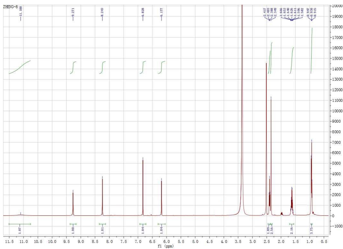
Figure S1. ^1\text{H} NMR of 4aa
