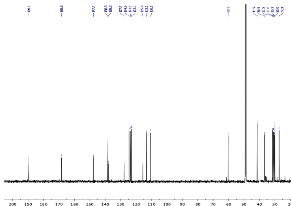
Figure S3. ^{13}\text{C} -NMR (150 MHz, \text{CD}_3\text{OD} ) spectra of 8-oxo-9-dihydromakomakine
