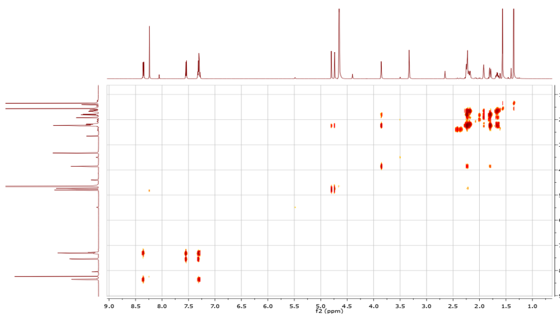
Figure S4. gs-H,H-COSY spectra of 8-oxo-9-dihydromakomakine in \text{CD}_3\text{OD}
