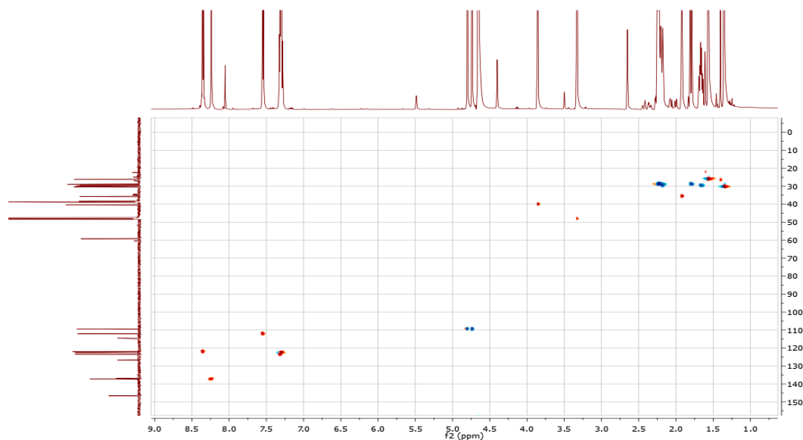
Figure S5. edited HSQC spectra of 8-oxo-9-dihydromakomakine in CD 3 OD
