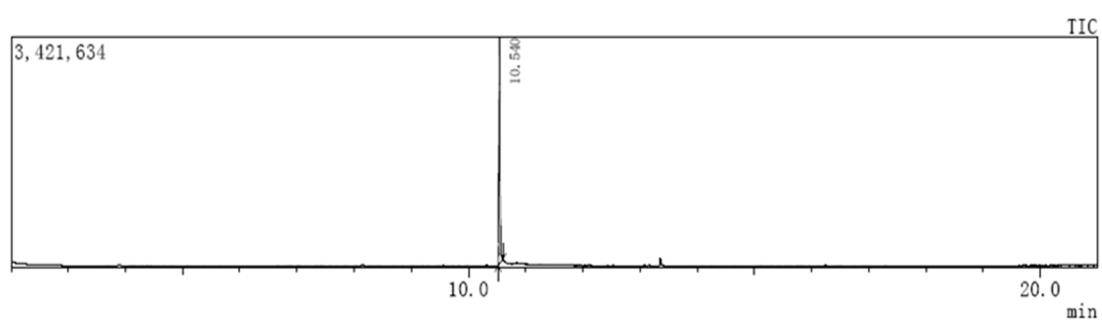
Figure S1. GC spectra of the product of the conversion of FA into EL.
