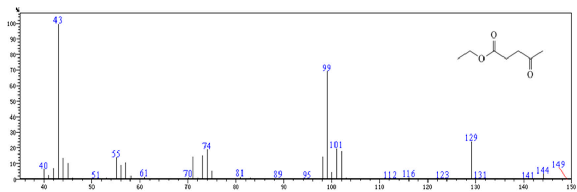
Figure S2. MS spectra of the product of the conversion of FA into EL
