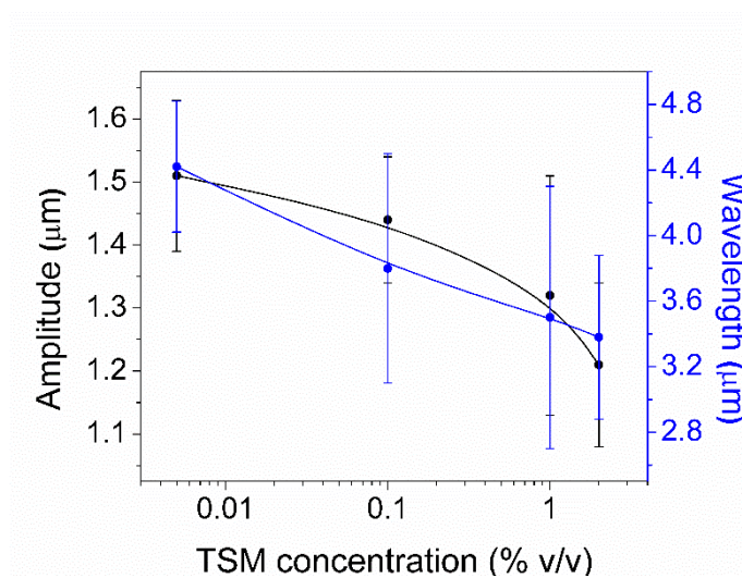
Figure S1. Amplitude and wavelength of the wrinkled patterns obtained by using different concentrations of TSM (0.005 %, 0.1 %, 1 %, and 2 % v/v) during functionalization process.
