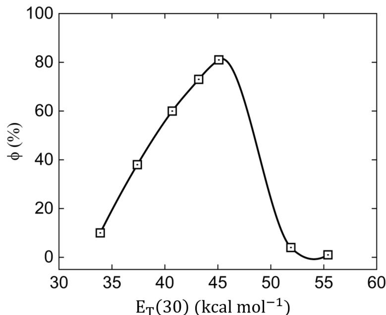
Figure 5. Fluorescence quantum yields of \text{ChN(CH}_3)_2 for different solvents (in ascending order of E_T(30) : toluene, tetrahydrofuran, dichloromethane, dimethylsulfoxide, dimethylformamide, ethanol, and methanol) determined through the Brouwer method.
