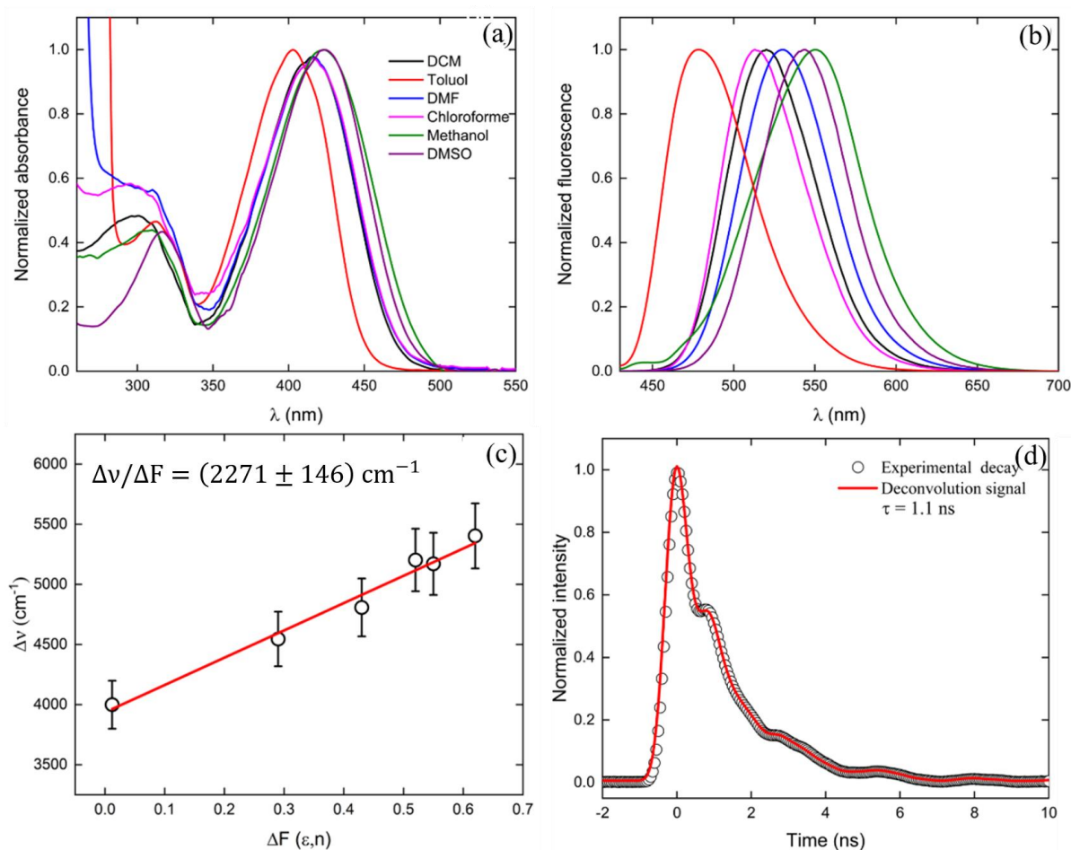
Figure 6. (a) linear absorption and (b) fluorescence emission of ChN(CH 3 ) 2 for different surrounding media (solvents). (c) represents the Stoke Shift (in wavenumber units) for different values of solvent polarity (in ascending order of \Delta F : toluene, chloroform, dichloromethane, dimethyl sulfoxide, dimethylformamide, and methanol), and (d) is the experimental (circles) fluorescence decay. The red line represents the adjustment considering the fluorescence experimental measurements and the instrument response function were convoluted.
