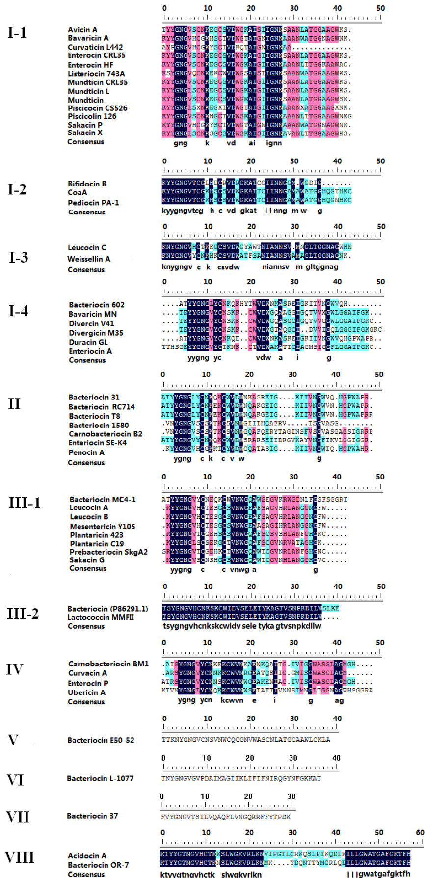
Figure 1. Multiple sequence alignment of class IIa bacteriocins.
