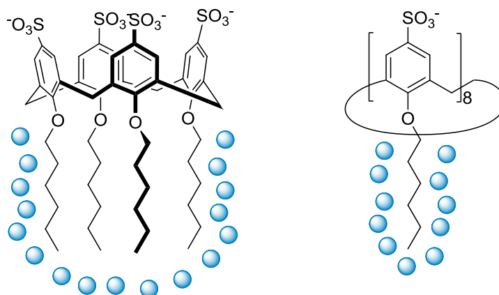
Figure 8. Conformation-dependent hydration of the alkyl chains of p -sulfonatocalix[ n ]arenes.
