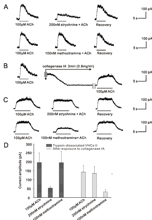
Figure 3. Change of the currents after exposure to collagenase IA on one trypsin-isolated cell. (A) Before exposure to collagenase IA, the trypsin-isolating cell displayed a typical fast inactivating current, which was strongly inhibited by 200 nM strychnine, but insensitive to 100 nM methoctramine; (B) 0.8 mg/mL collagenase IA dissociation solution was applied to the patched cell for 3 min. Note that there was a downward shift in the baseline; (C) After exposure to collagenase IA and incubated with normal external solution for 5 min, the fast inactivating current was totally abolished, while a non-inactivating current was activated. The non-inactivating current was insensitive to 200 nM strychnine, but could be potentially inhibited by 100 nM methoctramine. All of these above results were obtained from one same cell; (D) Bar histogram showed the inhibition effects of 200 nM strychnine and 100 nM methoctramine on the current evoked by 100 \mu M ACh. Each point represents the mean \pm SD of 6 cells. ( V_{\text{hold}} = -50 mV).
