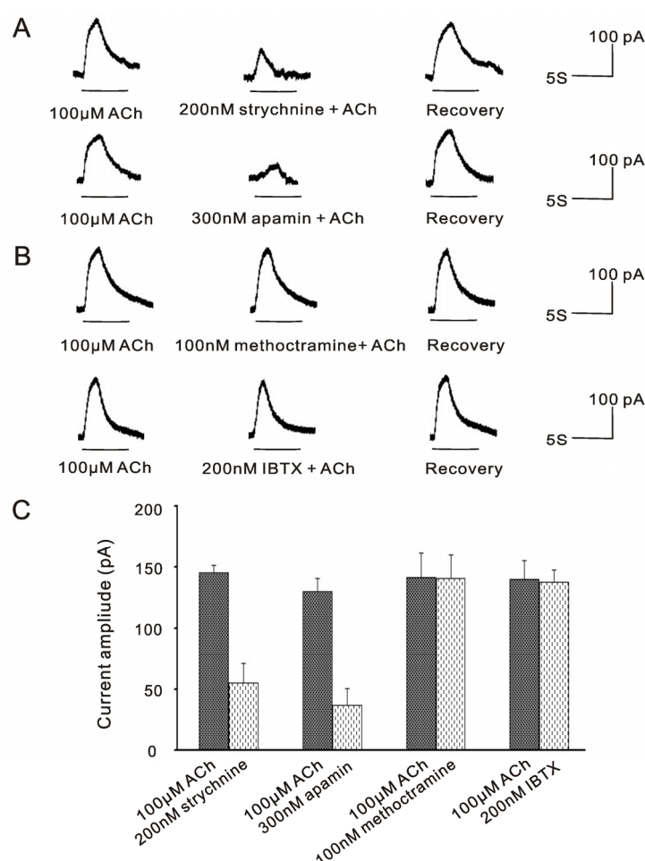
Figure 2. ACh activated SK2 currents in trypsin-isolated VHCs II. ACh routinely activated a fast inactivating outward current. (A) The current activated by 100 \mu M ACh was potently inhibited by strychnine and apamin, respectively; (B) The current activated by 100 \mu M ACh was insensitive to methoctramine and IBTX, respectively. All of these four results were obtained from the one same cell; (C) Bar histogram showed the inhibition effects of 200 nM strychnine, 300 nM apamin, 100 nM methoctramine and 200 nM IBTX on the current evoked by 100 \mu M ACh. Each point represents the mean \pm SD of 6 cells. ( V_{\text{hold}} = -50 mV).
