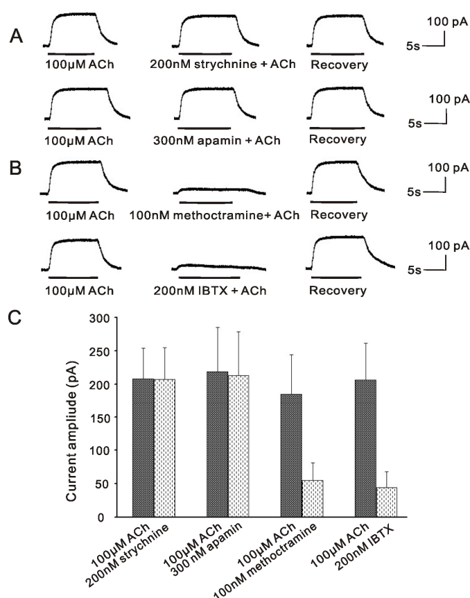
Figure 1. ACh-activated BK currents in collagenase IA isolated VHCs II. ACh routinely activated a non-inactivating outward current. (A) The current activated by 100 \mu M ACh was insensitive to strychnine and apamin, respectively; (B) The current activated by 100 \mu M ACh was potently inhibited by methoctramine and IBTX, respectively. All of these four results were obtained from the one same cell; (C) Bar histogram showed the effects of 200 nM strychnine, 300 nM apamin, 100 nM methoctramine and 200 nM IBTX on the current evoked by 100 \mu M ACh. Each point represents the mean \pm SD of 5–6 cells. ( V_{\text{hold}} = -50 mV).
