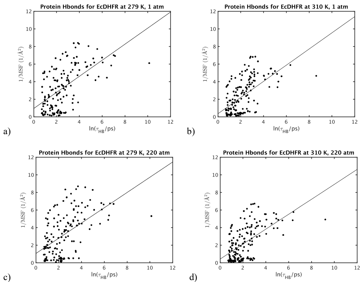
Figure S2. Correlation of inverse atomic fluctuations of hydrogen bond acceptors with the associated hydrogen bond lifetimes longer than 2 ps for EcDHFR at different conditions. Correlation coefficients: a) 0.594, b) 0.588, c) 0.535, d) 0.592.
