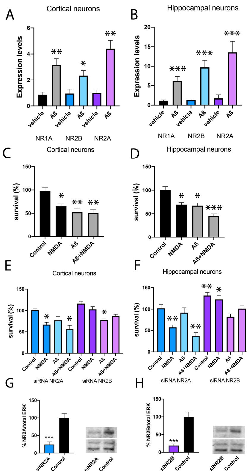
Figure 3. Analysis of neuronal survival in primary cultures silenced for NR2A or NR2B. (A,B) NR2A and NR2B expression levels were determined by RT-PCR in cortical and hippocampal primary cultures of neurons treated with Aβ1-42 (1 μM) or vehicle for 48 h. (C–F) Cortical and hippocampal primary cultures of neurons were transfected with siRNA for NR2A (blue), siRNA for NR2B (violet) or vehicle (black) and treated with Aβ1-42 (1 μM) or vehicle for 48 h followed by NMDA stimulation (15 mM) or vehicle for 24 h. Then, neurons were gently detached and mixed with an equal volume of trypan blue (0.4%) and counted with a TC20™ Automated Cell Counter (Biorad, 1450102). Values are the mean ± S.E.M. of 5 independent experiments performed in triplicates. One-way ANOVA
