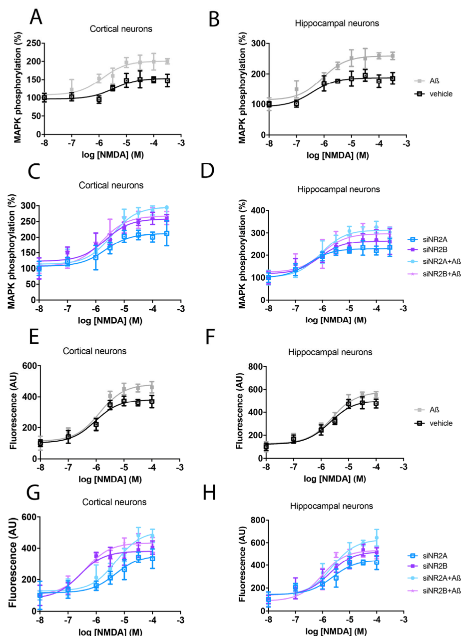
Figure 5. Differential signalling of NMDAR-containing NR2A or NR2B subunits in primary cultures of neurons treated with A \beta 1-42. Cortical and hippocampal primary cultures of neurons were transfected with siRNA for NR2A (blue), siRNA for NR2B (violet) or vehicle (black) and treated with A \beta 1-42 (1 \mu M) or vehicle for 48 h. After, cells were stimulated with a range of NMDA concentrations (10 nM to 300 \mu M) or vehicle for 10 min in MAPK phosphorylation assays or a few seconds when
