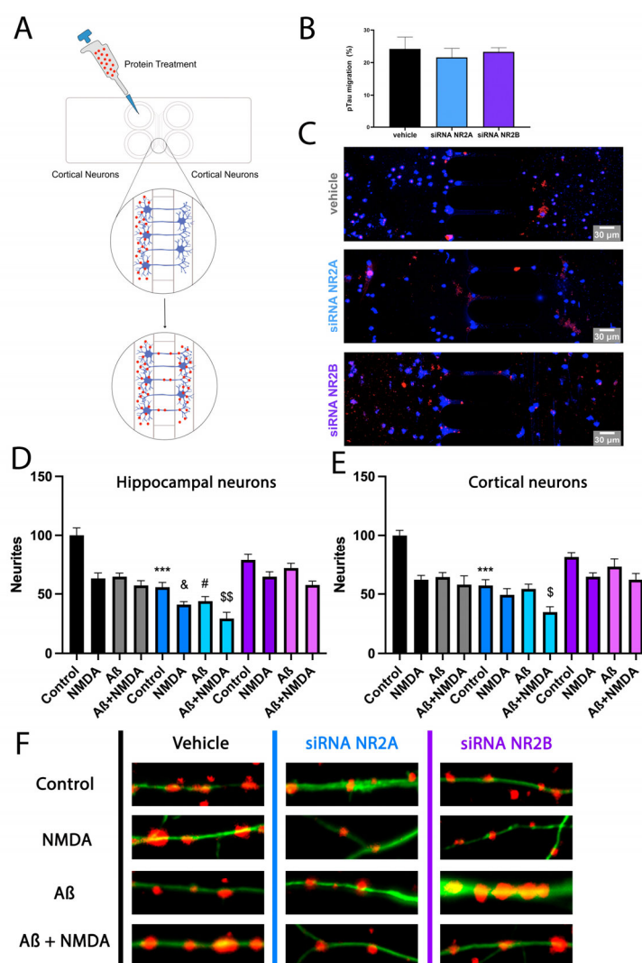
Figure 6. Effect of NMDAR-containing NR2A or NR2B subunits in pTau migration and neurite patterning in primary cultures of neurons treated with A \beta 1-42. (A–C) Mice cortical neurons were
