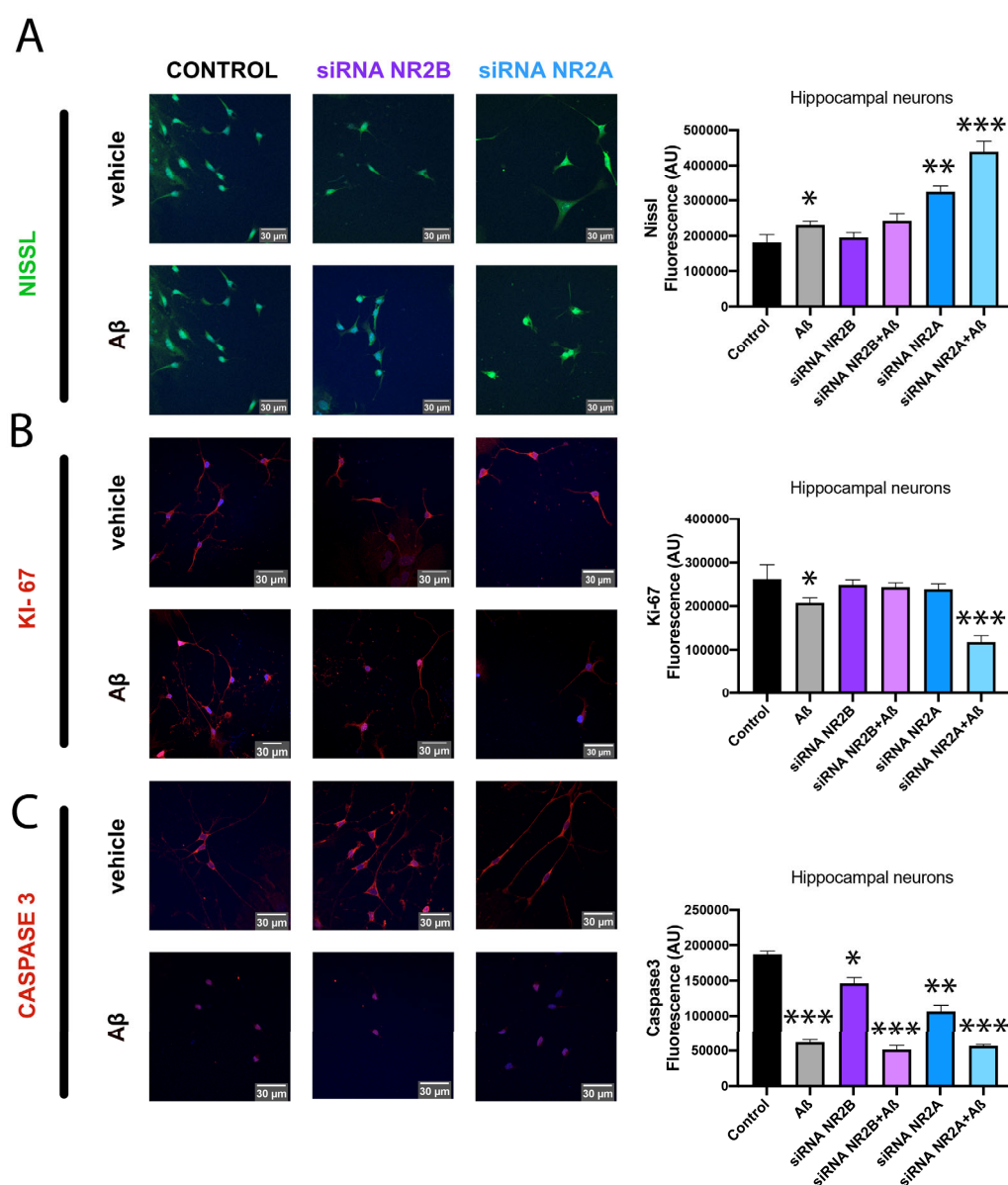
Figure 4. Immunocytochemistry assay of neuronal morphology in primary cultures treated with Aβ1-42. Immunocytochemistry assay was performed in hippocampal primary cultures of neurons transfected with siRNA for NR2A (blue), siRNA for NR2B (violet) or vehicle (black) and treated with Aβ1-42 (1 μM) or vehicle for 48 h. Neuronal survival was characterised by incubating with the specific antibodies: anti-Nissl (neuronal morphology) (A), anti-Ki-67 (neuronal proliferation) (B) or anti-Caspase3 (neuronal plasticity) (C). Detection is shown in green (A) or red (B,C) due to incubation with a secondary antibody conjugated to a fluorochrome Alexa 488 or Alexa 561, respectively. Scale bar: 30 μm. Values are the mean ± S.E.M. of 6 independent experiments performed in triplicates. One-way ANOVA followed by Bonferroni's multiple comparison post hoc test was used for statistical analysis (* p < 0.05 , ** p < 0.01 , *** p < 0.001 versus control condition).
