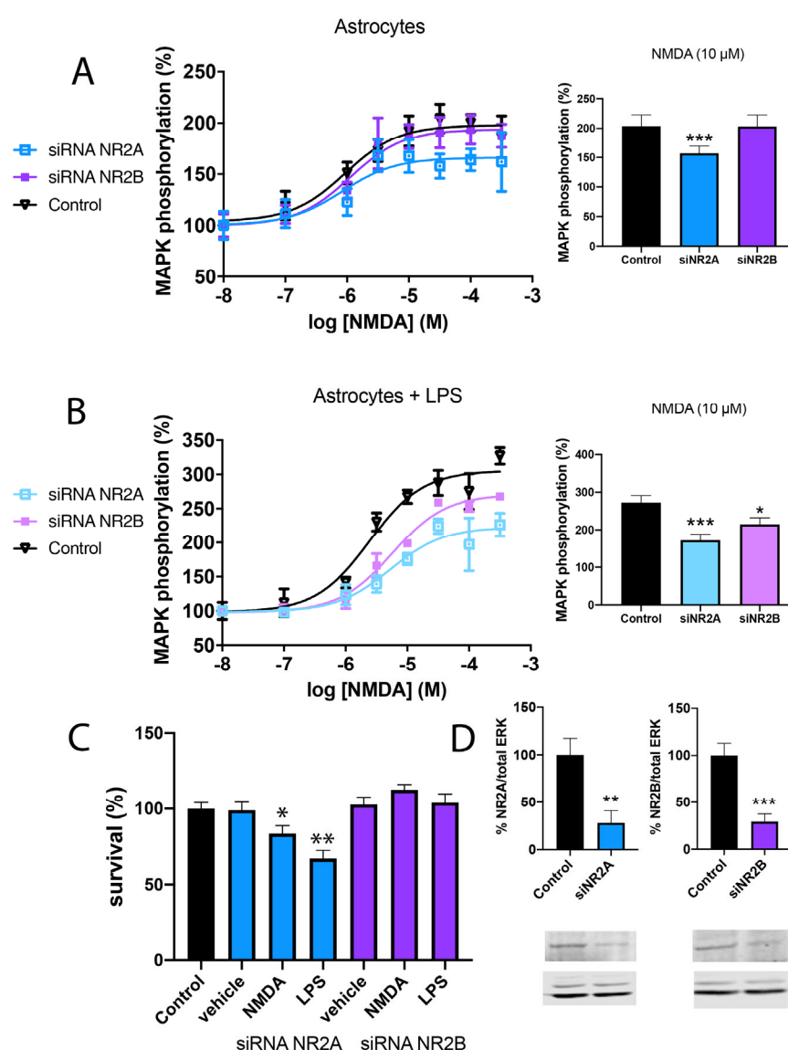
Figure 2. Differential signalling of NMDAR-containing NR2A or NR2B subunits in primary cultures of astrocytes. Primary cultures of astrocytes were transfected with siRNA for NR2A (blue), siRNA for NR2B (violet) or vehicle (black) and treated with 1 \mu M LPS plus 200 U/mL IFN- \gamma (B,C) or vehicle
