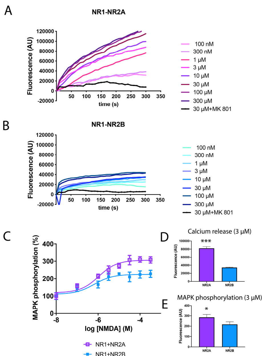
Figure 1. Differential signalling of NMDAR-containing NR2A or NR2B subunits in transfected HEK-293T cells. ( A,B,D ) HEK-293T cells were transfected with the cDNAs for the NMDAR subunits NR1A (0.6 μg/well), NR2A (0.6 μg/well) ( A ) or NR2B (0.6 μg/well) ( B ) and the calcium sensor GCaMP6 (0.5 μg/well). Cells were pre-treated with MK-801 (1 μM) or vehicle and treated with increasing concentrations of NMDA (100 nM to 300 μM). Real-time calcium-induced fluorescence was collected for 300 s. Values are representative curves of 8 independent experiments performed in duplicates. ( C,E ) HEK-293T cells were transfected with the cDNAs NR1A (0.6 μg/well), NR2A (0.6 μg/well) (violet) or NR2B (0.6 μg/well) (blue). Cells were treated with increasing concentrations of NMDA (10 nM to 300 μM) and ERK1/2 phosphorylation was analysed using an AlphaScreen®Sure-Fire® kit (Perkin Elmer, Waltham, MA, USA). Values are the mean ± S.E.M. of 6 independent experiments performed in triplicates. ( D,E ) Calcium release and MAPK phosphorylation induced by 3 μM NMDA at 250 after activation. Values are the mean ± S.E.M. of 8 independent experiments performed in duplicates. One-way ANOVA followed by Bonferroni's multiple comparison post hoc test was used for statistical analysis (* p < 0.05 , *** p < 0.001 comparing NMDAR-containing NR2A versus NMDAR-containing NR2B).
