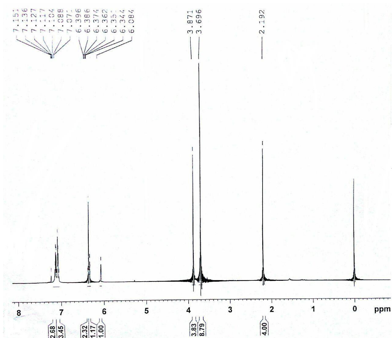
Figure.S7: 1 H NMR Spectrum of 2-methyl-5-phenyl-1-(3,4,5-trimethoxyphenyl)-1H-pyrrole. compound (3)
