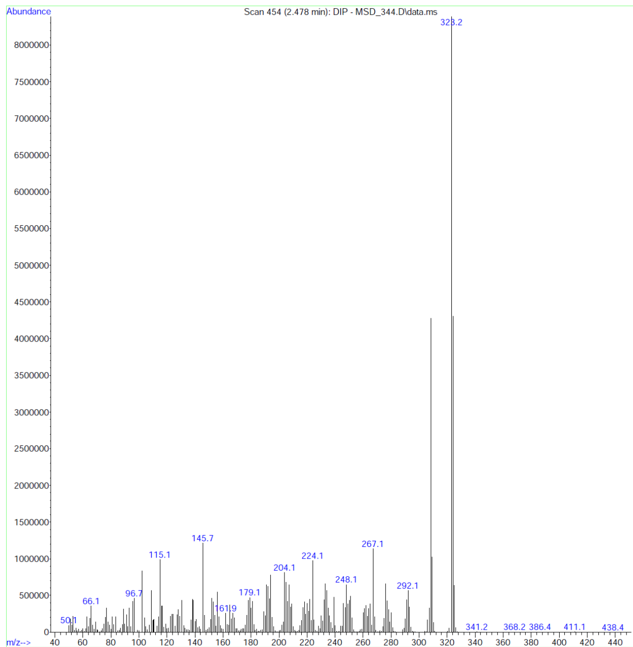
Figure.S11: Mass Spectrum of 2-methyl-5-phenyl-1-(3,4,5-trimethoxyphenyl)-1H-pyrrole. compound (3)
