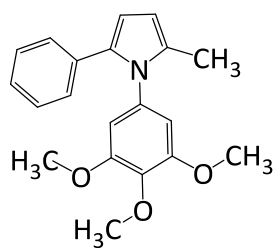
Structure of Compound 3
