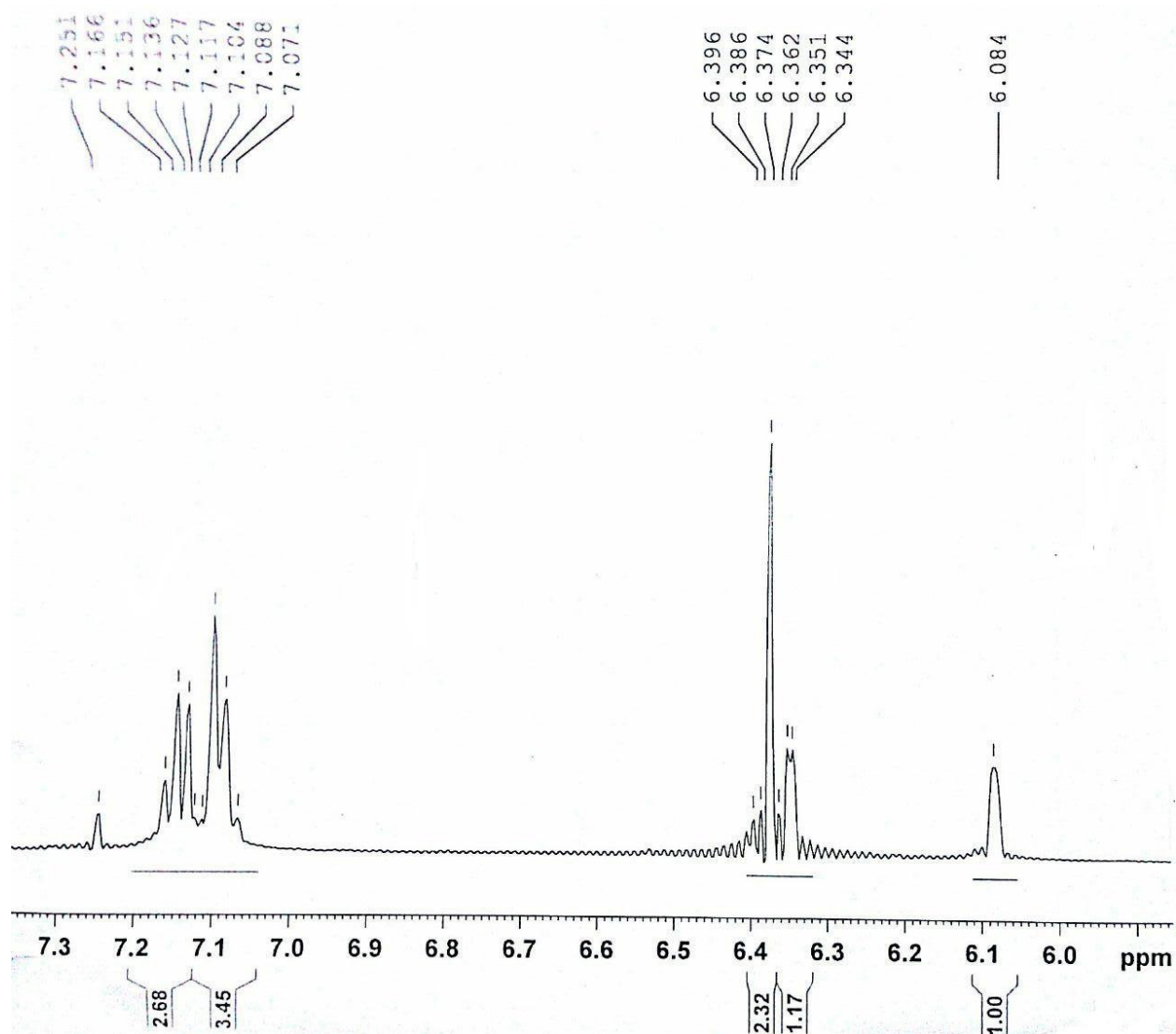
Figure.S8: 1 H NMR Spectrum of 2-methyl-5-phenyl-1-(3,4,5-trimethoxyphenyl)-1H-pyrrole. compound (3) - Expanded
