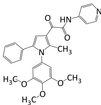
Structure of Compound 4
