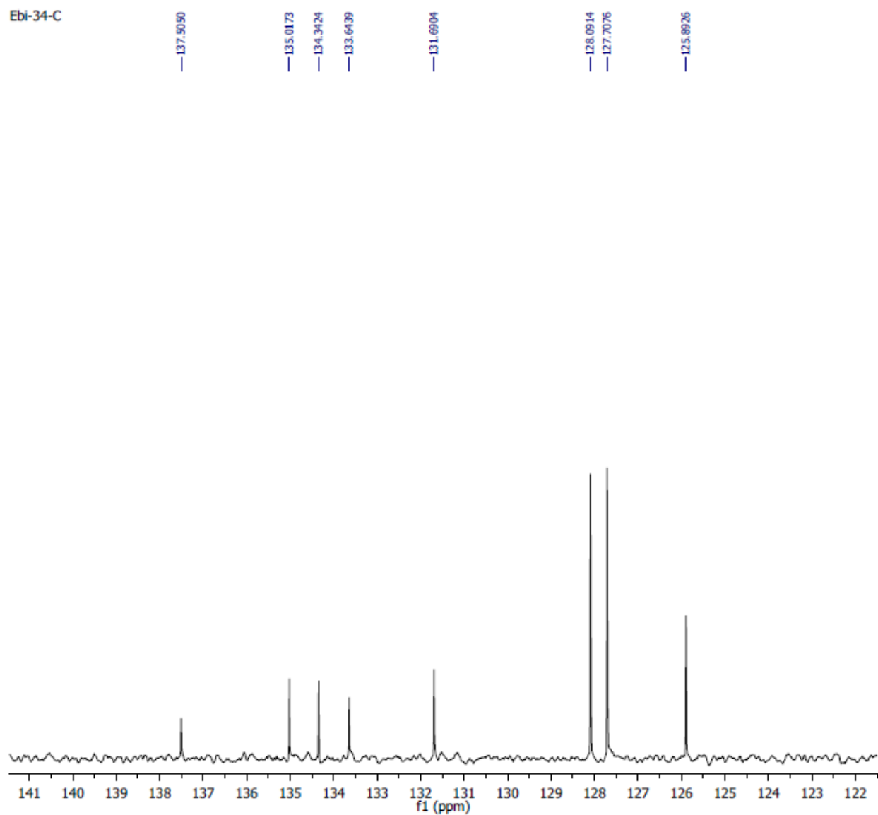
Figure.S10: ^{13}\text{C} NMR Spectrum of 2-methyl-5-phenyl-1-(3,4,5-trimethoxyphenyl)-1H-pyrrole. compound (3) – Expanded
