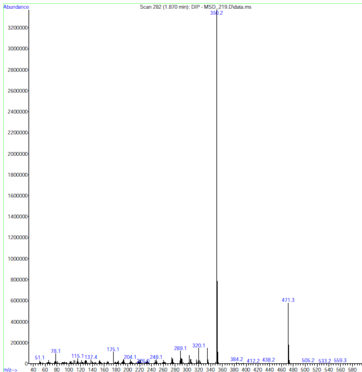
Figure.S6 -Mass spectrum of 2-(2-methyl-5-phenyl-1-(3,4,5-trimethoxyphenyl)-1H-pyrrol-3-yl)-2-oxo-N-(pyridin-4-yl) acetamide. Compound (4)
