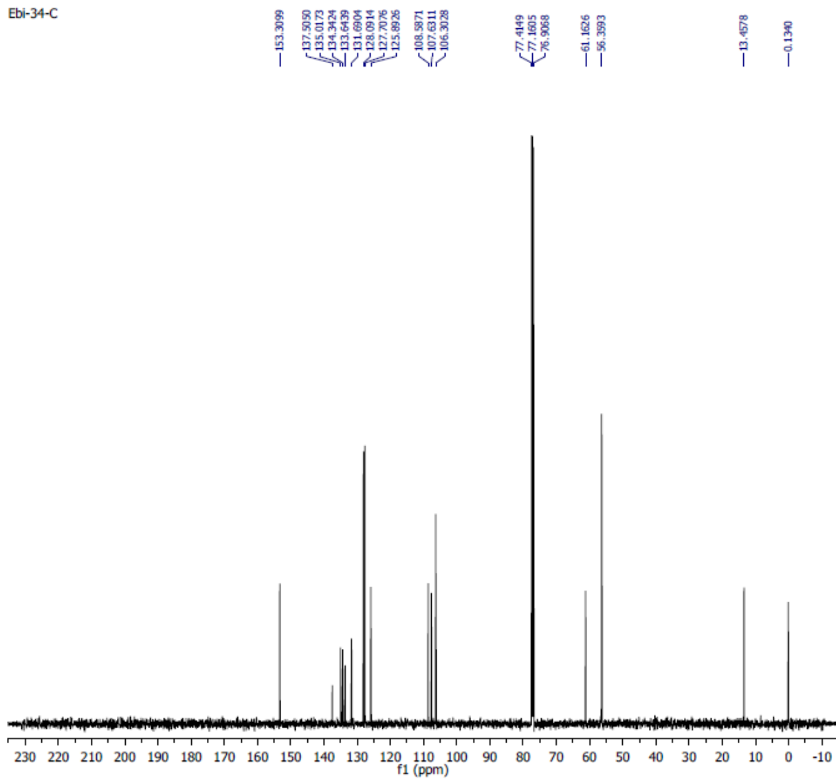
Figure.S9: 13 CNMR Spectrum of 2-methyl-5-phenyl-1-(3,4,5-trimethoxyphenyl)-1H-pyrrole. compound (3)
