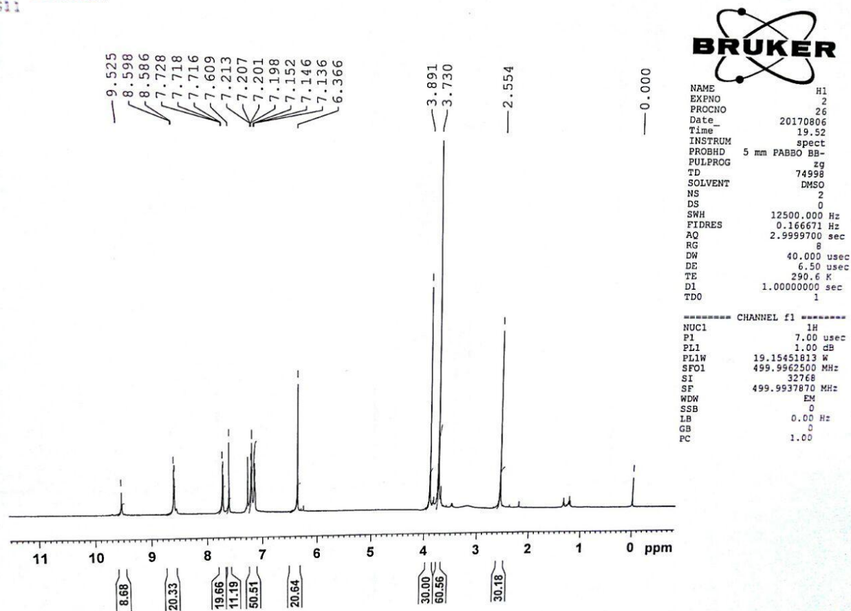
Figure.S1 - ^1\text{H} NMR spectrum of 2-(2-methyl-5-phenyl-1-(3,4,5-trimethoxyphenyl)-1H-pyrrol-3-yl)-2-oxo-N-(pyridin-4-yl) acetamide. Compound (4)
