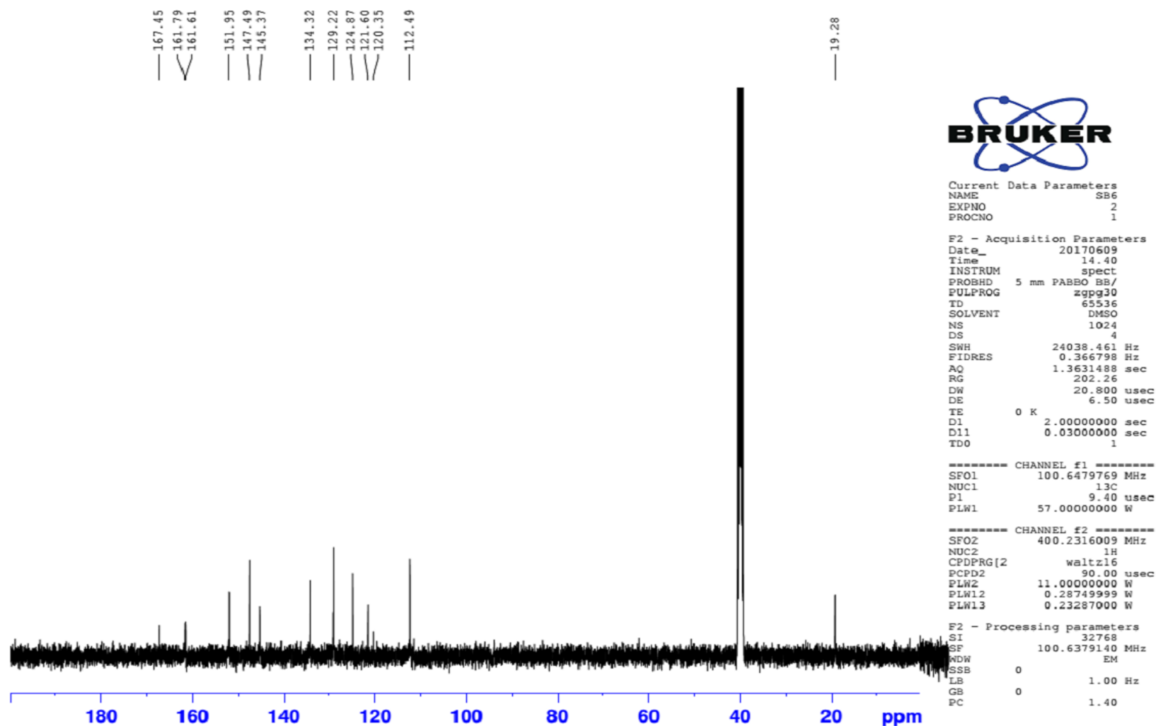
Figure S4. ^{13}\text{C} -NMR Spectrum of ( E )- N' -(4-fluorobenzylidene)-5-methyl-2-(pyridin-3-yl)thiazole-4-carbohydrazide
