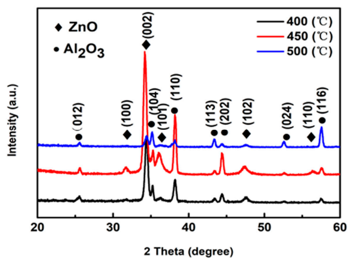
Fig. S1 XRD patterns of the ZnO film annealed at 400 °C, 450 °C and 500 °C, respectively.
