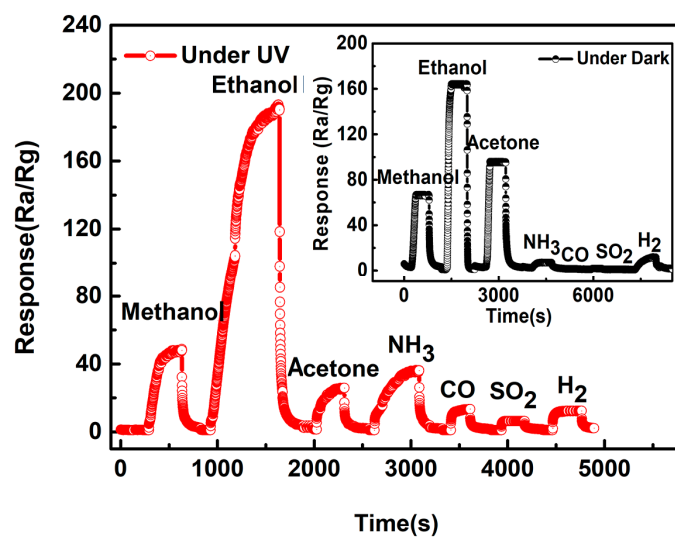
Fig. S4 Responses curve of the ZnO film sensor to various gases of 1000 ppm under dark and under UV light illumination.
