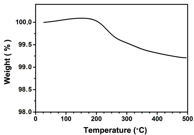
Fig. S2 TGA of the ZnO film from room temperature to 500 °C
