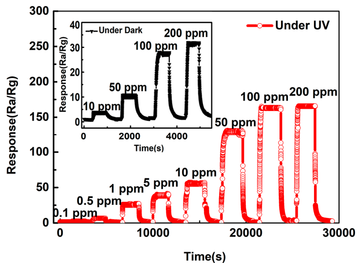
Fig. S3 Response curve of the ZnO film sensor to different concentrations of C_2H_5OH from 0.1 to 200 ppm under dark and under UV LED activation.
