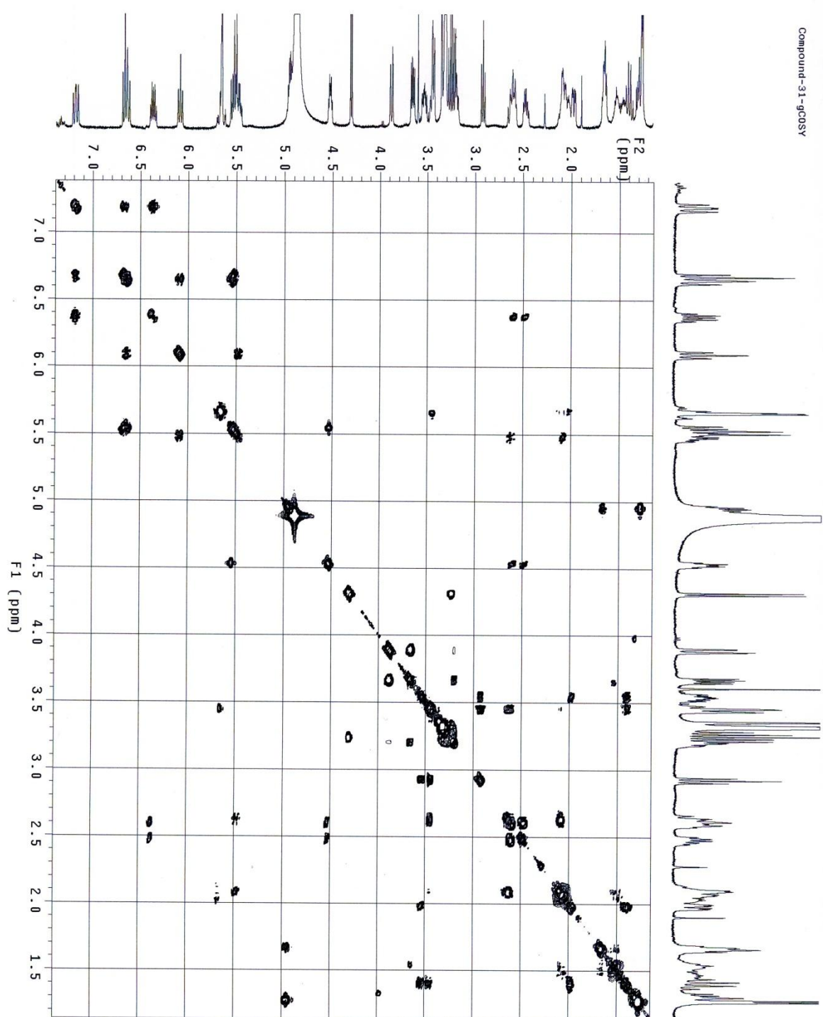
Figure S10. COSY spectrum of compound 2 in CD 3 OD.
