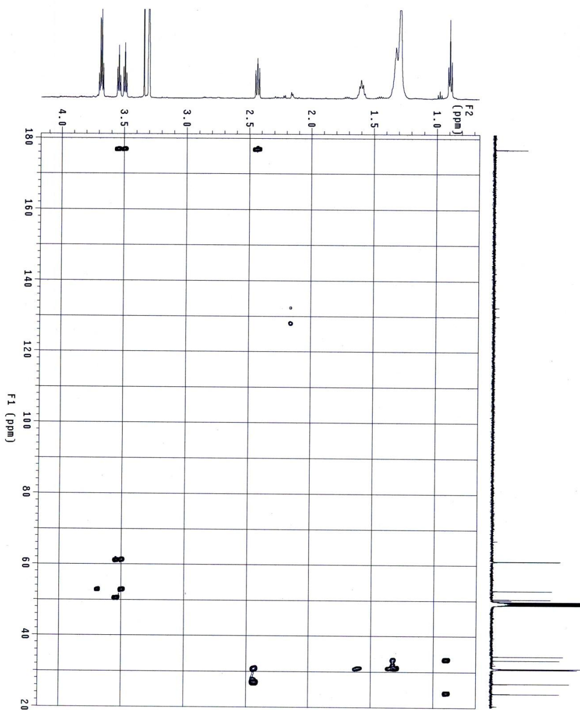
Figure S6. HMBC spectrum of compound 1 in CD 3 OD.
