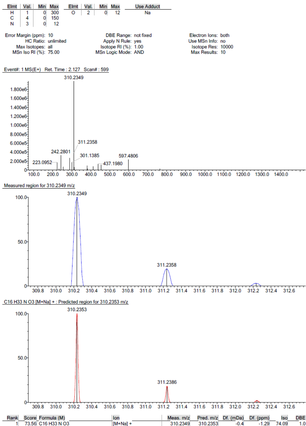
Figure S1. HRESIMS spectrum of compound 1 .
