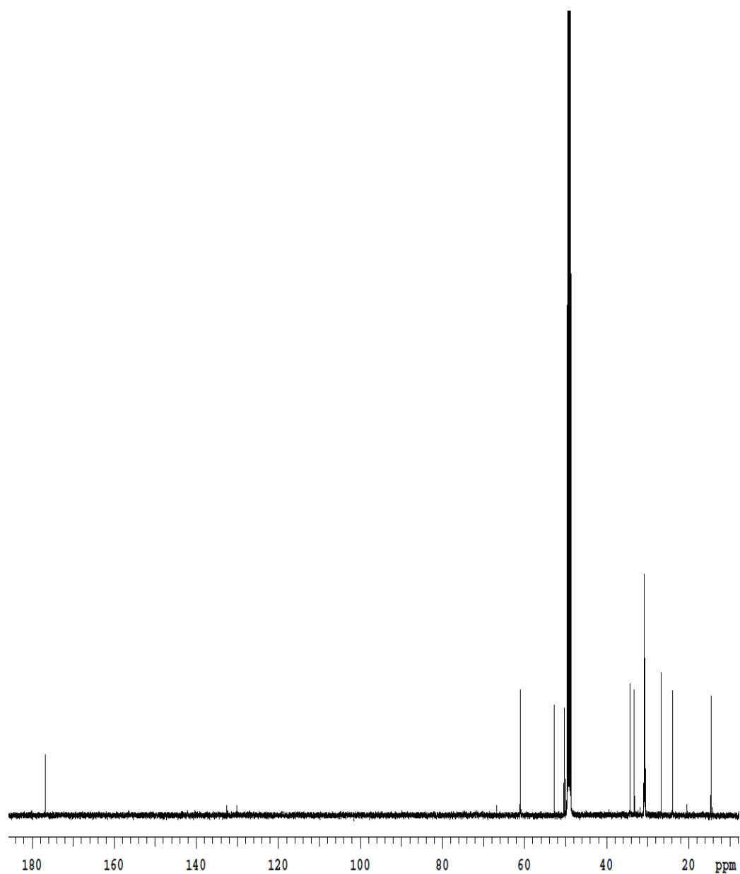
Figure S3. ^{13}\text{C} NMR spectrum of compound 1 recorded in \text{CD}_3\text{OD} at 125 MHz.
