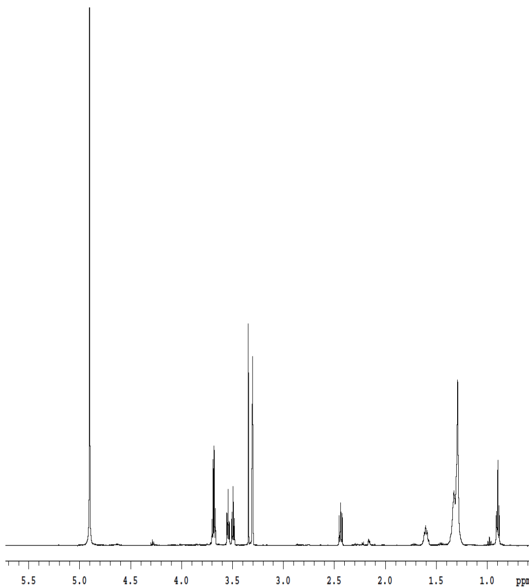
Figure S2. ^1\text{H} NMR spectrum of compound 1 recorded in \text{CD}_3\text{OD} at 500 MHz.
