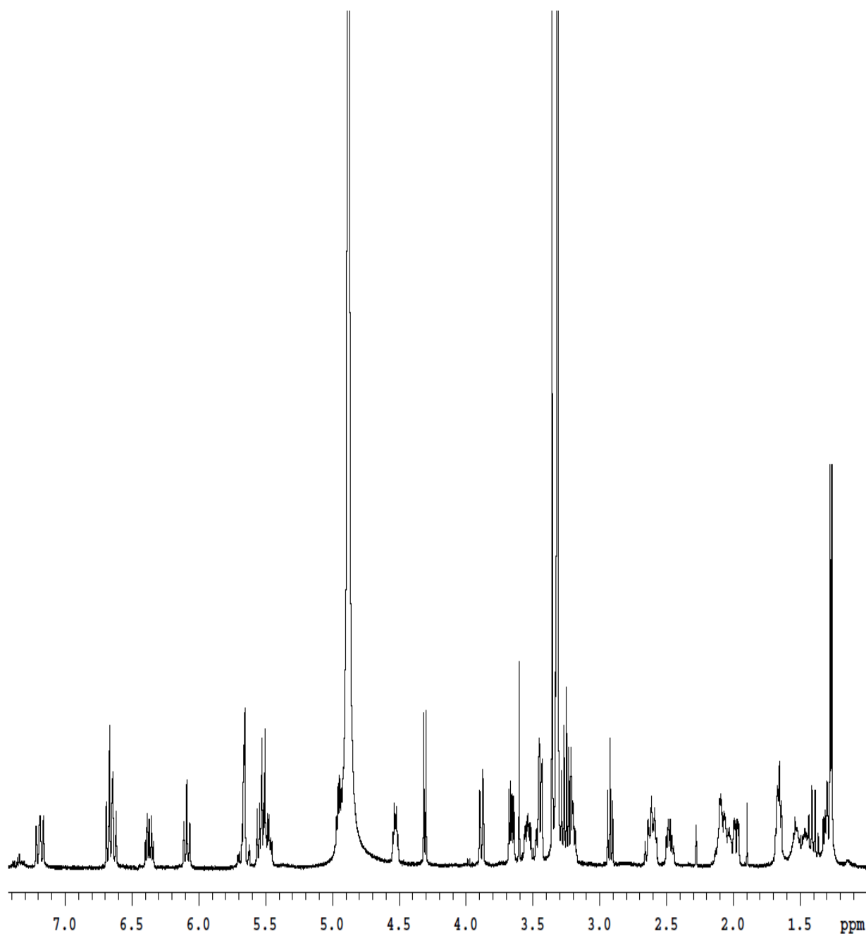
Figure S8. ^1\text{H} NMR spectrum of compound 2 recorded in \text{CD}_3\text{OD} at 500 MHz.
