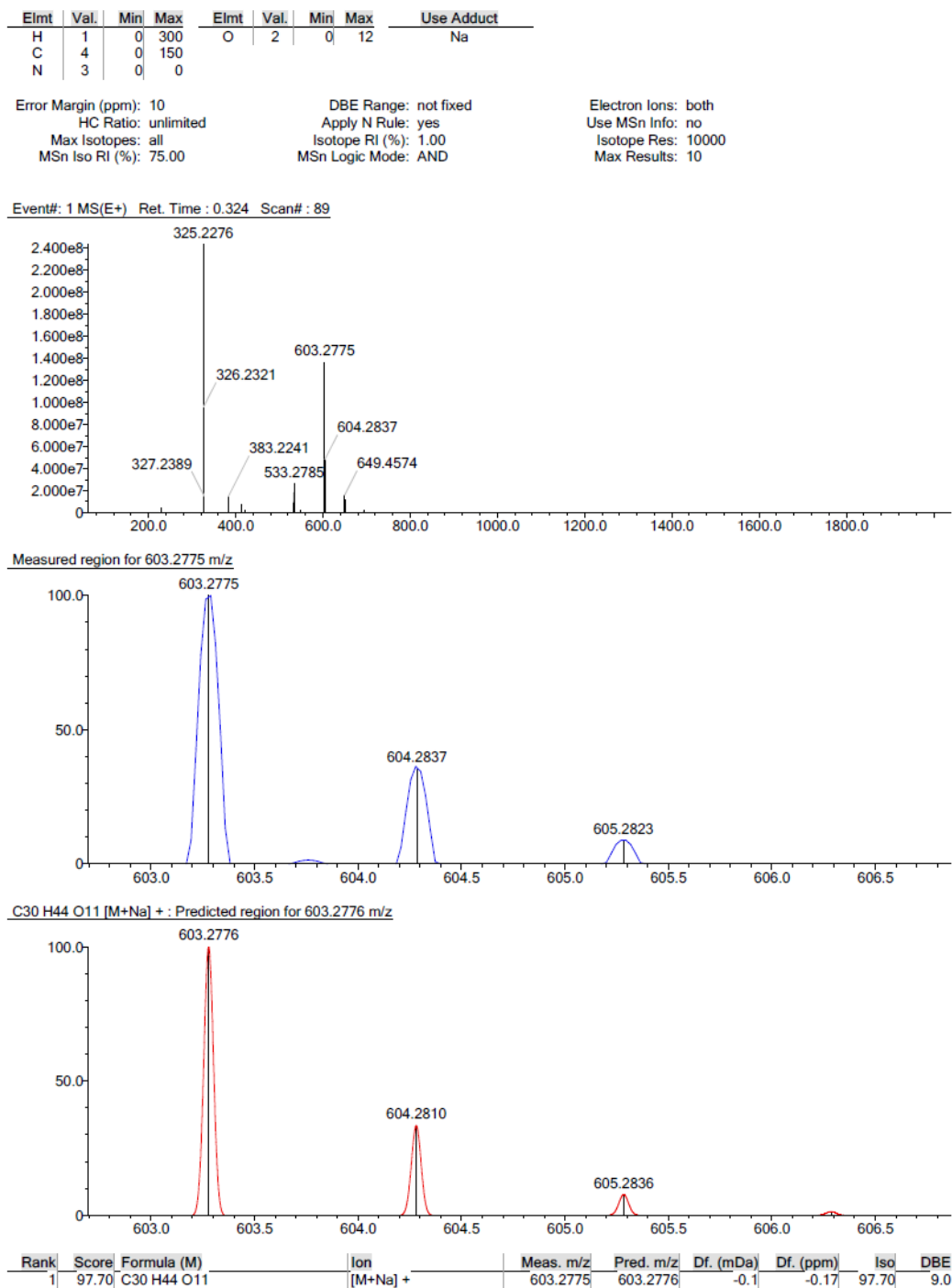
Figure S7. HRESIMS spectrum of compound 2.
