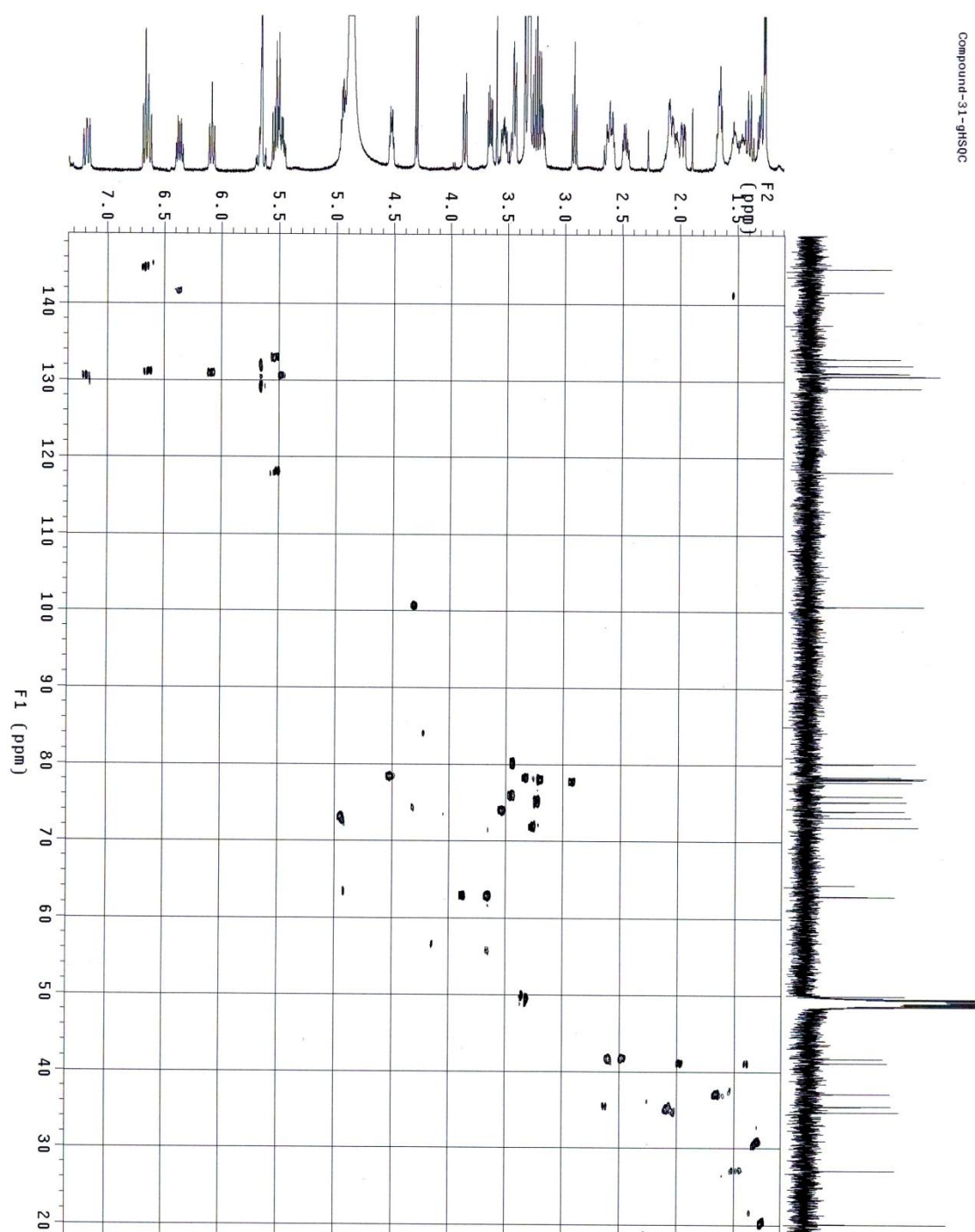
Figure S11. HSQC spectrum of compound 2 in CD 3 OD.
