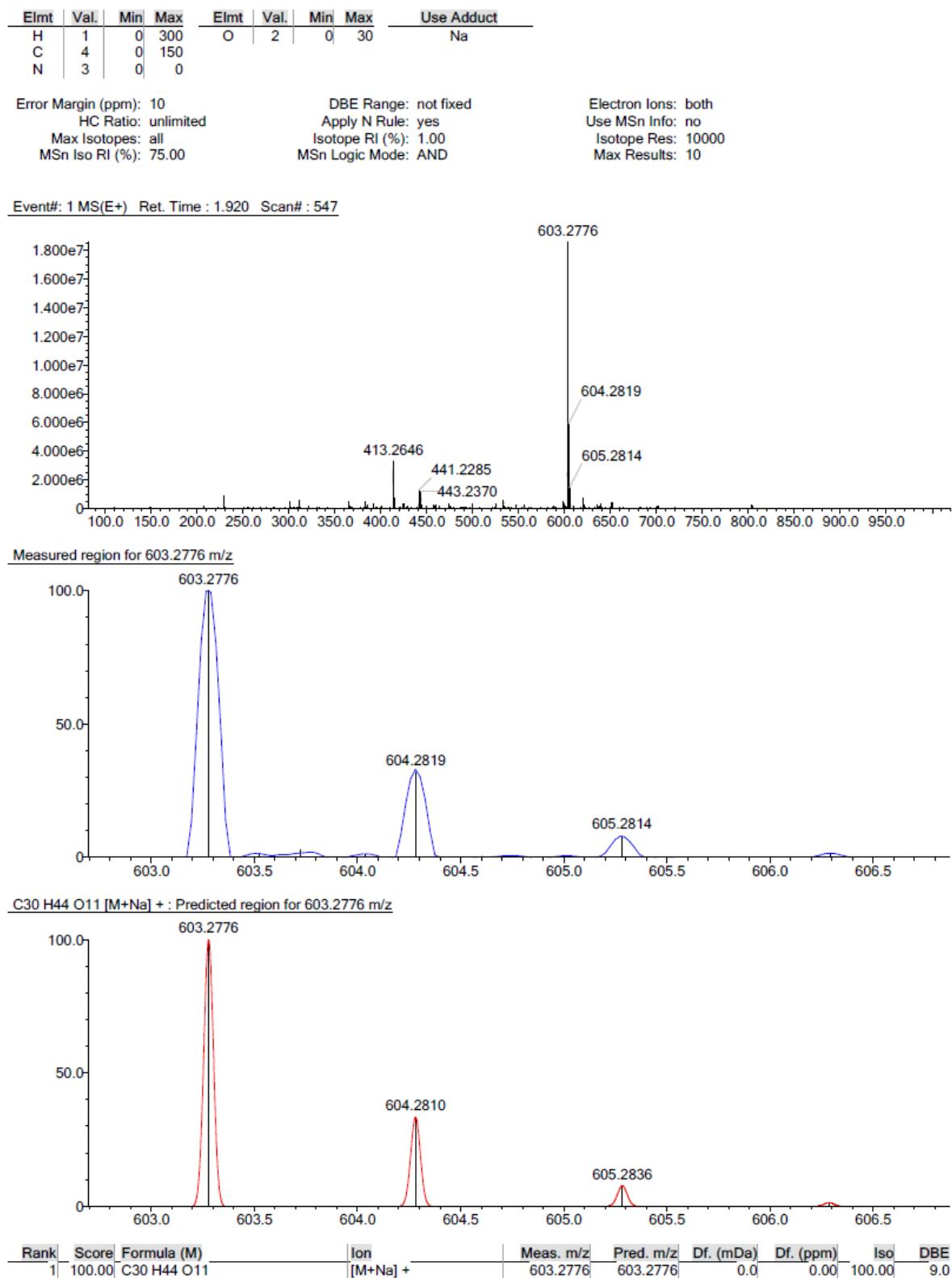
Figure S12. HRESIMS spectrum of compound 3 .
