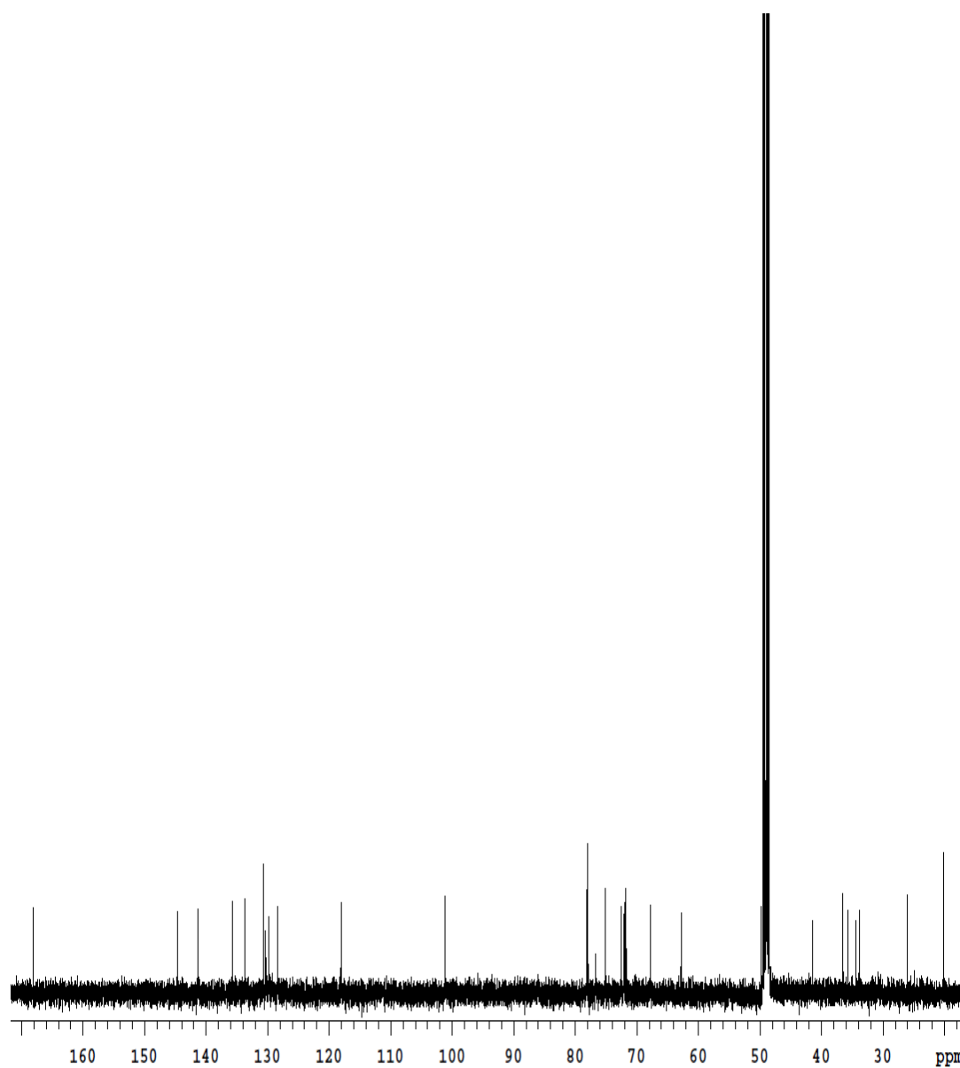
Figure S14. ^{13}\text{C} NMR data of compound 3 recorded in \text{CD}_3\text{OD} at 125 MHz.
