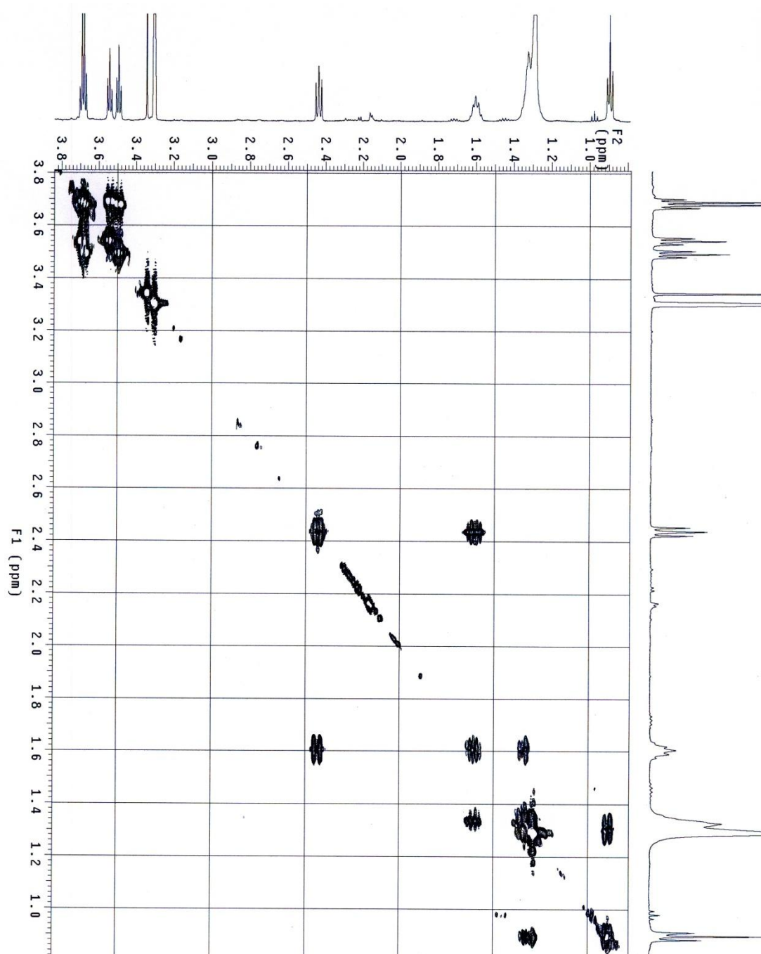
Figure S4. COSY spectrum of compound 1 in CD 3 OD.
