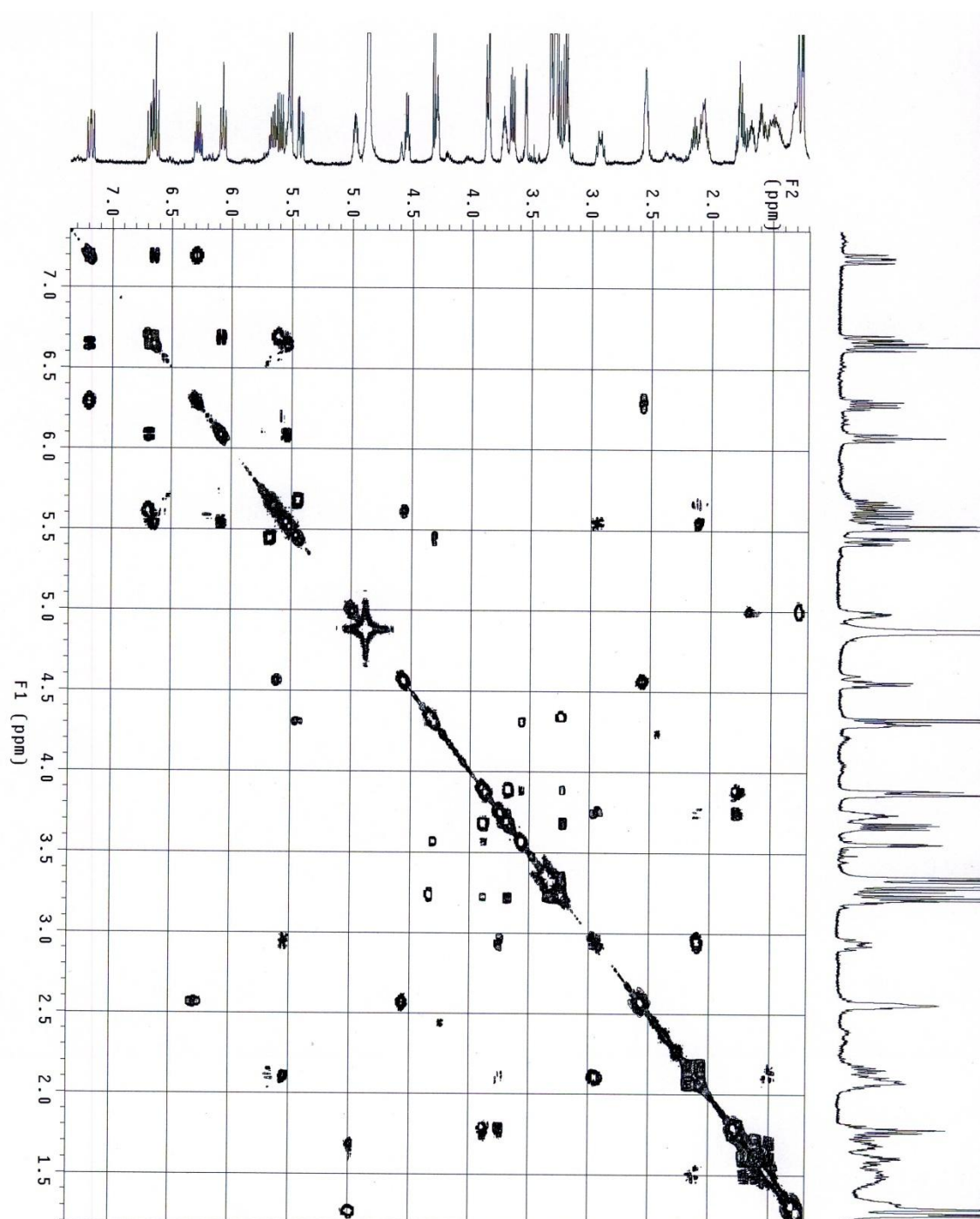
Figure S15. COSY spectrum of compound 3 in CD 3 OD.
