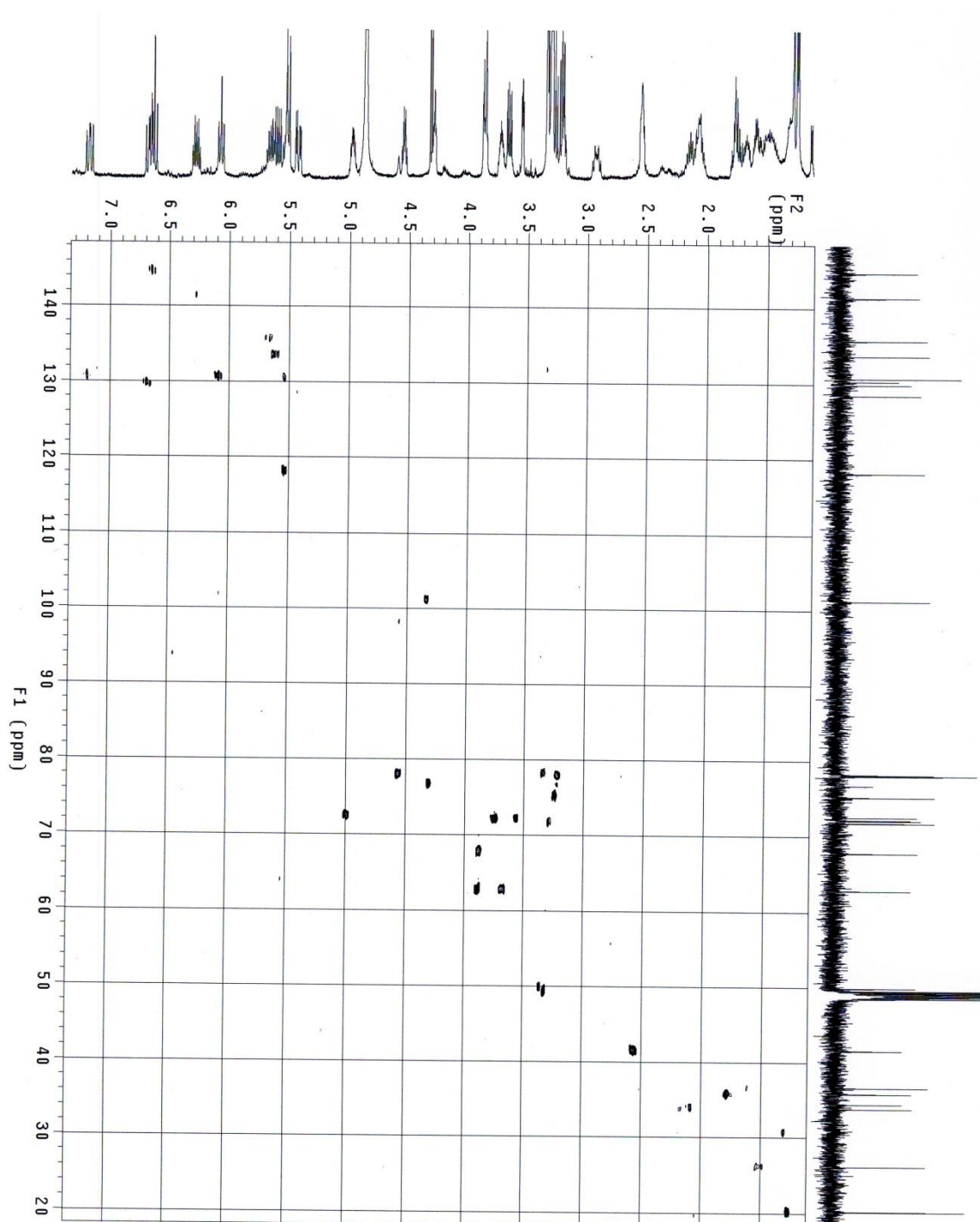
Figure S16. HSQC spectrum of compound 3 in CD 3 OD.
