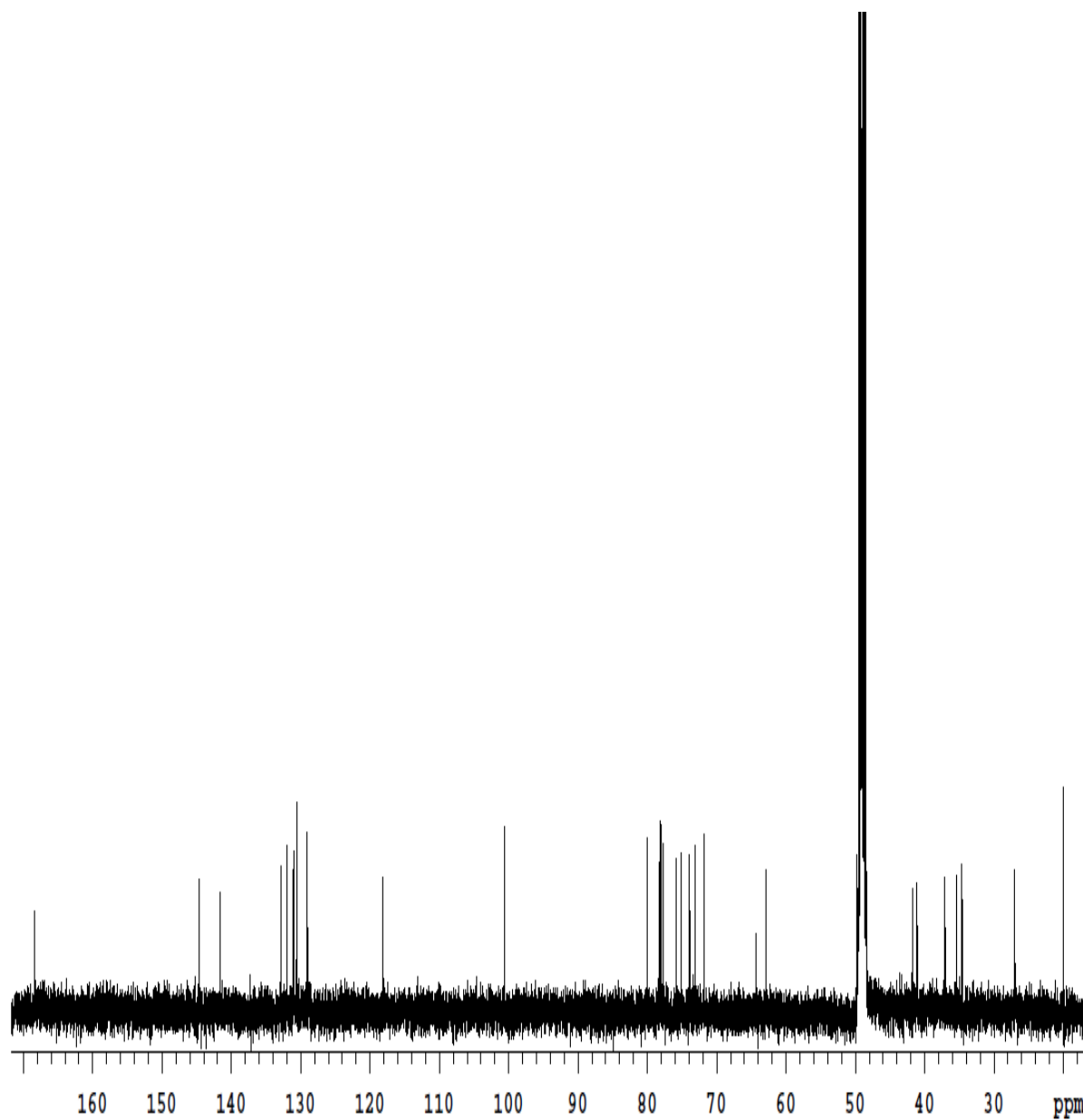
Figure S9. ^{13}\text{C} NMR of compound 2 recorded in \text{CD}_3\text{OD} at 125 MHz.
