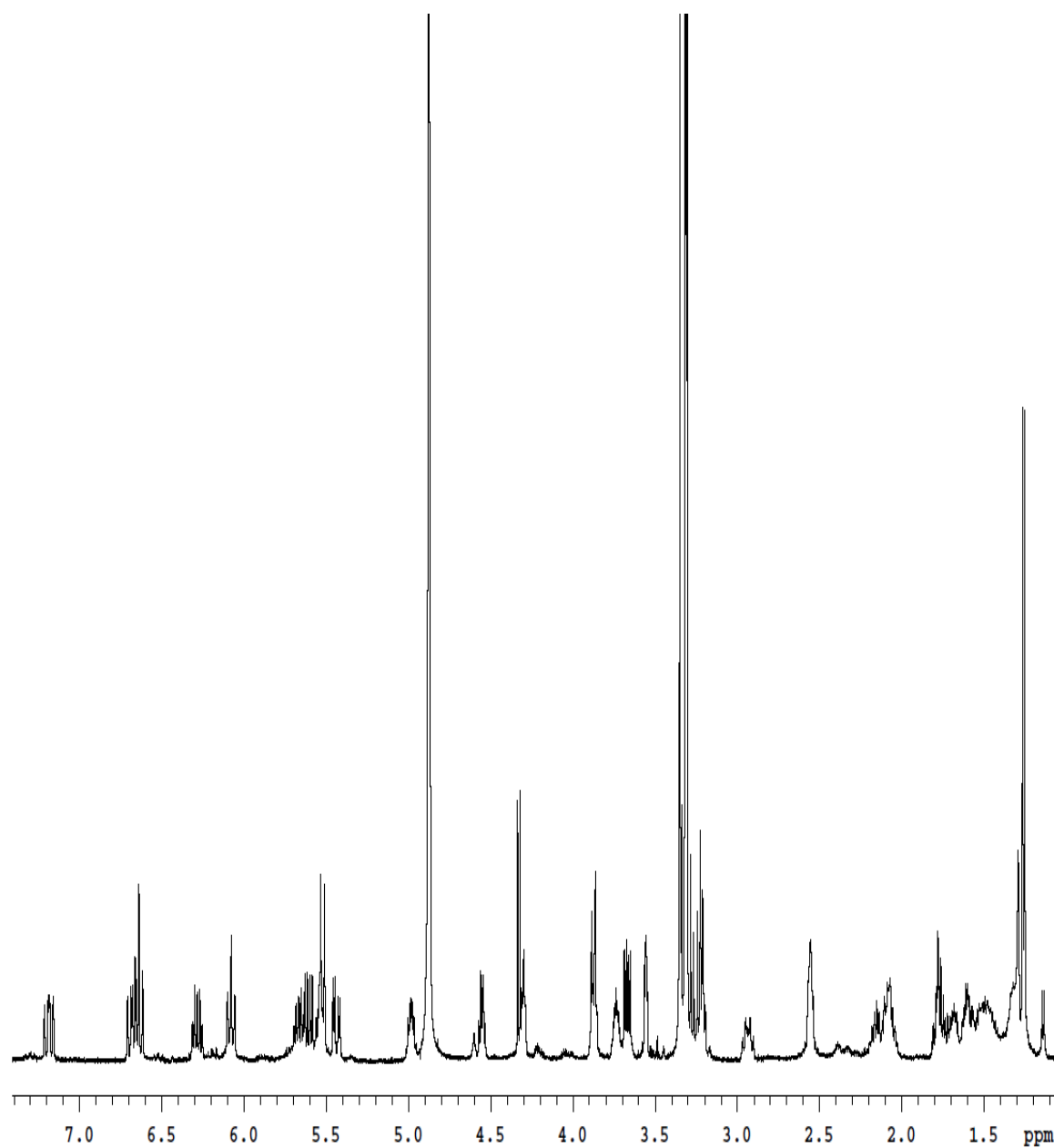
Figure S13. ^1\text{H} NMR data of compound 3 recorded in \text{CD}_3\text{OD} at 500 MHz.
