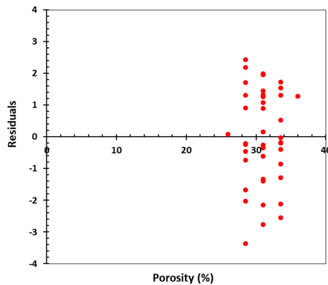
Figure 21. Residuals vs. porosity for the database analyzed.
