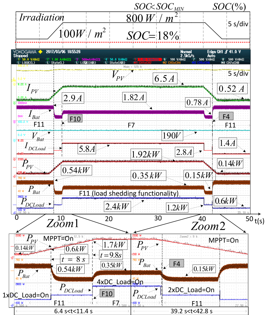
Figure 11. Experiment 2.
