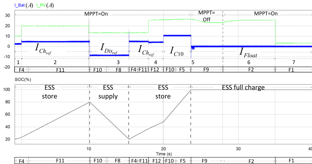
Figure 6. Simulation waveforms, I_{\text{Bat}} , I_{\text{PV}} = I_{\text{PV1}} + I_{\text{PV2}} the SOC over time.
