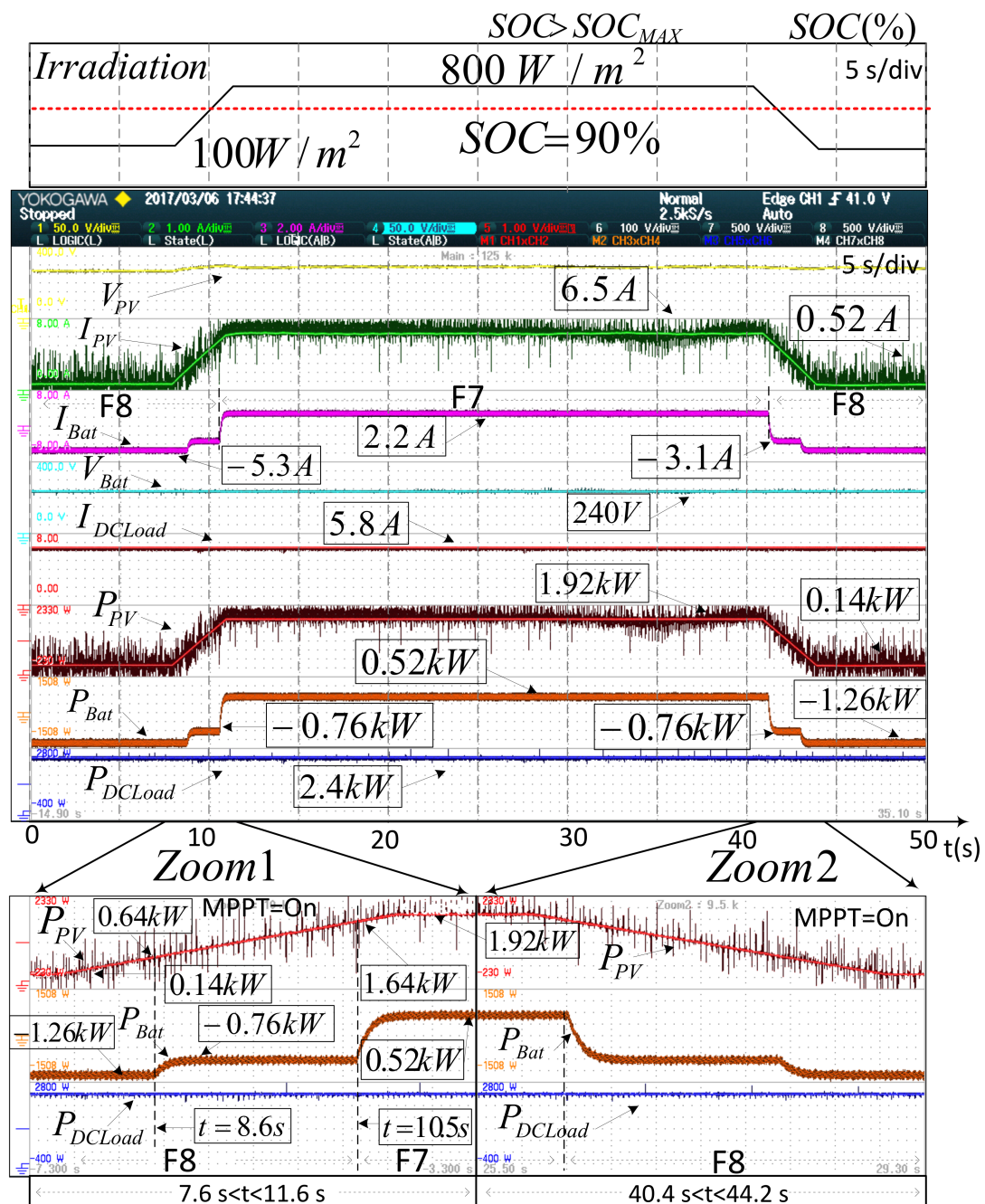
Figure 10. Experiment 1.
