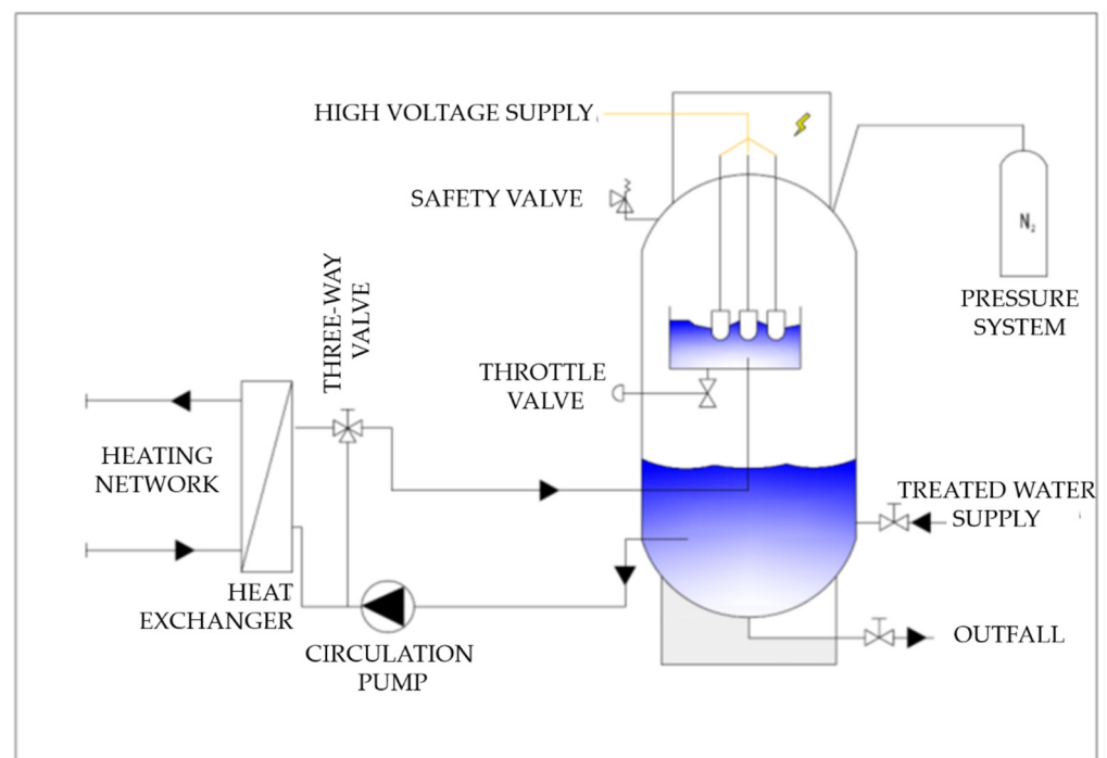
Figure 12. Scheme of the electrode boiler.
