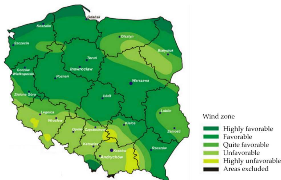
Figure 9. Wind map in Poland [66].
