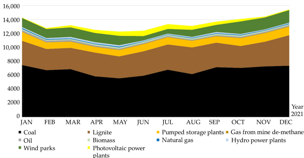
Figure 7. Electricity production in Poland in 2021 (GWh).
