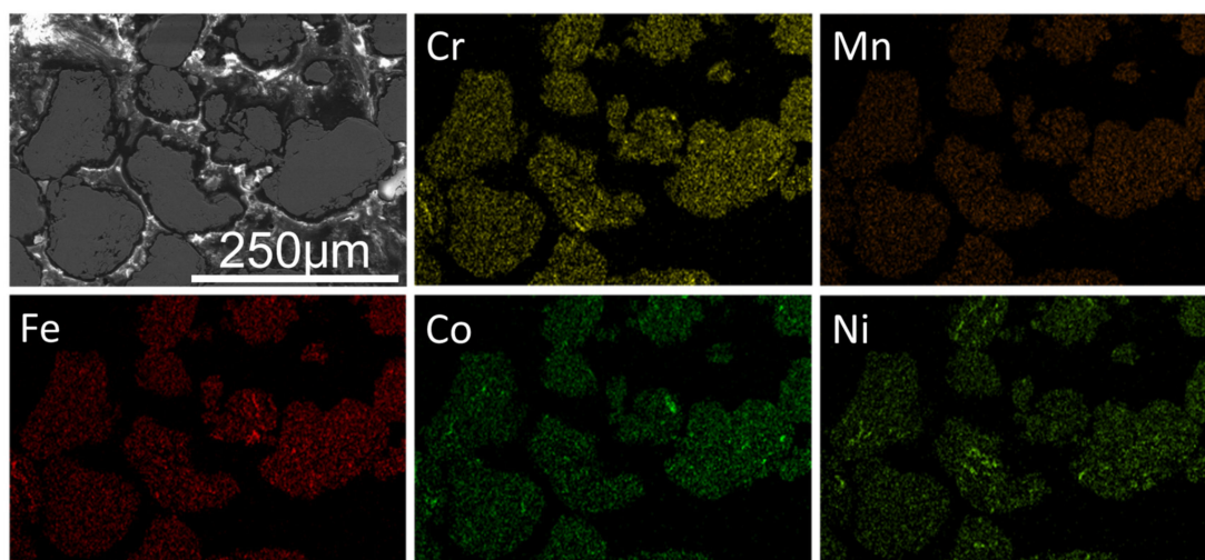
Figure 3. SEM image and EDS maps of 50 h-milled powders.
