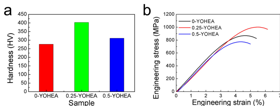
Figure 8. (a) Microhardness and (b) tensile curves of CrMnFeCoNi composites after SPSe.
