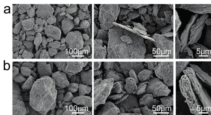
Figure 5. SEM images of HEA powders with different \text{Y}_2\text{O}_3 content after milling for 50 h: (a) 0.25-YOHEA; (b) 0.5-YOHEA.
