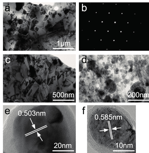
Figure 7. TEM images of SPSe HEAs: (a) 0-YOHEA; (b) Selected area diffraction in (a); (c) 0.25-YOHEA; (d) 0.5-YOHEA; (e) HRTEM image of a single Y_2O_3 in (c); (f) HRTEM image of a single Y_2O_3 in (d).
