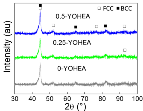
Figure 4. XRD patterns of HEA powders with different \text{Y}_2\text{O}_3 content after milling for 50 h.
