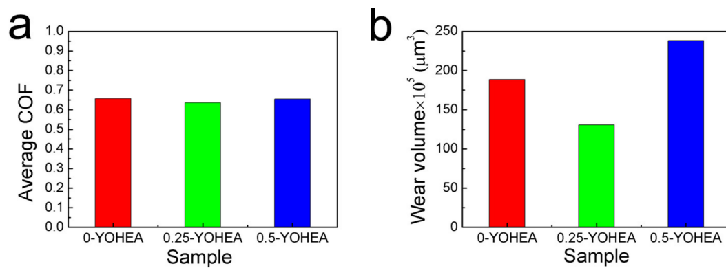
Figure 10. Average COF and wear loss of HEA composites.
