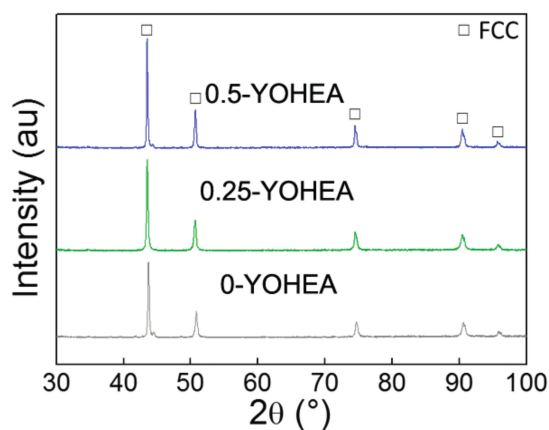
Figure 6. XRD patterns of HEA composites with different \text{Y}_2\text{O}_3 content.
