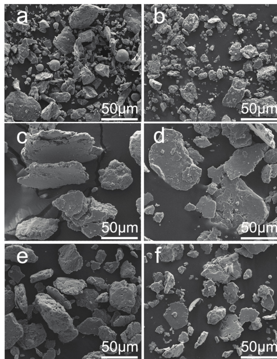
Figure 2. SEM images of CrMnFeCoNi powders with different milling times: (a) 1 h; (b) 10 h; (c) 20 h; (d) 30 h; (e) 40 h; (f) 50 h.
