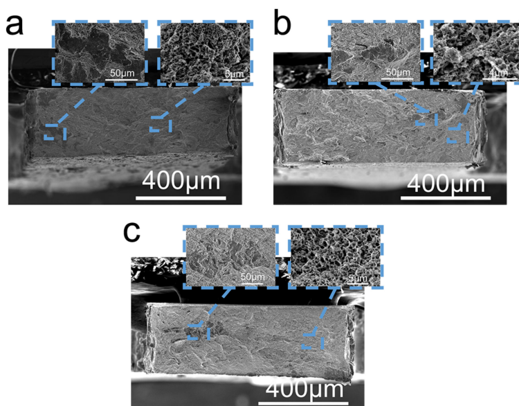
Figure 9. Fracture surface of (a) 0-YOHEA, (b) 0.25-YOHEA and (c) 0.5-YOHEA; the insert shows the cleavage surface and dimples in the corresponding area.
