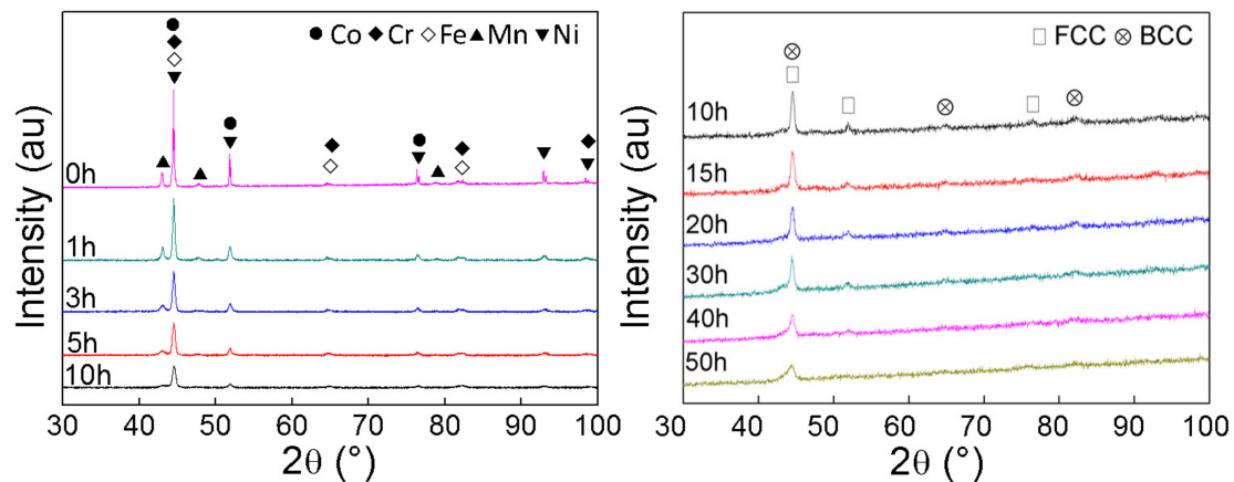
Figure 1. XRD patterns of CrMnFeCoNi powders under different milling times.
