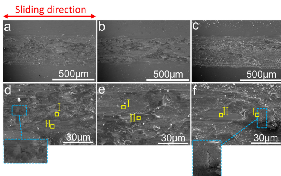
Figure 11. SEM morphologies of the worn surface of the HEA composites (a), 0-YOHEA (d), 0.25-YOHEA (b,e) and 0.5-YOHEA (c,f).
