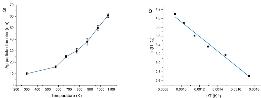
Figure 6. Graphical representation of the mean diameter growth of Ag particles in different temperatures (a). The error bars represent the standard error. An Arrhenius type plot based on Equation (6) for determination of activation energy ( Q_A ) for Ag NP growth on the SiO 2 matrix (b).
