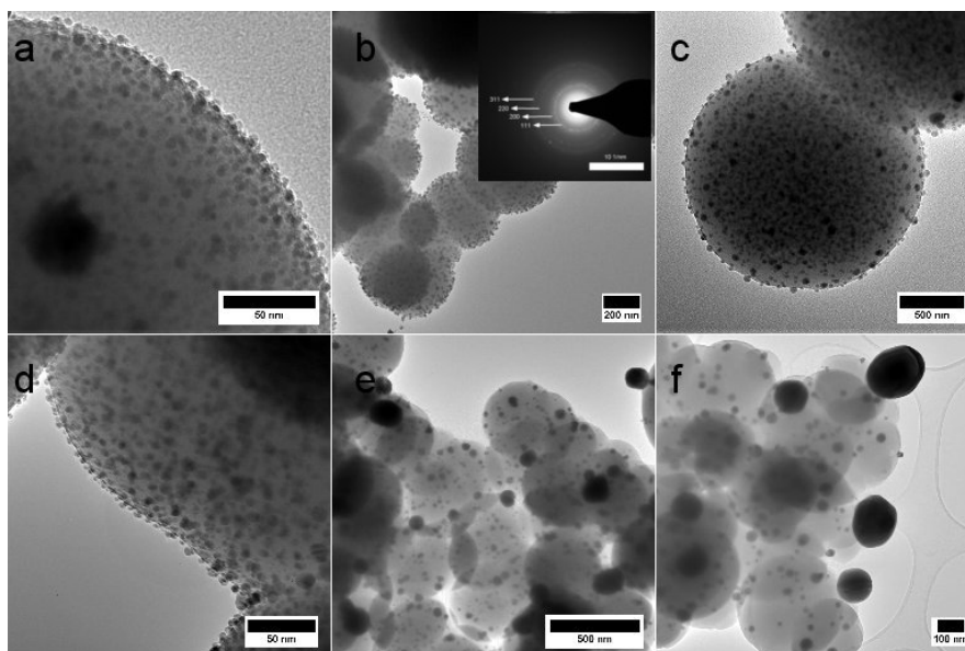
Figure 4. TEM images of (a) the dried SiO 2 -Ag powder and the powders heat treated at (b) 300 °C [12]; (c) 400 °C; (d) 500 °C; (e) 700 °C and (f) 800 °C for 75 min. The lighter parts represent the silica matrix, whereas the darker spots are silver particles. The insert in (b) displays the electron diffraction pattern revealing crystalline silver particles after heat treatment at 300 °C. Scale bars in (a) 50 nm; (b) 200 nm; (c) 500 nm; (d) 50 nm; (e) 500 nm and (f) 100 nm.
