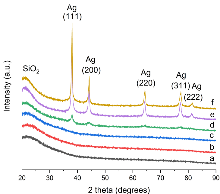
Figure 2. X-ray diffraction patterns of SiO 2 -Ag powders heat treated at (a) 300 °C; (b) 400 °C; (c) 500 °C; (d) 600 °C; (e) 700 °C; and (f) 800 °C for 75 min.
