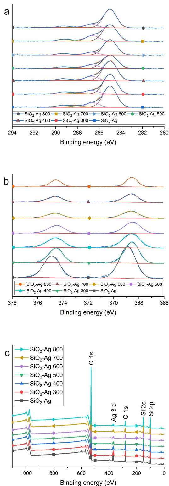
Figure 5. High resolution XPS spectra showing (a) the \text{C } 1s high resolution spectra and (b) the \text{Ag } 3d peaks for the powders. XPS survey spectra of (c) all \text{SiO}_2\text{-Ag} powders.
