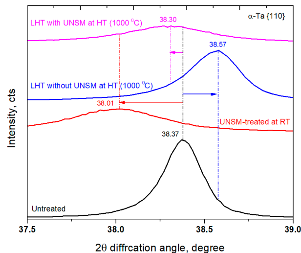
Figure 5. Comparison in intensity peak {110} shift to lower and higher angles of the untreated, UNSM-treated at RT, LHT without and with UNSM treatment specimens.
