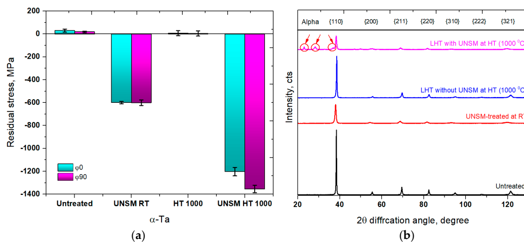
Figure 3. Variation in surface residual stress (a) and X-ray diffraction (XRD) pattern (b) of the untreated, UNSM-treated at RT and LHT without and with UNSM treatment at 1000 °C specimens.
