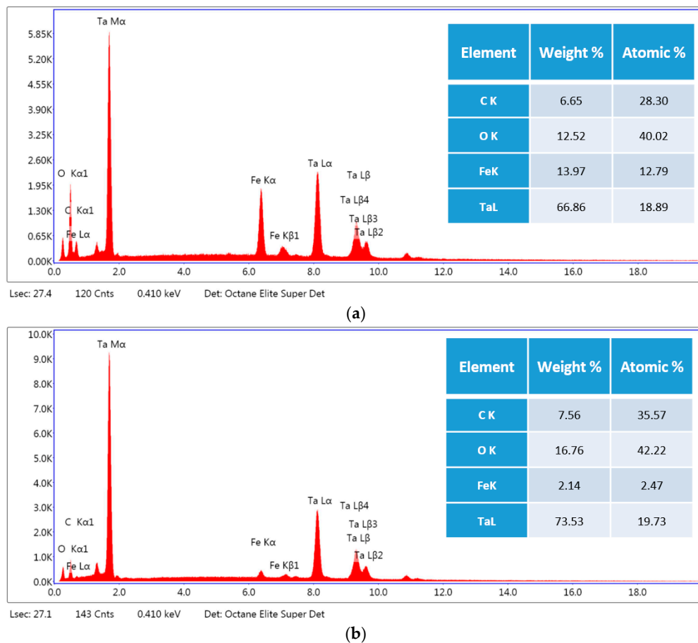
Figure 12. EDX (energy-dispersive X-ray spectroscopy) of the wear track generated on the surface of the UNSM-treated at RT (a) and LHT with UNSM treatment at HT of 1000^\circ\text{C} ; (b) specimens.
