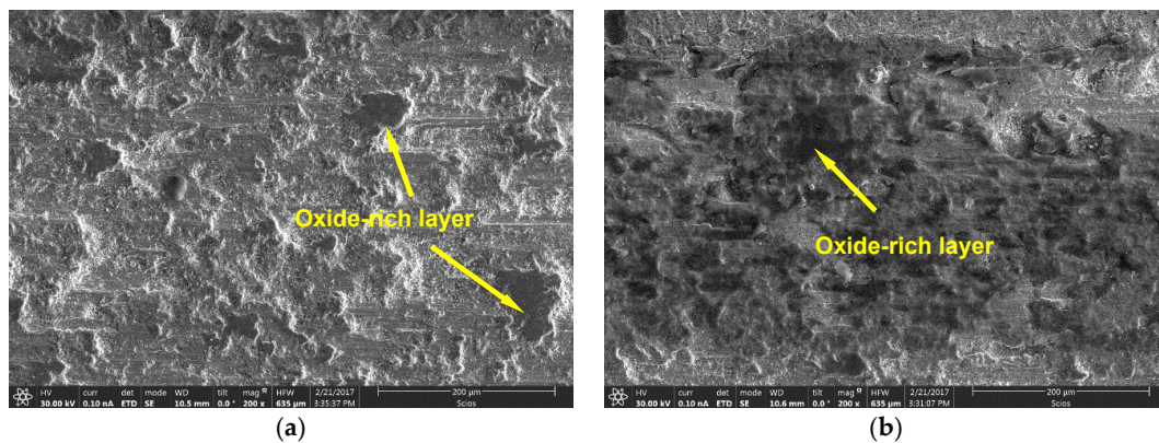
Figure 11. Scanning electron microscopy (SEM) images of the wear track generated on the surface of the UNSM-treated at RT (a) and LHT with UNSM treatment at HT of 1000^\circ\text{C} (b) specimens.
