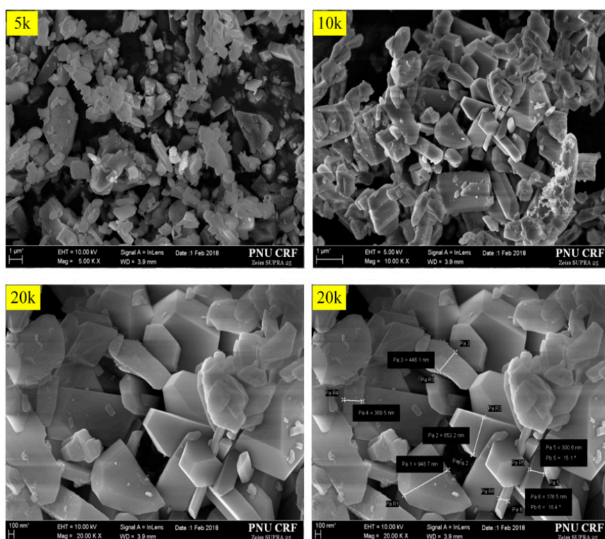
Figure S1. SEM micrographs of synthesized manganese violet pigment at different magnifications: 5 k \times , 10 k \times , and 20 k \times .
