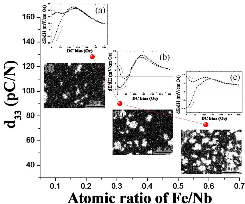
Figure 23. Longitudinal piezoelectric strain coefficient for (1 - x) KNNLS- x NZF composites as a function of atomic ratio of Fe/Nb. ME coefficient for (1 - x) KNNLS- x NZF / Ni / (1 - x) KNNLS- x NZF bending mode laminates: (a) x = 0.1 ; (b) x = 0.2 ; and (c) x = 0.3 . Fe (white color) mapping images for (1 - x) KNNLS- x NZF composites: (d) x = 0.1 ; (e) x = 0.2 ; and (f) x = 0.3 .
