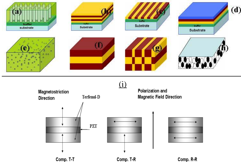
Figure 1. Schematics of the magnetoelectric composites illustrating the multiple possibilities (a) self-assembled nano-pillar structures; (b) layer by layer deposition; (c) deposition accompanied by masking and patterning; (d) three phase deposition for gradient materials; (e) particles dispersed in a polymer matrix; (f) lamination; (g) checkerboard arrangement; (h) sintered particulates; and (i) variation in poling, applied field direction and measuring electrodes.
