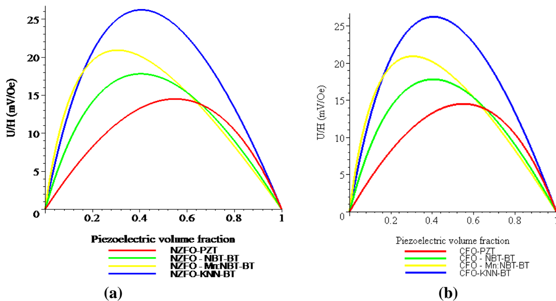
Figure 8. Piezoelectric volume fraction dependence of longitudinal magnetoelectric (ME) voltage coefficient for bilayers of NZFO and piezoelectrics (a) and CFO and piezoelectrics (b).
