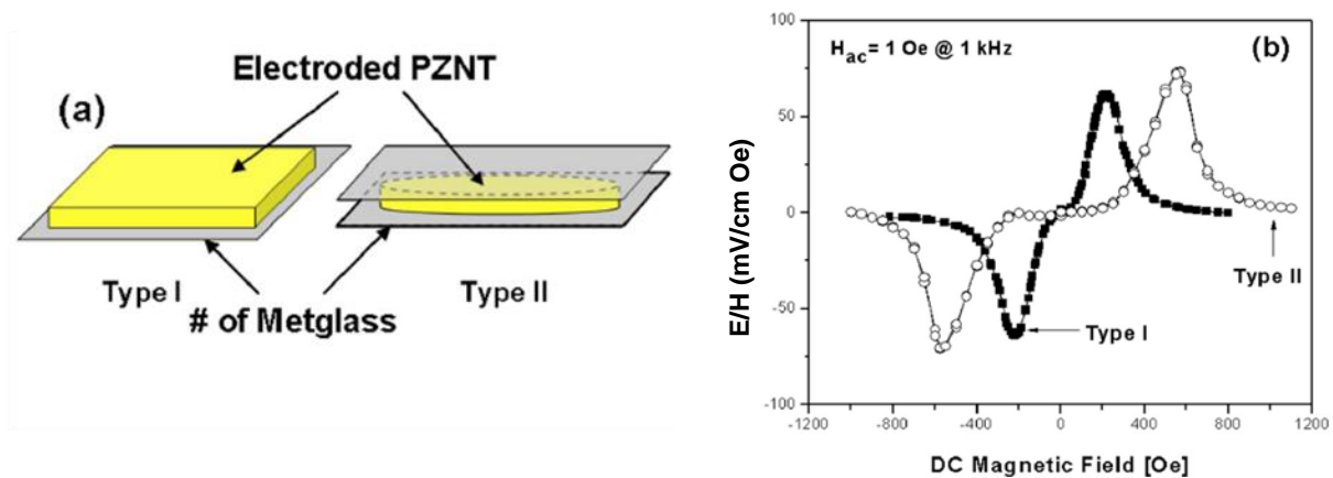
Figure 21. (a) Schematic diagram and (b) ME voltage coefficients for PZNT/Metglas bilayer and Metglas/PZNT/Metglas trilayer laminates.
