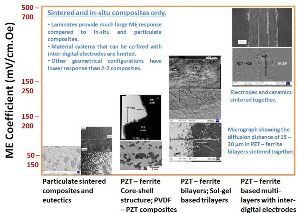
Figure 13. Magnetolectric coefficient for various bulk sintered composites.
