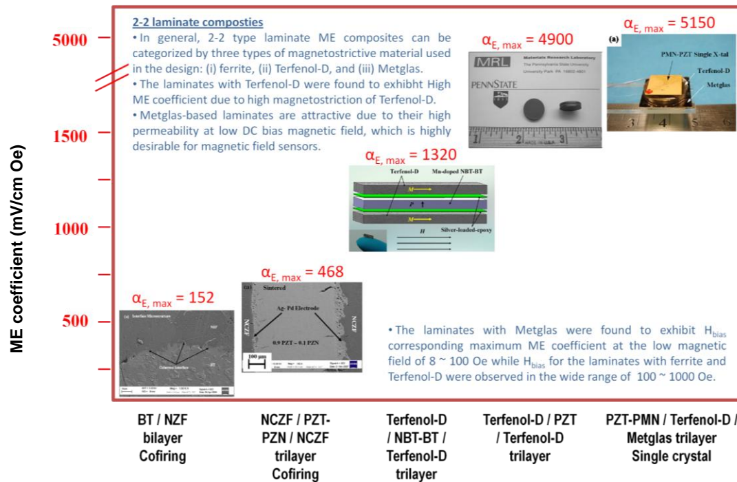
Figure 20. Magnetoelectric coefficient for 2-2 laminate composites in off-resonance conditions.
