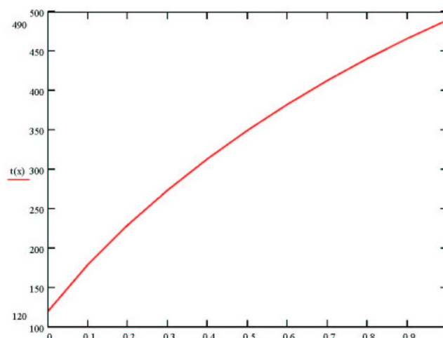
Figure 6. Calculated dependence of the Curie temperature of the system \text{Ba}_{1-x}\text{Pb}_x\text{TiO}_3 .
