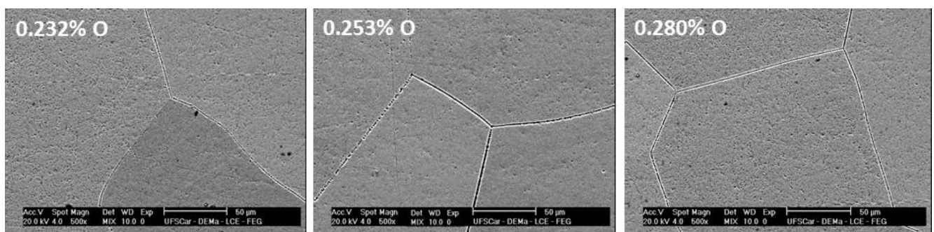
Figure 3. SEM microstructures for the TNZT alloy with 0.232%, 0.253% and 0.280% of oxygen.
