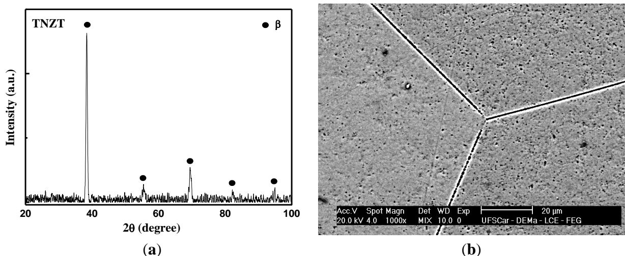
Figure 1. (a) XRD patterns; and (b) SEM microstructures of the TNZT alloy after homogenization heat treatment for 6 h at 1273 K, followed by furnace cooling.
