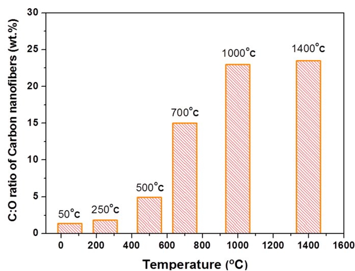
Figure S2. Influence of carbonization temperature on the elemental composition of carbonized starch.
