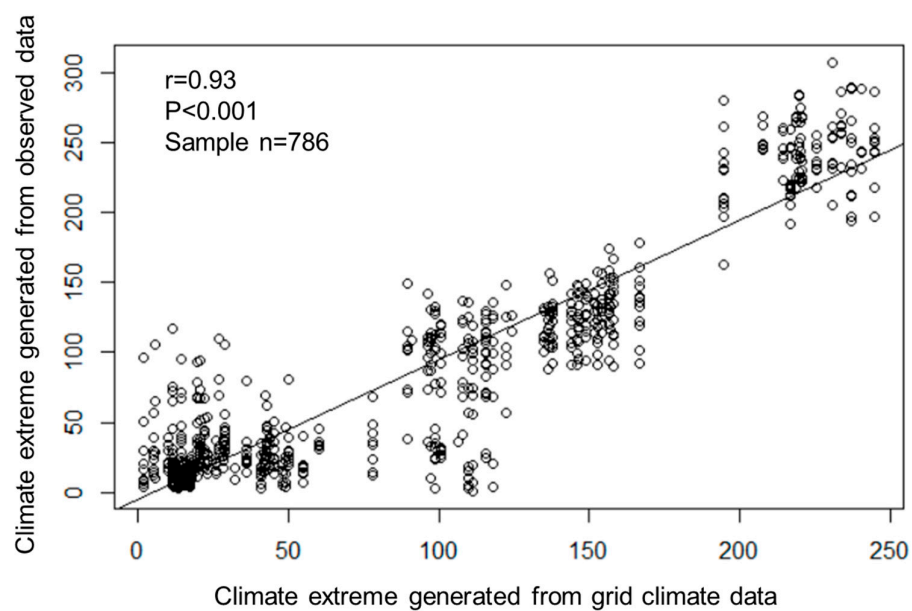
Figure S1. Validation of grid climate data. Pearson coefficient and p value were confirmed by comparing observed meteorological data and grid data that used in this study.
