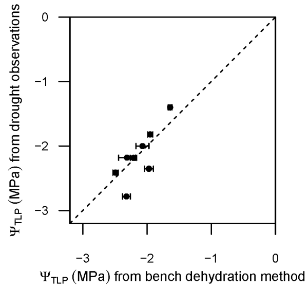
Figure S2. Turgor loss point ( \Psi_{TLP} \pm 1SE ) of eight Eucalyptus species, calculated from standard pressure-volume curves (bench dehydration method) and \Psi_{TLP} calculated from progressive observations of leaf water potential ( \Psi_{leaf} ) and live fuel moisture content (LFMC) of plants subject to imposed drought. Mean absolute error is 0.19 MPa.
