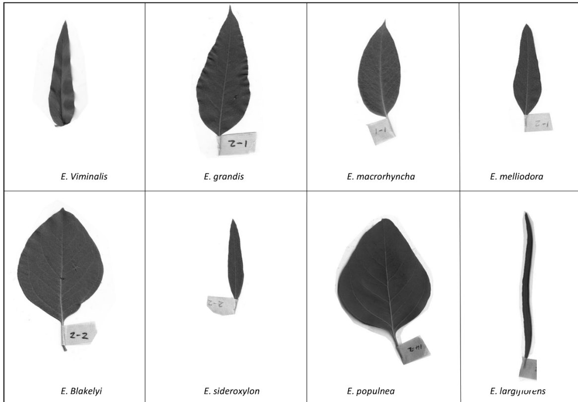
Figure S1. Scanned images of the leaves of each species used in the common garden study. Not to scale.
