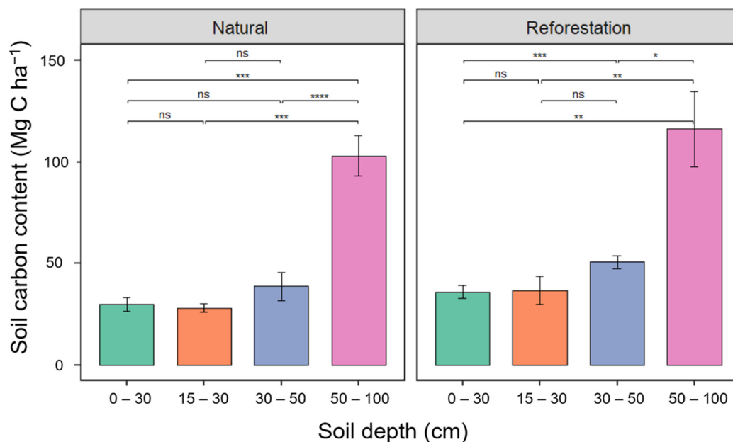
Figure 9. Average soil carbon content at varying soil depths from 0 to 100 cm at the natural and reforestation sites. Significant differences were denoted by * which indicates significance level at p < 0.01 – 0.05 , ** at p < 0.01 – 0.001 , *** at p < 0.001 – 0.0001 , and **** at p < 0.0001 while ns means no significant difference.
