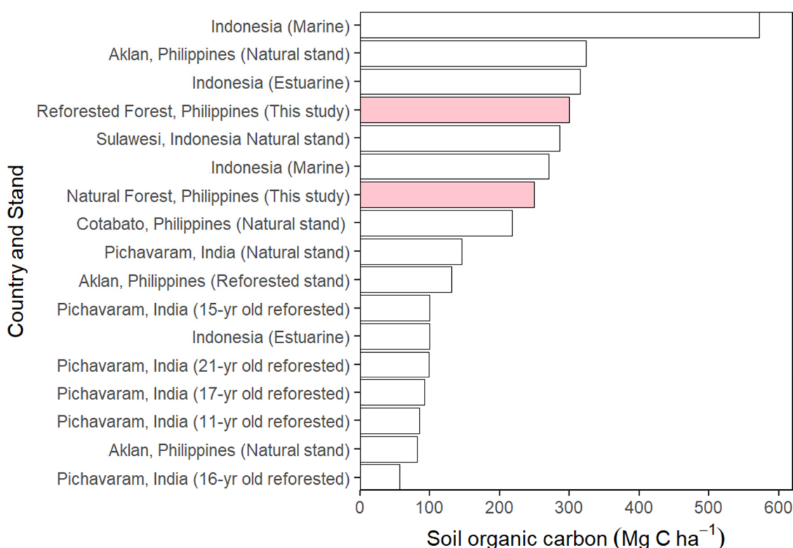
Figure 11. Comparison of studies on mangrove soil organic carbon in the Philippines and other mangrove-rich countries in Asia. These include an estuarine and marine stand in Indonesia [68,69], a reforestation and natural mangrove stands in the Philippines [20,70,71], and reforestation stands in India [72].
