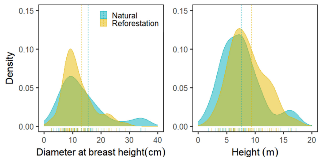
Figure 4. Kernel Density histogram of diameter at breast height (DBH, left panel) and height (right panel) of tree species in the natural and reforestation sites.
