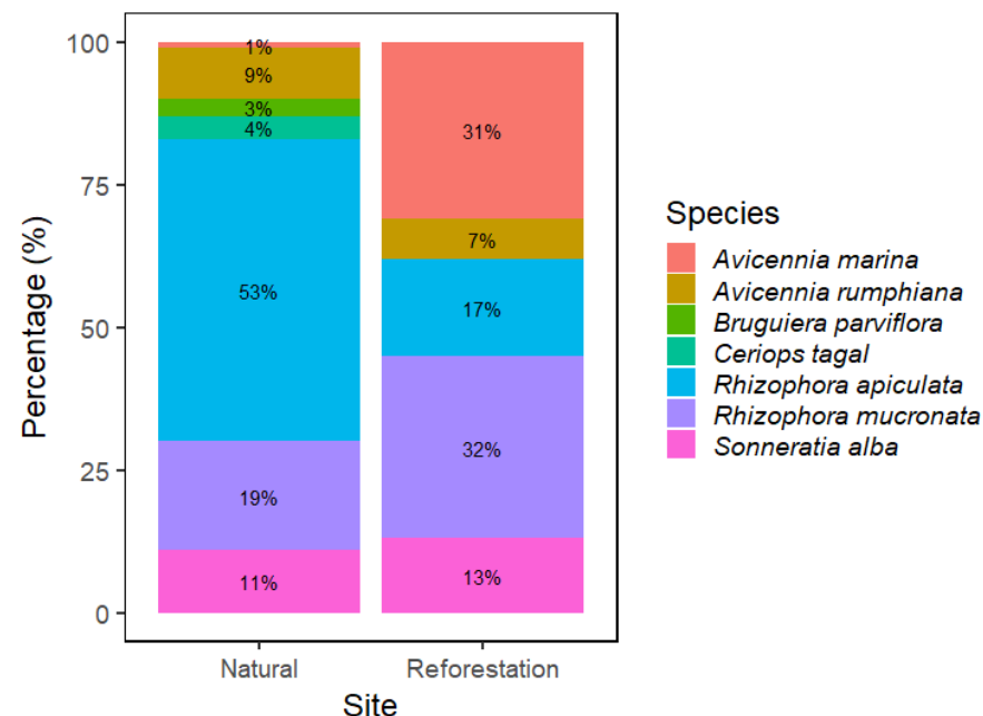
Figure 3. Percentage distribution of species existing in the natural and reforestation sites based on the number of trees recorded during the measurement.
