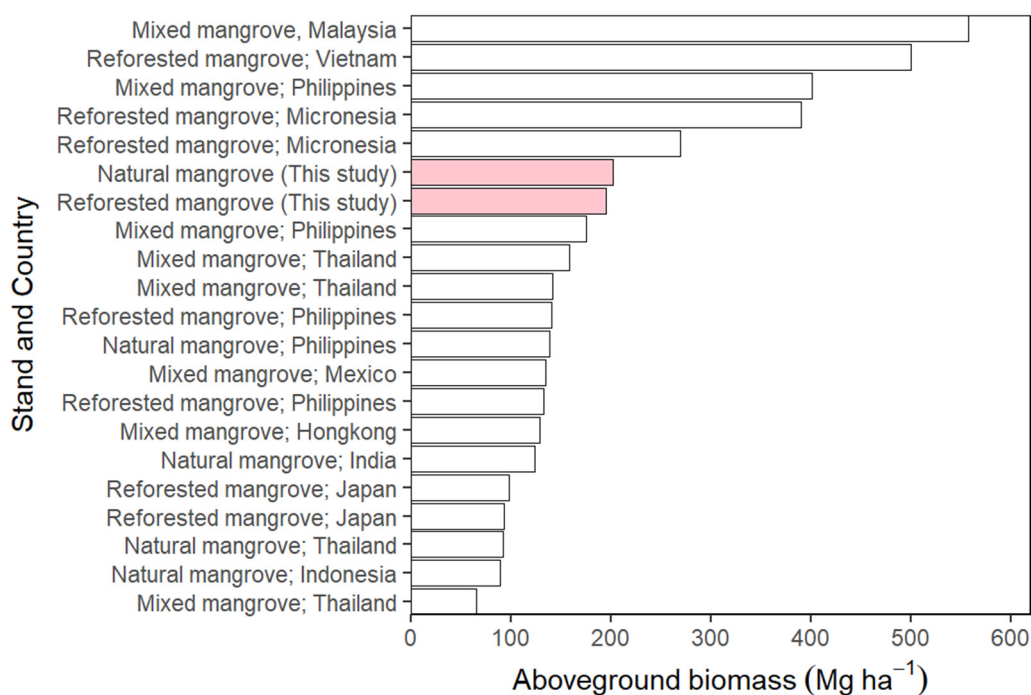
Figure 10. Comparison of studies on mangrove aboveground biomass in the Philippines and other mangrove-rich countries in Asia. These forests include mixed mangrove forests [30,56–60], reforested mangrove forests [8,56,61–63], and natural mangrove forests [8,64,65].
