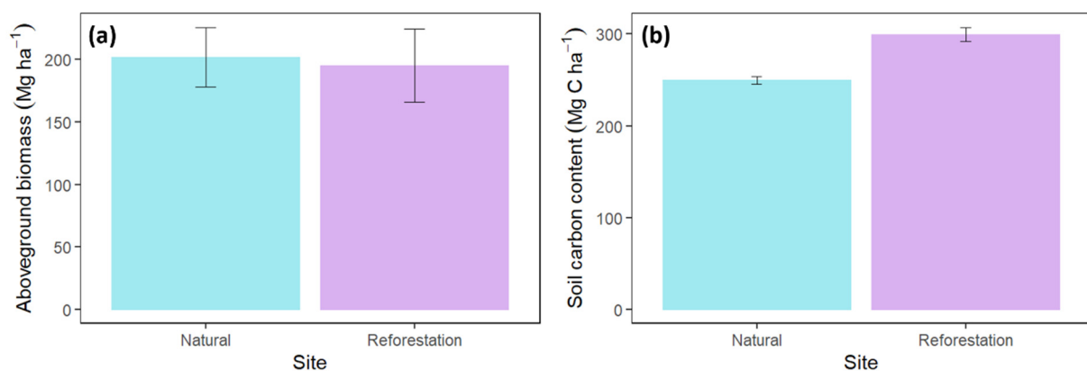
Figure 6. The total aboveground biomass (panel a) and soil carbon content (panel b) in the natural mangrove stand and reforestation mangrove site in Zamboanga del Sur, Philippines.
