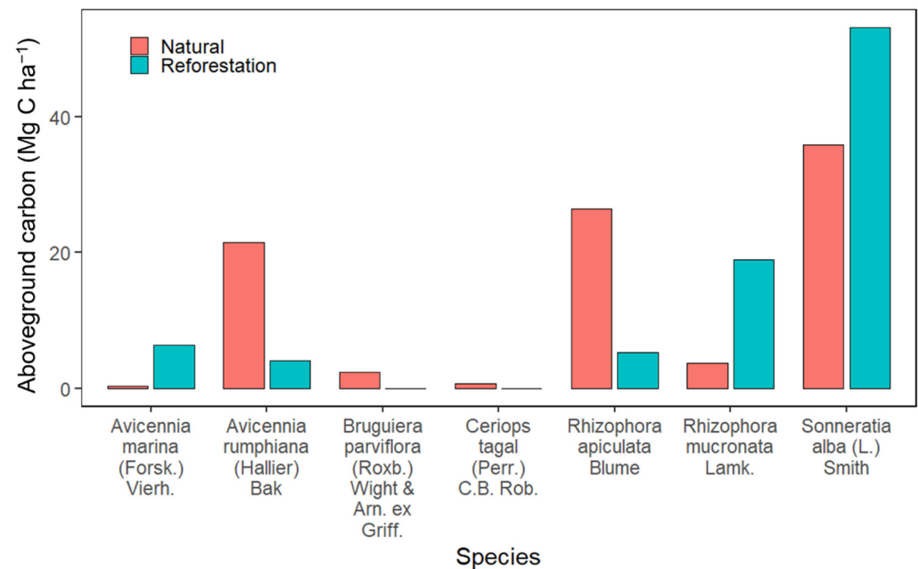
Figure 7. The total aboveground biomass per species in the natural mangrove forest and the reforestation site.
