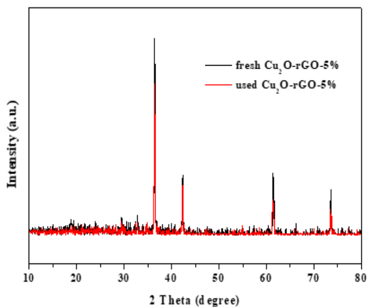
Figure S1. XRD patterns of the fresh and used photocatalysts after 20 h of photocatalytic reaction.
