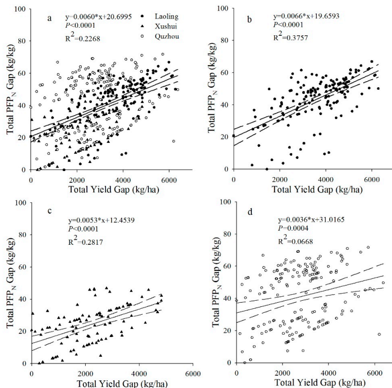
Figure 4. Relationship between the total yield gap and total PFP N gap of summer maize for all three sites (a) and in Laoling (b), Xushui (c), and Quzhou (d). The lines represent trend lines.
