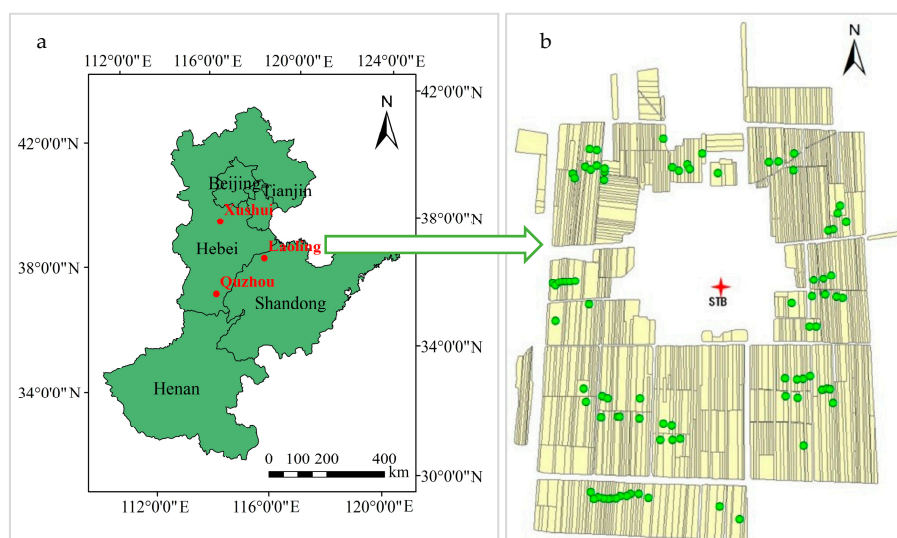
Figure 1. (a) Location of the study sites in the North China Plain (NCP)—red circles; (b) an example of the distribution of monitored fields in one village of Laoling county; the red star is the location of the Laoling Science and Technology Backyard (STB). Residential areas are not shown.
