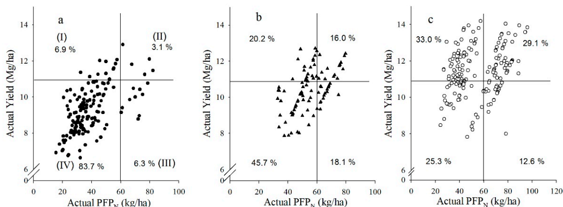
Figure 5. Distribution of yield and PFP N on farms at Laoling (a), Xushui (b), and Quzhou (c). The horizontal and vertical lines are standards for high yield and high efficiency, respectively. For each site, sector (I) represents a high yield and low efficiency (HL), sector (II) represents high yield and high efficiency (HH), sector (III) represents low yield and high efficiency (LH), and sector (IV) represents low yield and low efficiency (LL).
