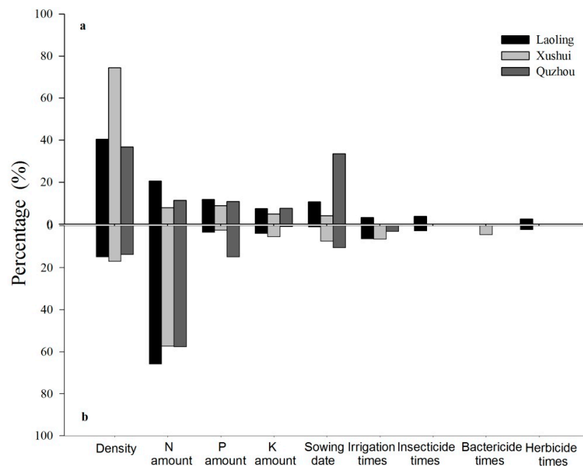
Figure 6. The corresponding proportion of fields in which management factors were the most important factors limiting the yield (a) and PPF_N (b) for the Laoling, Xushui, and Quzhou sites of the NCP in 2015–2016.
