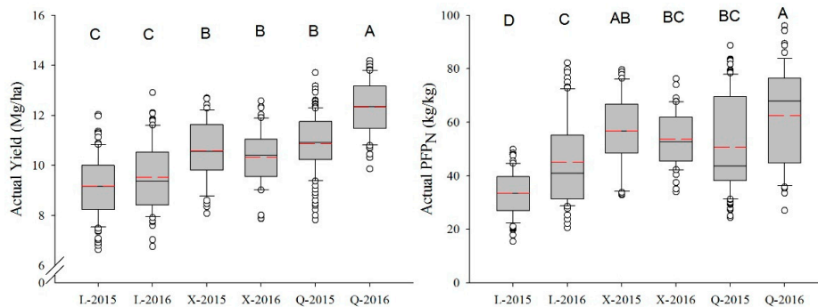
Figure 3. Box plots of the actual summer maize yields (left) and nitrogen use efficiencies (PFP N , grain yield per unit N fertilizer, right) obtained by farmers during 2015–2016 at the three sites. For each site, the three black horizontal lines in the boxes indicate the 75th percentile (top), median (solid line across boxes), and 25th percentile summer maize yield (bottom); the upper and lower bars outside the boxes show the 90% and 10% summer maize yields. The red dotted lines across the boxes are the mean yields of summer maize. The values followed by different letters in each box indicate significant differences at p \leq 0.01 by the Duncan's test.
