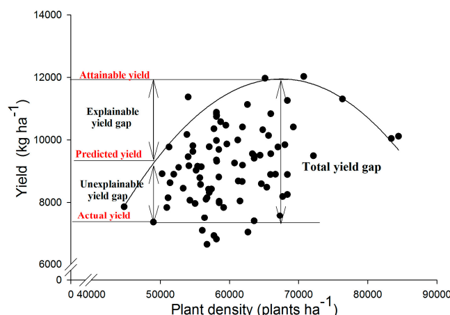
Figure 2. Relationship between summer maize yield and plant density in Laoling in 2015. The curved black line is the boundary line; the values of the upper, middle, and lower horizontal lines are the attainable yield, predicted yield, and actual yield on farms, respectively. The total yield gap is the difference between the attainable yield and the actual yield; the explainable yield gap is the difference between the attainable yield and the predicted yield; and the remainder is the unexplainable yield gap.
