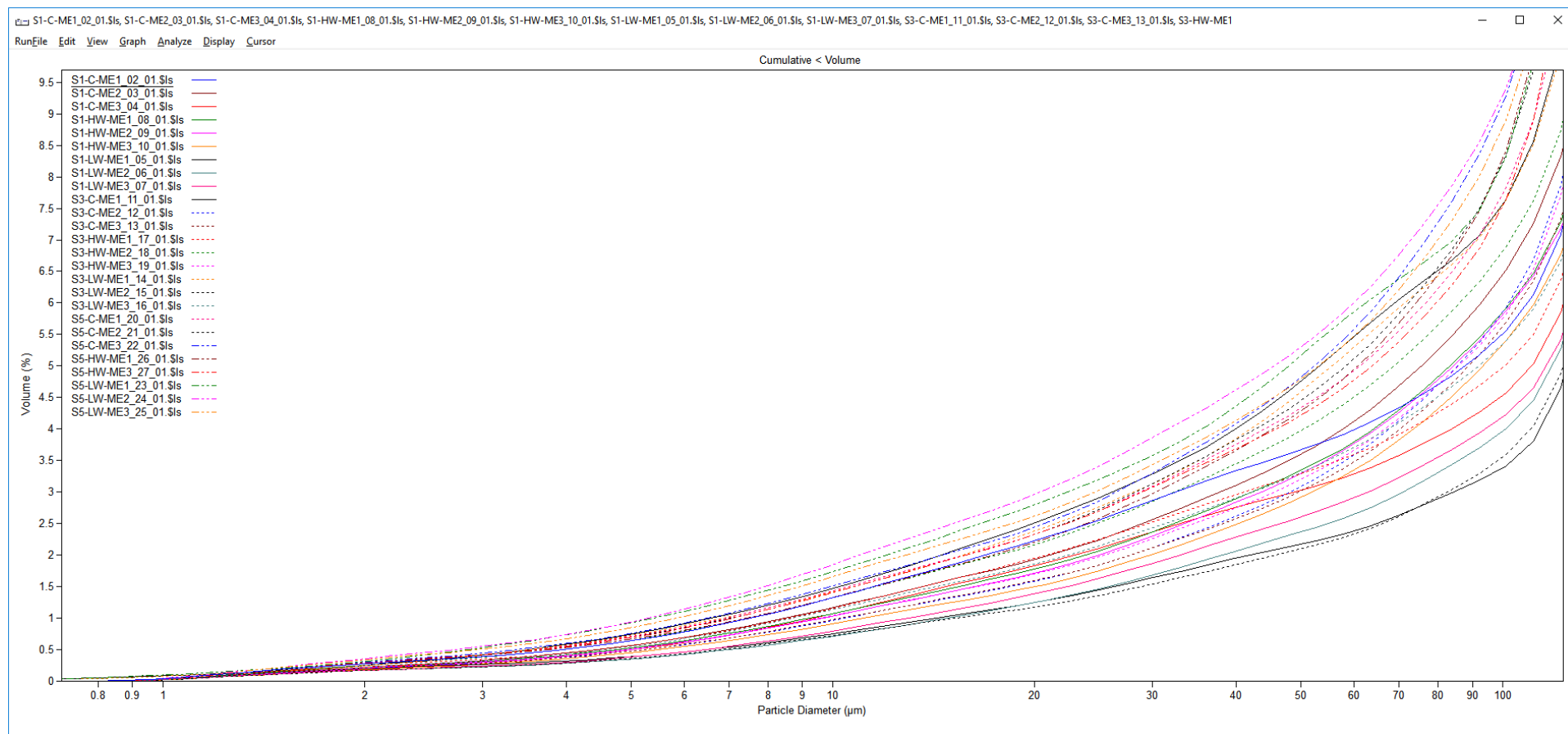
Figure S1. Cumulative Particle Size Distributions. Variation in curve shape occurs after the 40 μm range.
