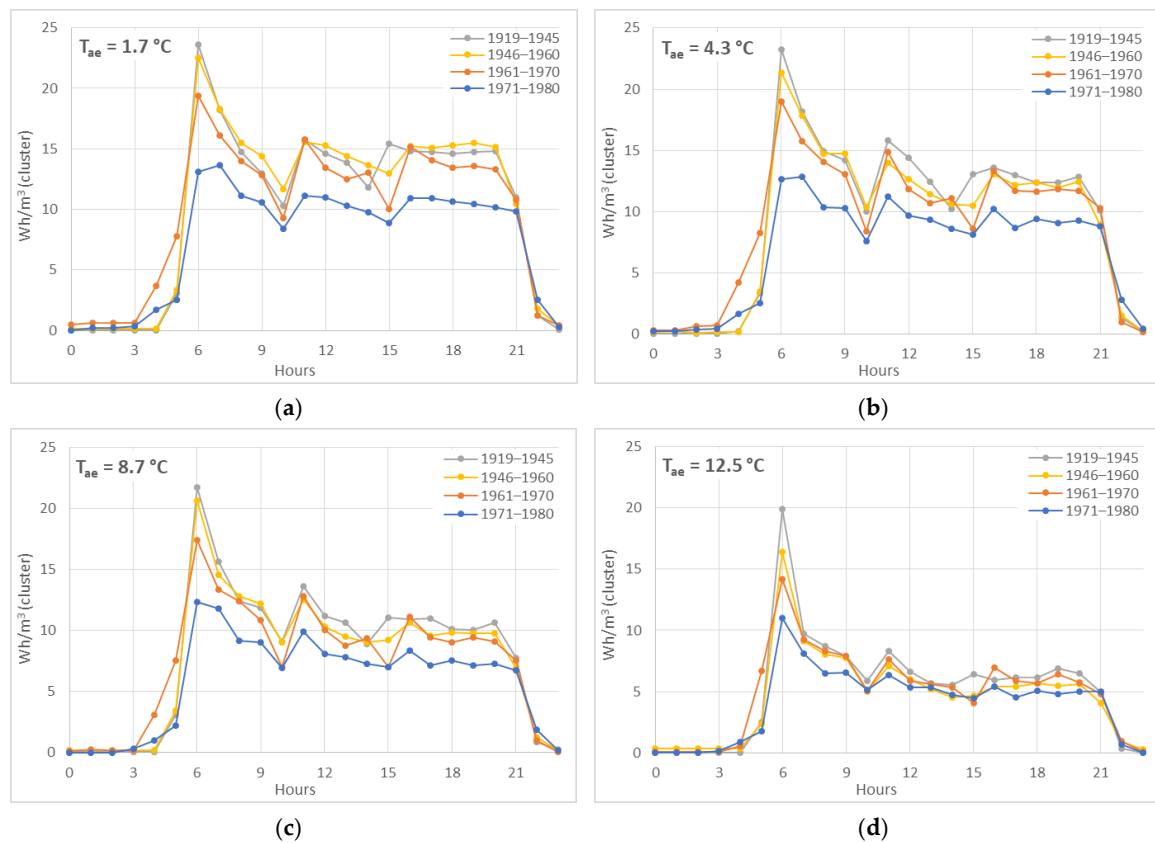
Figure 5. Space heating hourly consumptions (Wh/m 3 ) with different T_{ao} —(a) 1.7 °C, (b) 4.3 °C, (c) 8.7 °C, (d) 12.5 °C—for four clusters of buildings: cluster 1—1919–1945; cluster 2—1946–1960; cluster 3—1961–1970; cluster 4—1971–1980.
