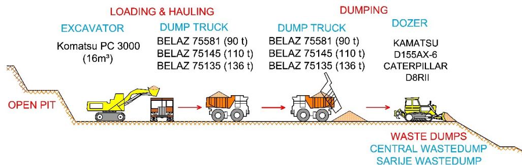
Figure 6. Current waste-mining technology at Ugljevik East 1.
