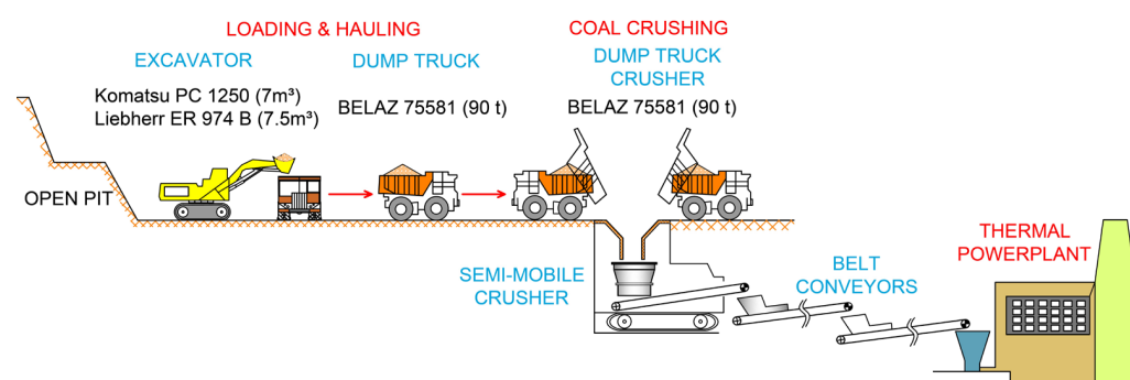
Figure 5. Current coal-mining technology at Ugljevik East 1.
