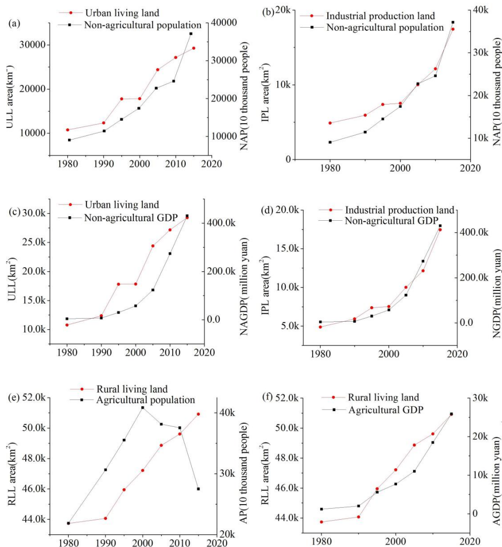
Figure 9. Trend chart among population, GDP and EPL changes: (a) ULL and NAP; (b) IPL and NAP; (c) ULL and NAGDP; (d) IPL and NAGDP; (e) RLL and AP; and (f) RLL and AGDP.
