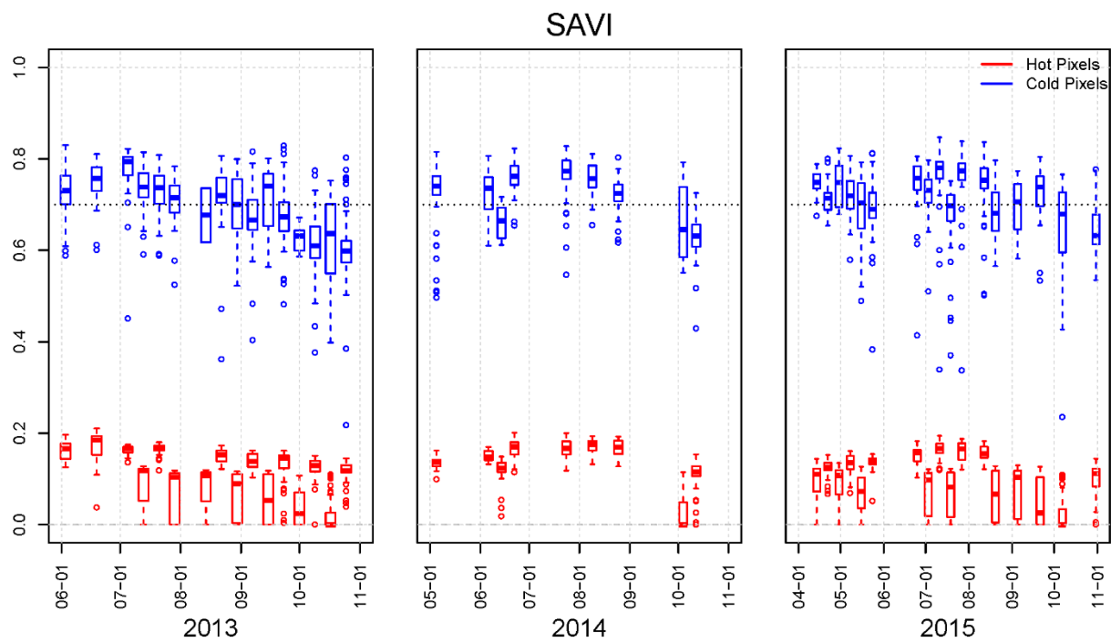
Figure S1: Distribution of SAVI values for hot and cold candidate pixels.
