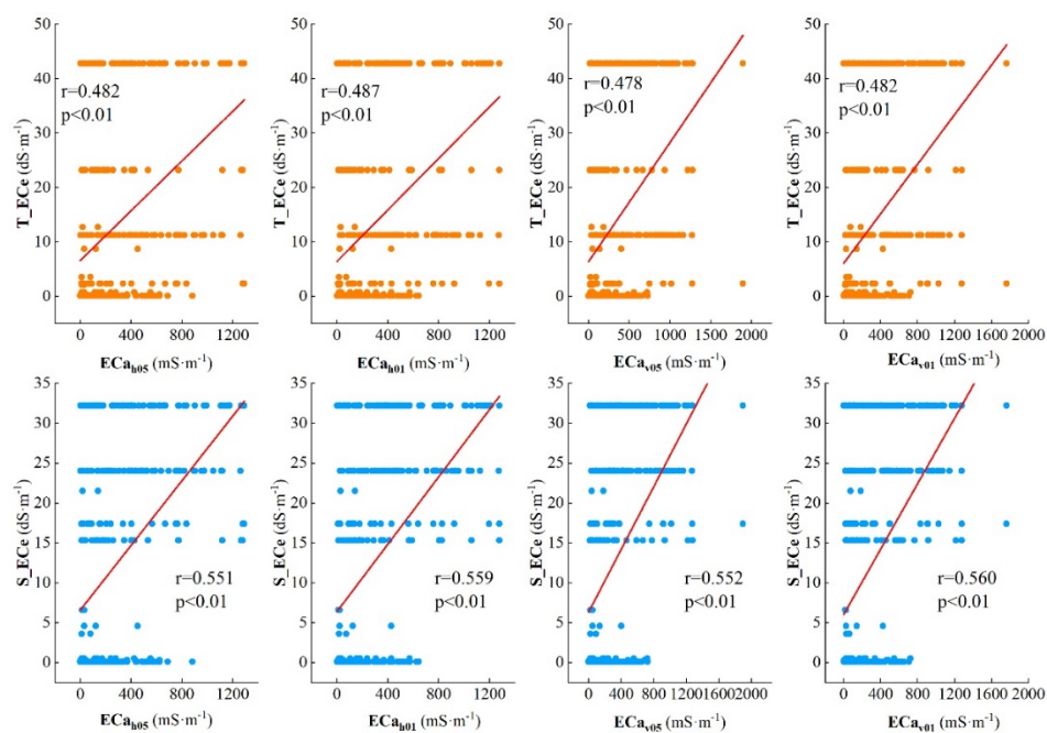
Figures.S1 Scatter plot of observed ECa (four dipole mode) from this study with ECe at depth of 0- 30 cm (T_ECe, dS·m -1 ) and 30-100 cm (S_ECe, dS·m -1 ) from HWSD.
