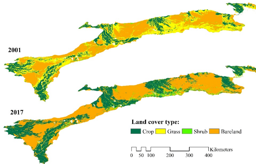
Figures.S2 Land use type of 2001 and 2017 in the study area
