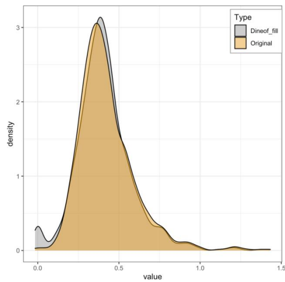
Figure S2 The density distribution of the original (orange) and gap-filled(gray) pixels
