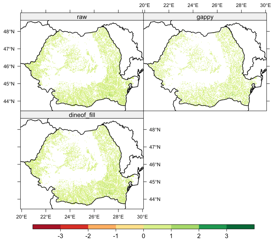
Figure S1 The maps of the original (top-left), artificially gaps (top-right) and dineof filling gaps (bellow left) of 241 -2012 composite
