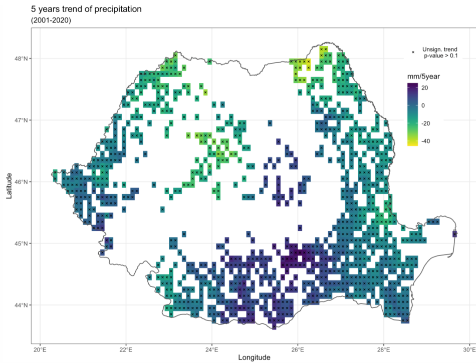
Figure S4 Sen's slope trend for precipitation amount (6 of March- 13 of September) between 2001 and 2020 (no significant values at p < 0.10 )
