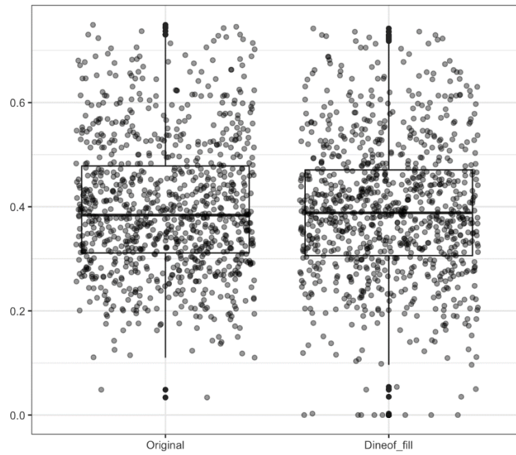
Figure S3 The boxjitterplot of the original (left) and gap-filled (right) pixels
