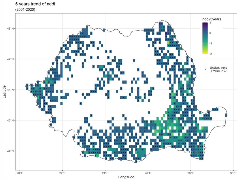
Figure S5 Sen'slope trend for drought frequency (6 of March- 13 of September) derived from NDDI between 2001 and 2020 (sparse significant values, especially in the south-east of Romania)
