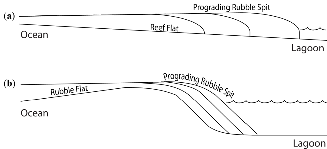
Figure 6. Model demonstrating how the rate of progradation is dependent on the underlying substrate and accommodation space for (a) rubble prograding over a reef flat, and (b) rubble prograding into the lagoon.
