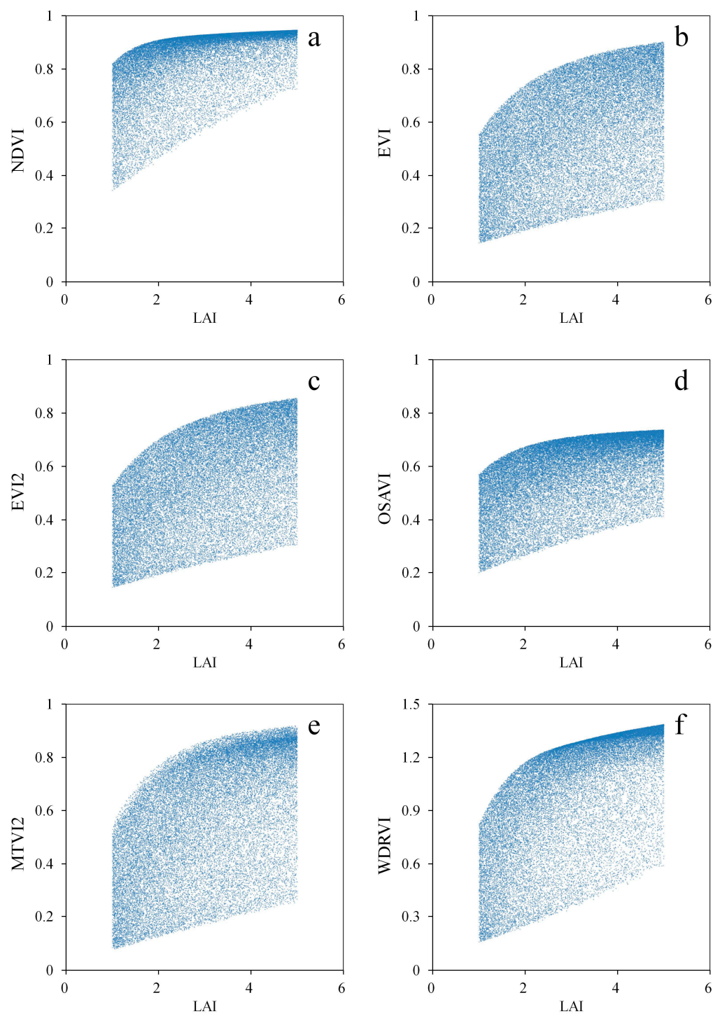
Figure S2. Model simulated relationships between LAI and VIs: (a) NDVI, (b) EVI, (c) EVI2, (d) OSAVI, (e) MTVI2, (f) WDRVI.
