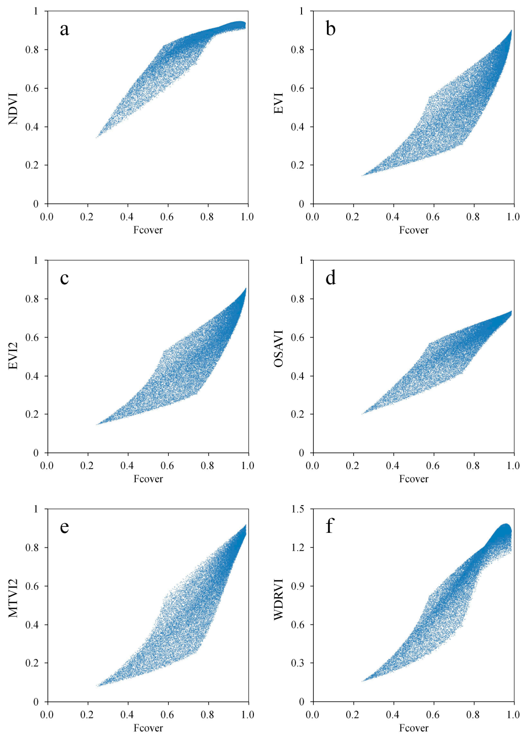
Figure S3. Model simulated relationships between Fcover and VIs: (a) NDVI, (b) EVI, (c) EVI2, (d) OSAVI, (e) MTVI2, (f) WDRVI.
